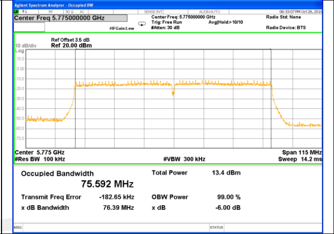
W58_11ac80_-6_Bandwidth_5775M
