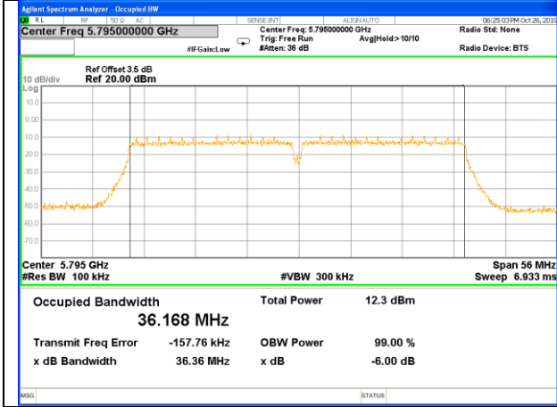
W58_11ac40_Higher_6BW
