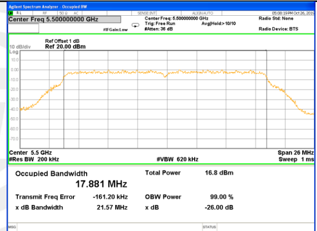
W56_11n20_Higher_26BW and 99%
