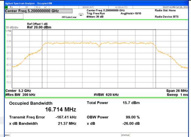
W52_11n20_Lower_26BW and 99%
