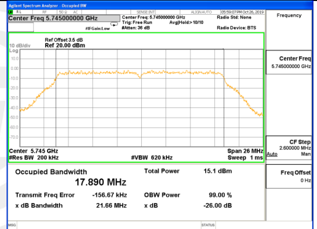
W58_11n20_Higher_26BW and 99%
