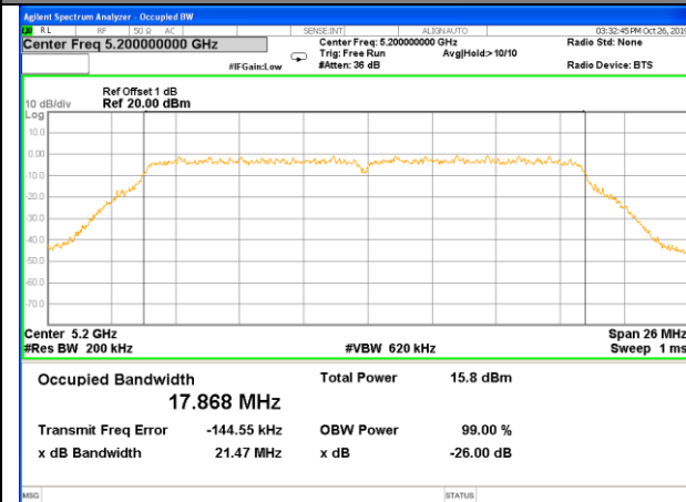
W52_11n20_Middle_26BW and 99%
