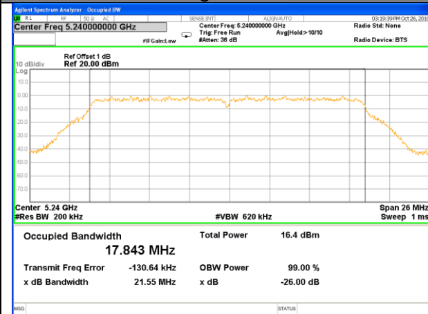
W52_11ac20_Higher_26BW and 99%
