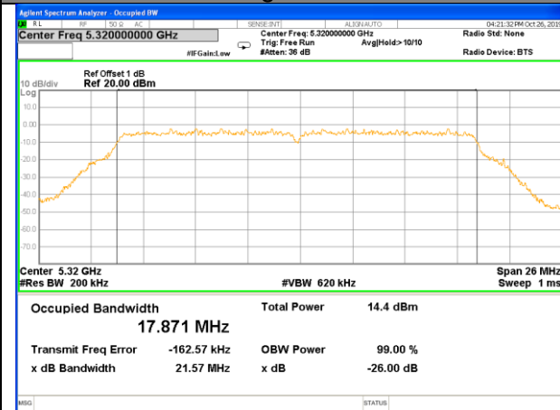
W53_11ac20_Higher_26BW and 99%
