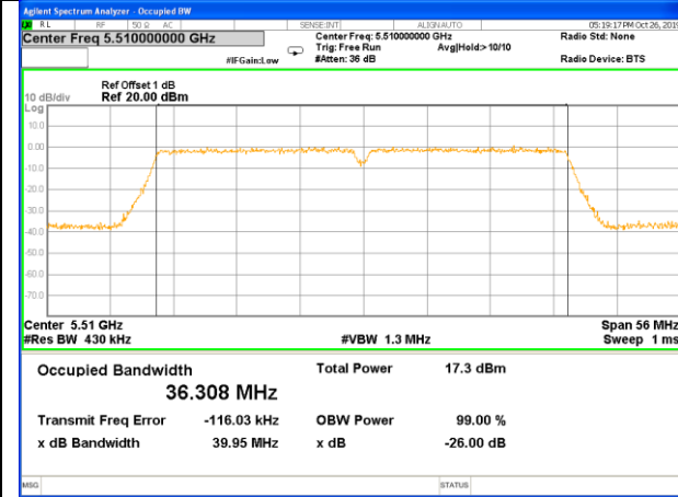
W56_11n40_Higher_26BW and 99%
