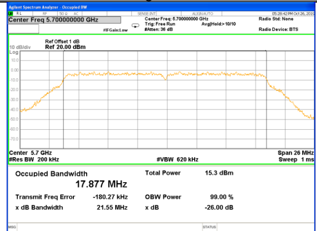
W56_11ac20_Higher_26BW and 99%
