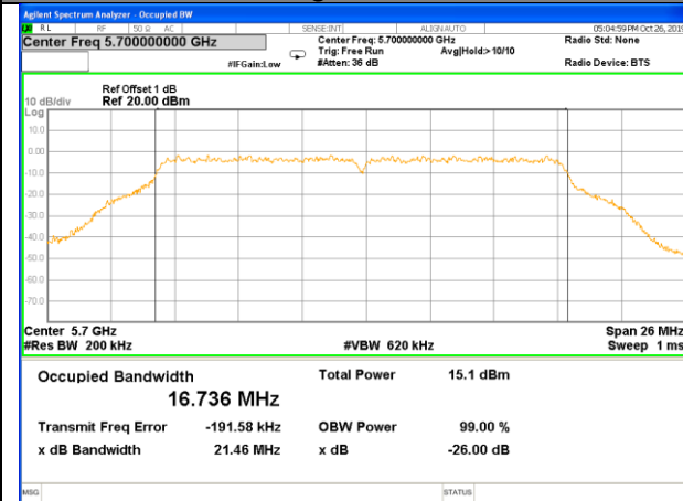
W56_11n20_Middle_26BW and 99%
