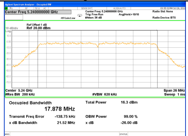
W52_11n20_Higher_26BW and 99%
