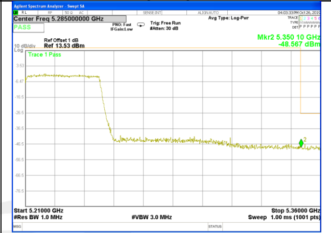
W52_11ac80_CH42(5210MHz)_Band edge_Right
