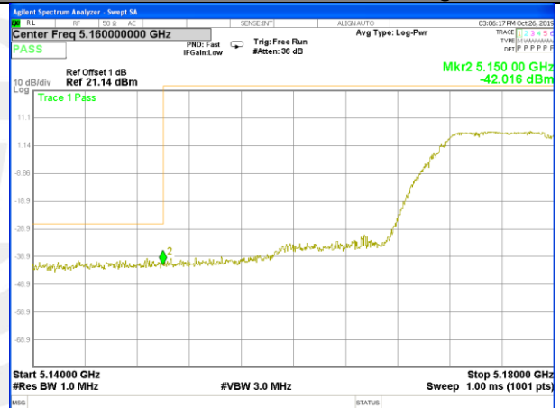
W52_11n20_Lower_Conducted Spurious
