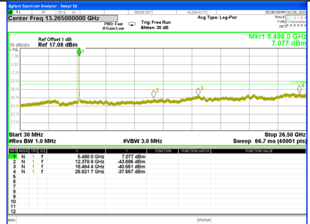
W56_11n20_Lower_Conducted Spurious
