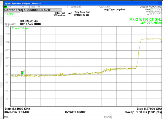
W53_11ac80_CH58(5290MHz)_Conducted Spurious
