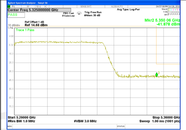
W53_11ac80_CH58(5290MHz)_Band edge_Right
