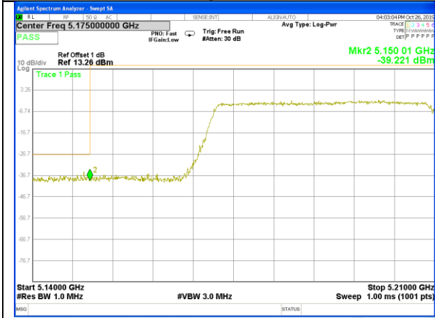
W52_11ac80_CH42(5210MHz)_Band edge_left
