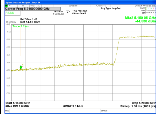
W53_11ac80_CH58(5290MHz)_Band edge_left
