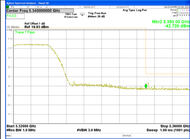
W53_11ac40_Higher_Conducted Spurious
