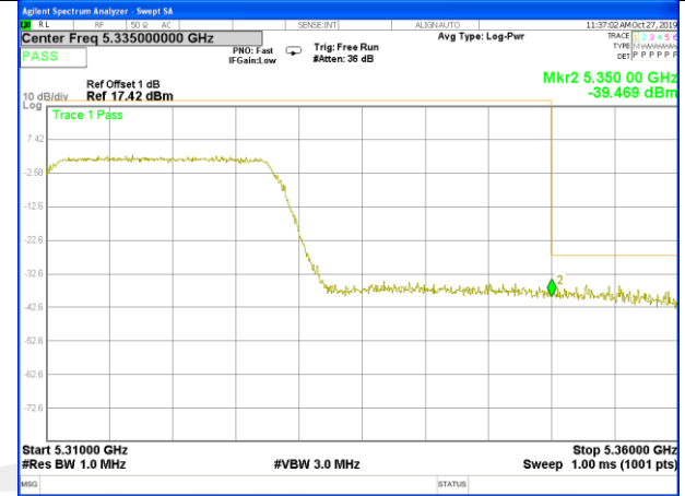
W53_11ac20_Middle_Conducted Spurious
