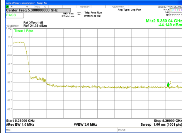
W52_11ac40_Higher_Conducted Spurious
