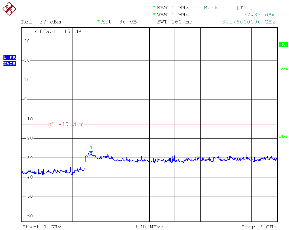
GPRS 850MHz Channel = 190, 1GHz to 9GHz
