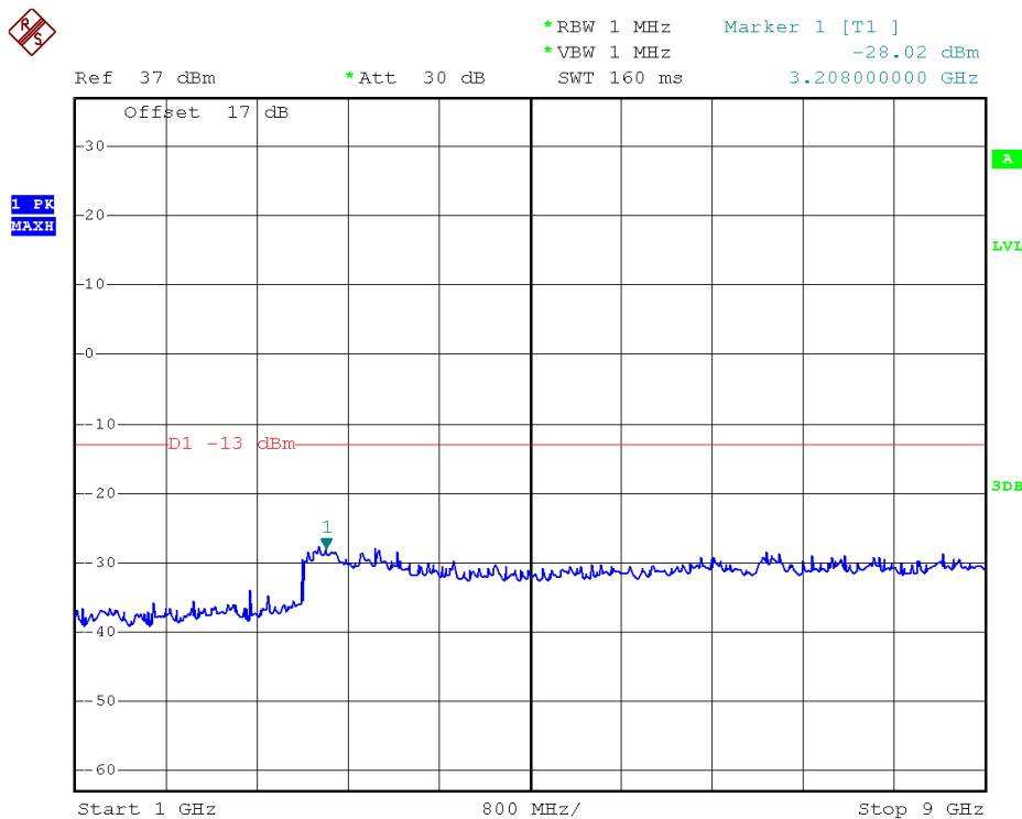
GPRS 850MHz Channel = 251, 1GHz to 9GHz
