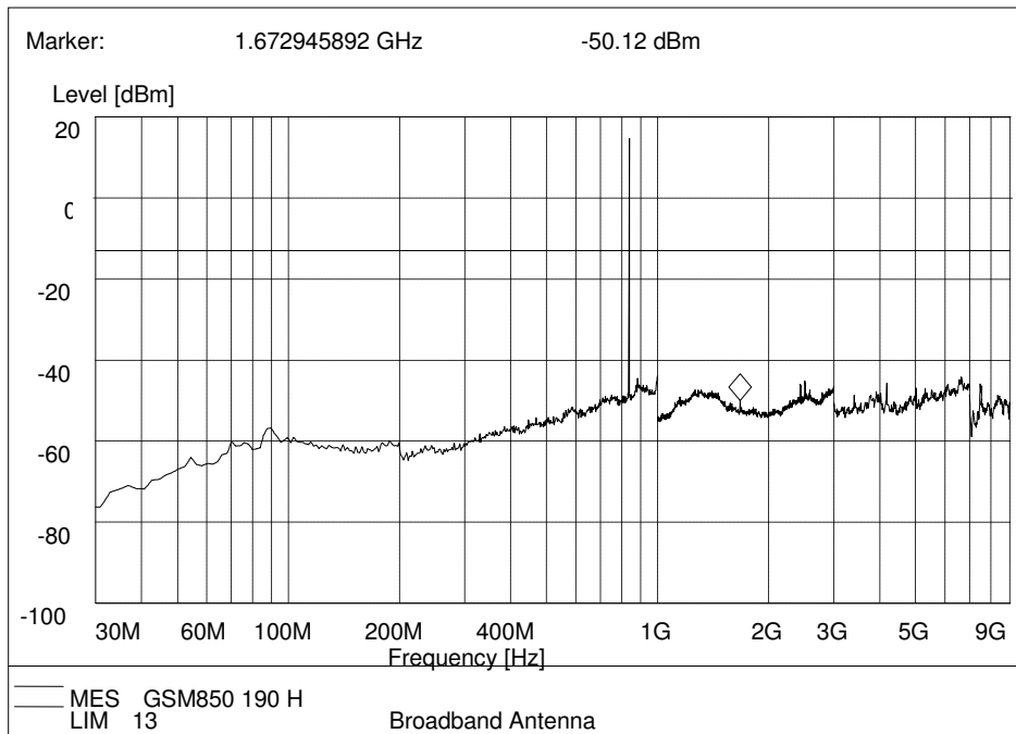
GPRS 850MHz, Test Antenna Horizontal
