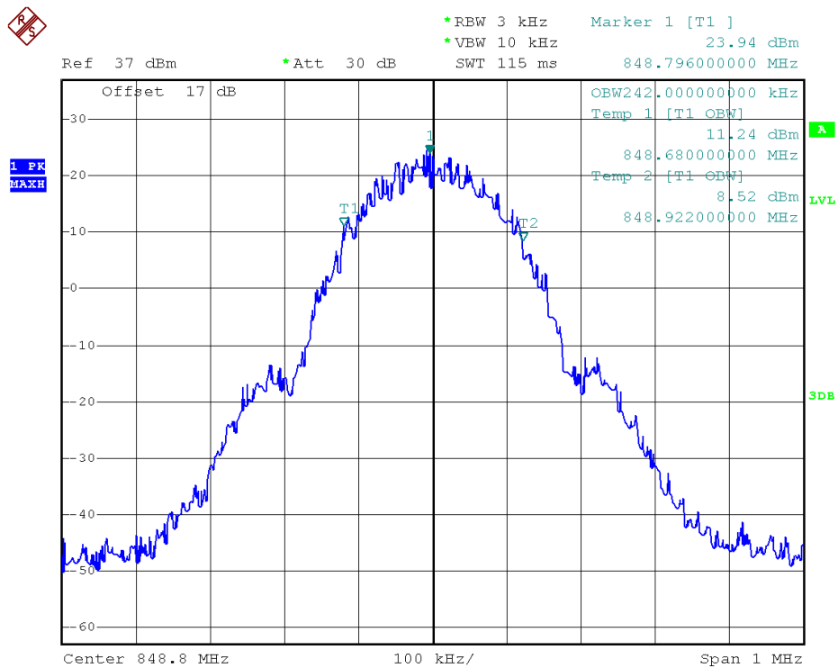
(Plot A6: GPRS 850MHz Channel = 251 99% Occupied Bandwidth)
