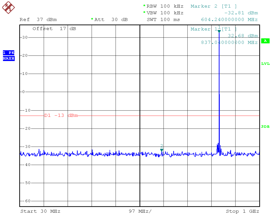
GPRS 850MHz Channel = 190, 30MHz to 1GHz
