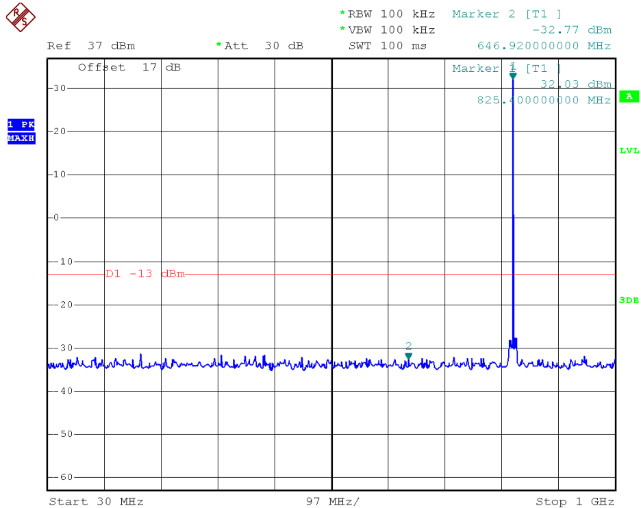
GPRS 850MHz Channel = 128, 30MHz to 1GHz
