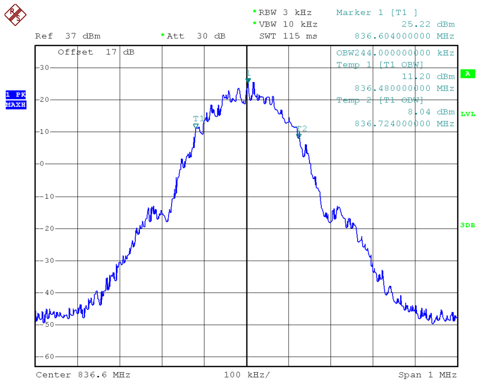
(Plot A4: GPRS 850MHz Channel = 190 99% Occupied Bandwidth)
