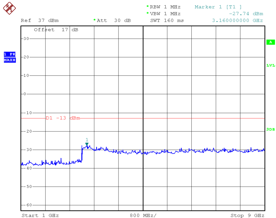
GPRS 850MHz Channel = 128, 1GHz to 9GHz
