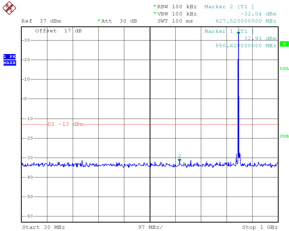
GPRS 850MHz Channel = 251, 30MHz to 1GHz
