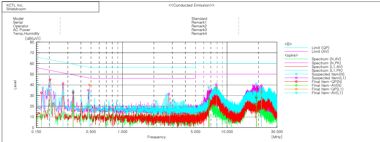
Figure 6. plot of Conducted Emission
