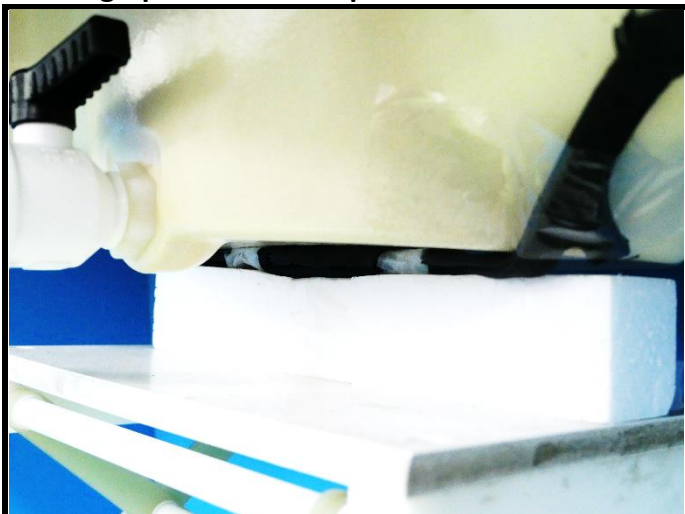
The EUT Surface of Antenna Location tested at 0 mm
