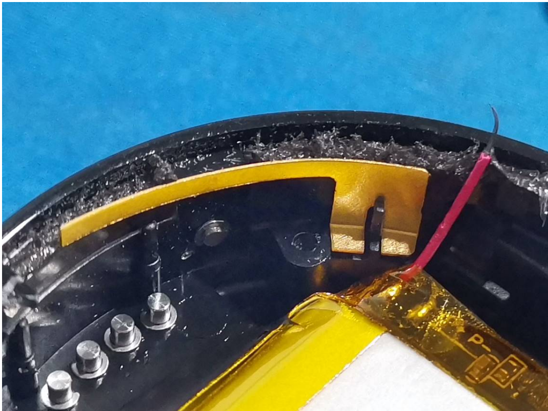
BLE/ANT+ Antenna
