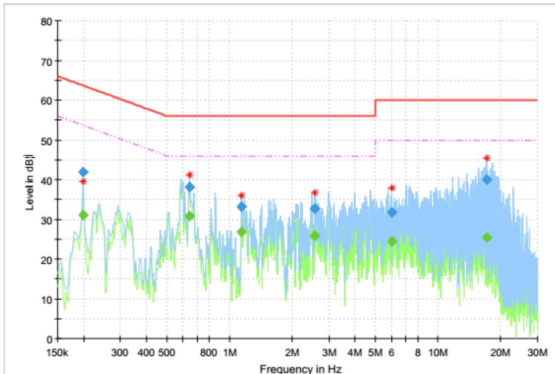
Figure 4 TX mode (150kHz-30MHz)
