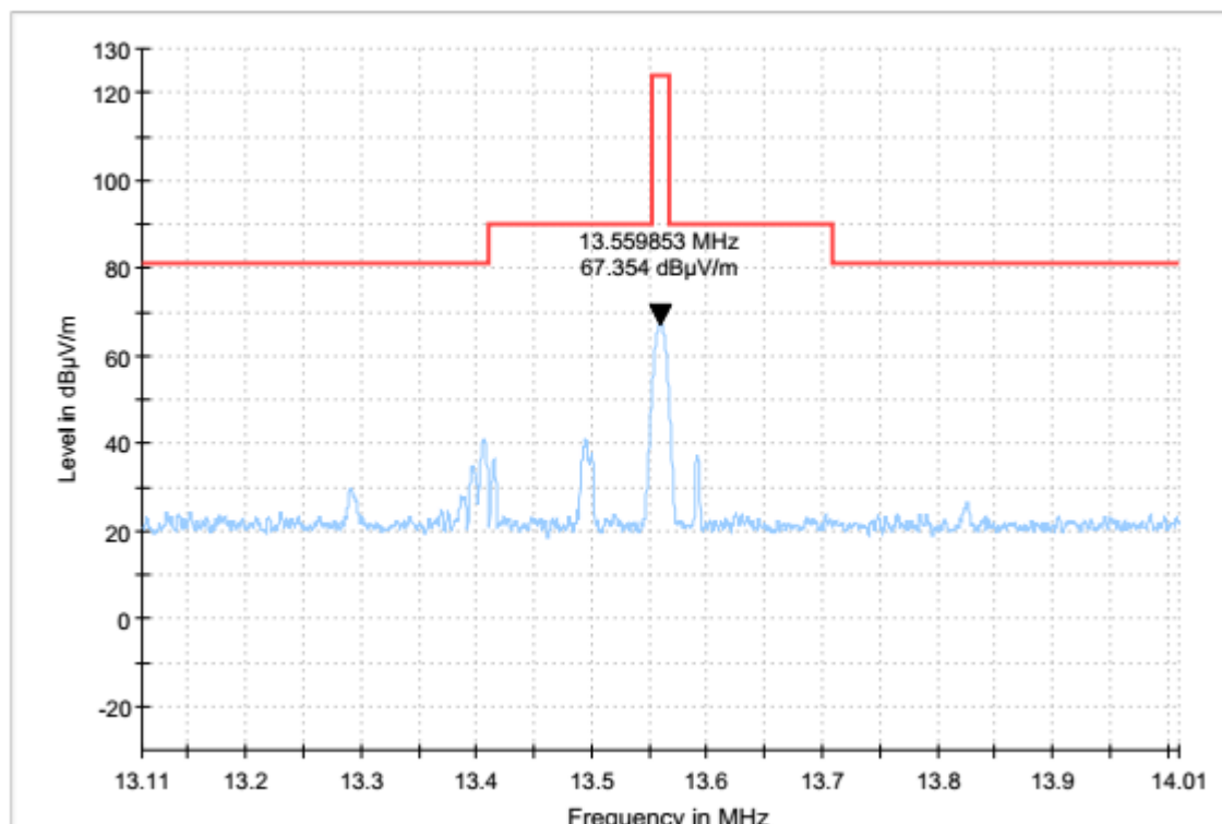
Figure 1 TX mode
