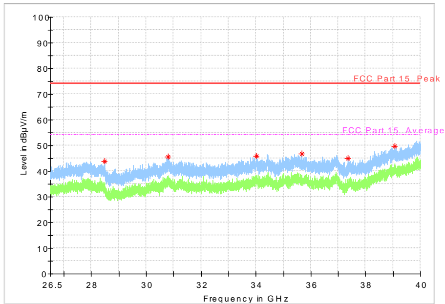
Fig. 67 Radiated emission: 802.11n, (802.11n-HT40, Ch159, 26.5 GHz - 40 GHz)
