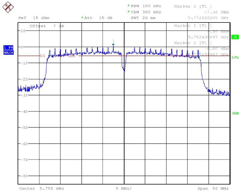
Fig. 7 Occupied 6dB Bandwidth (802.11n-HT40, Ch 151)
