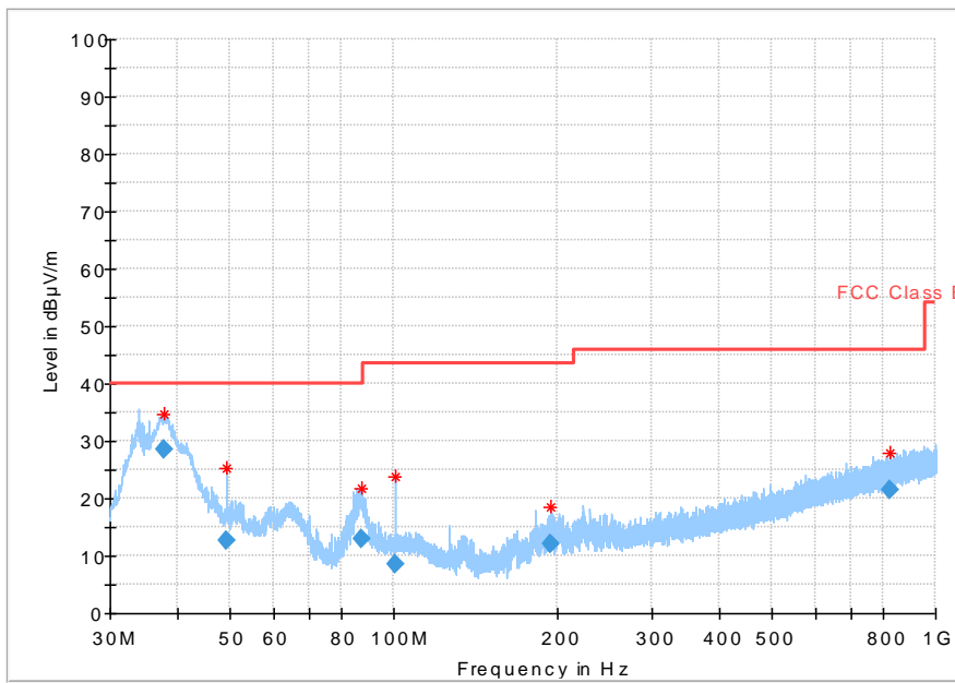
Fig. 48 Radiated Spurious Emission (802.11n-HT20, Ch149, 30 MHz-1 GHz)
