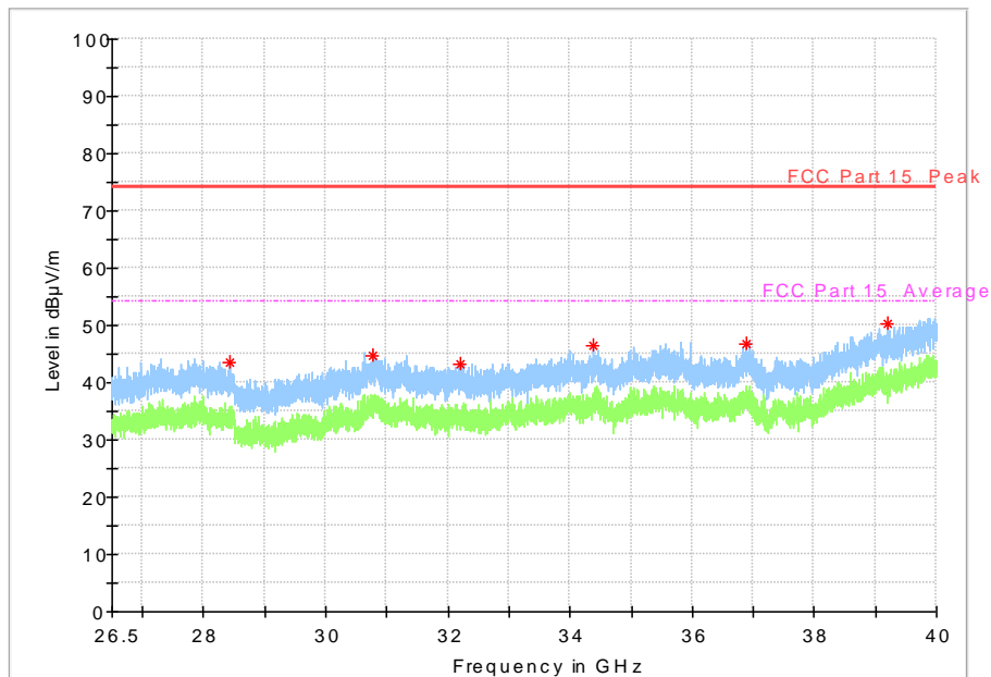
Fig. 42 Radiated emission: 802.11n, (802.11a, Ch157, 26.5 GHz - 40 GHz)
