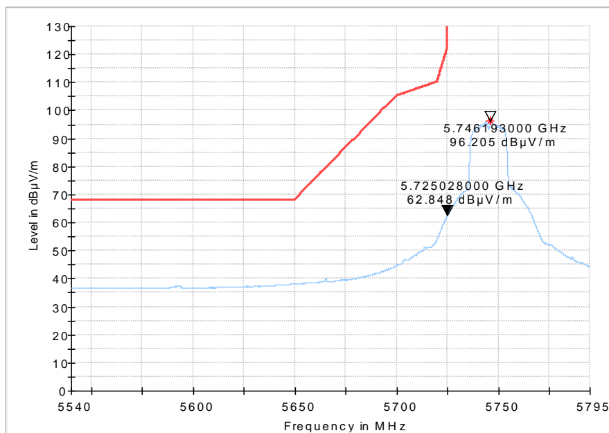
Fig. 75 Band Edges (802.11n-HT20, 5745MHz)
