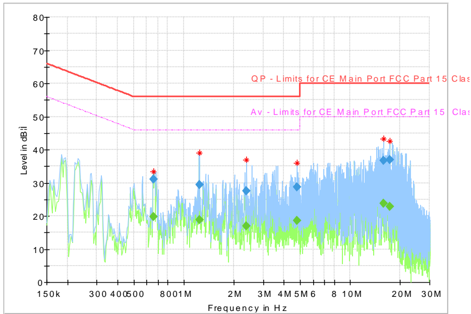
Fig. 79 AC Powerline Conducted Emission-802.11a
