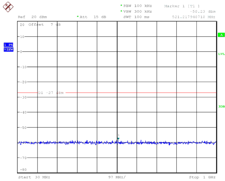
Fig. 30 Conducted Spurious Emission (802.11n-HT40, Ch159, 30 MHz-1 GHz)
