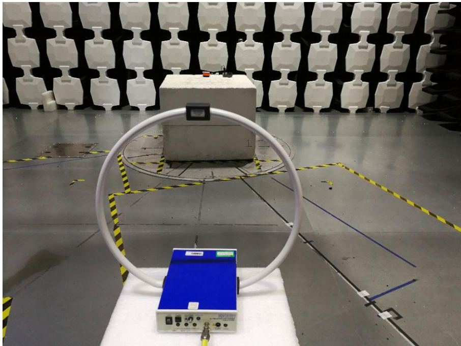
Description: Radiated Emission Test Setup (NFC_ Below 30MHz)
