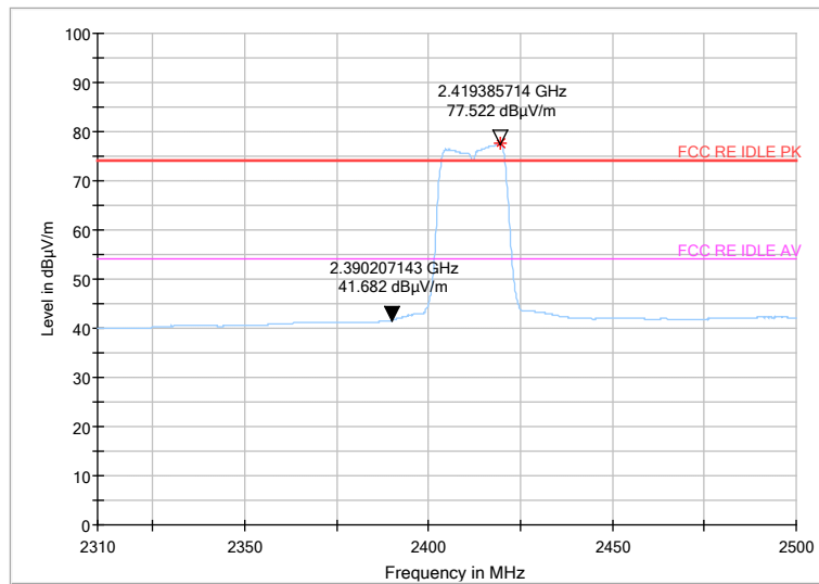
Fig.67 Radiated emission (Power): 802.11n, low channel
