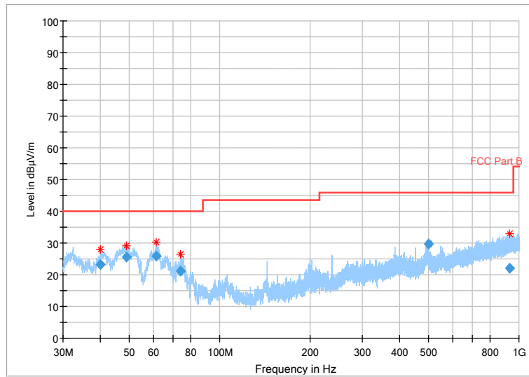
Fig.59 Radiated Spurious Emission (802.11b,Ch1,30MHz~1GHz)
