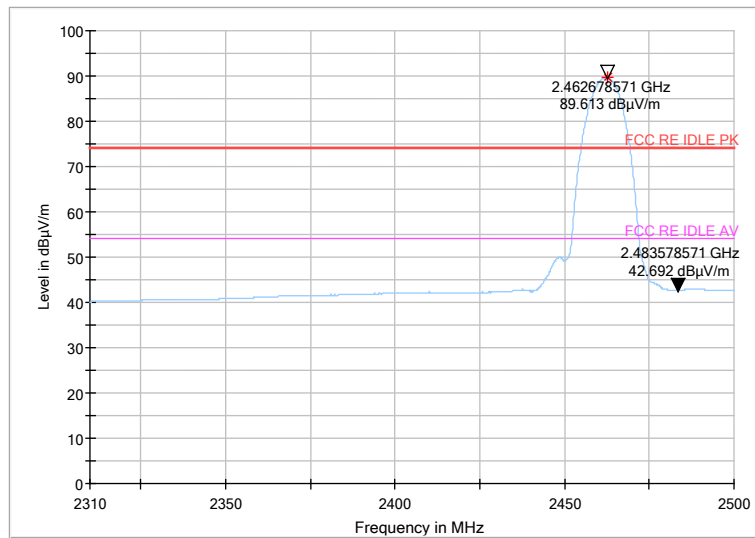
Fig.58 Radiated emission (Power): 802.11b, high channel
