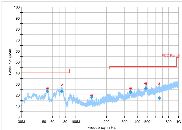
Fig.18 Radiated emission: Ch0, 30MHz~1GHz
