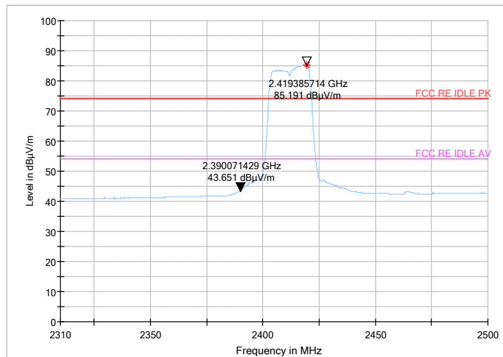
Fig 11. Radiated emission (Power): 802.11n, low channel
