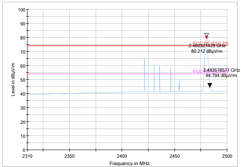
Average Detector
