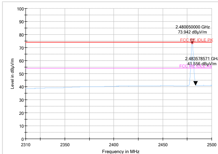
Fig 5 Radiated emission (Power): GFSK, high channel
