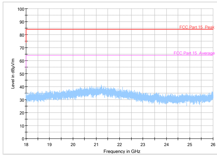
ALL Channel 18GHz~26GHz
