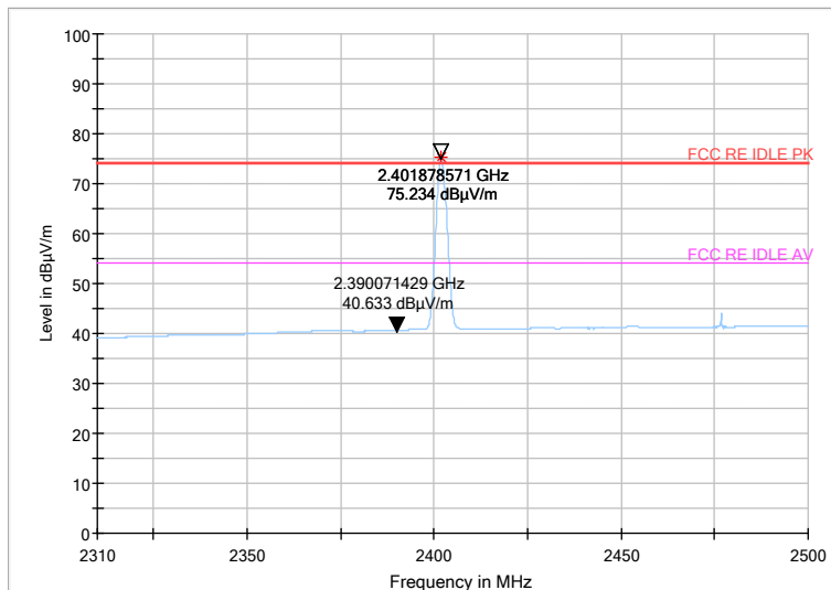
Fig 53 Radiated emission (Power): 8DPSK, low channel
