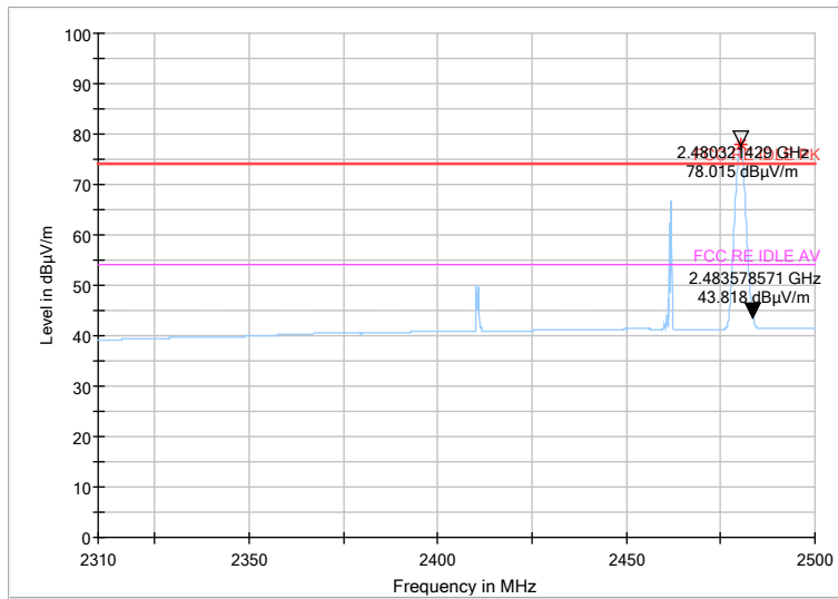
Average Detector
