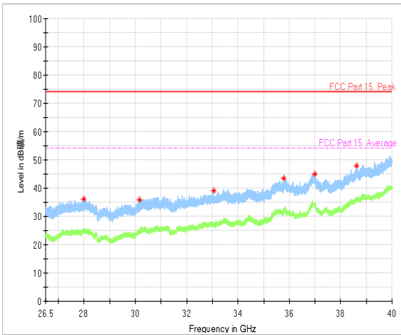
Radiated Spurious Emission (802.11n-HT40, ch151, 26.5GHz-40GHz)
