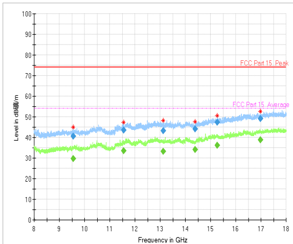
Radiated Spurious Emission (802.11n-HT40, ch151, 8GHz-18GHz)
