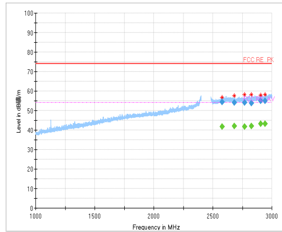
Bandedge:Ch39
