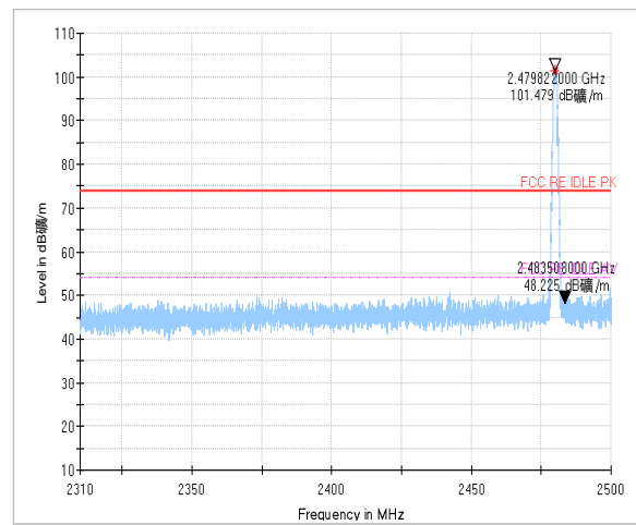
Bandedge:Ch39
