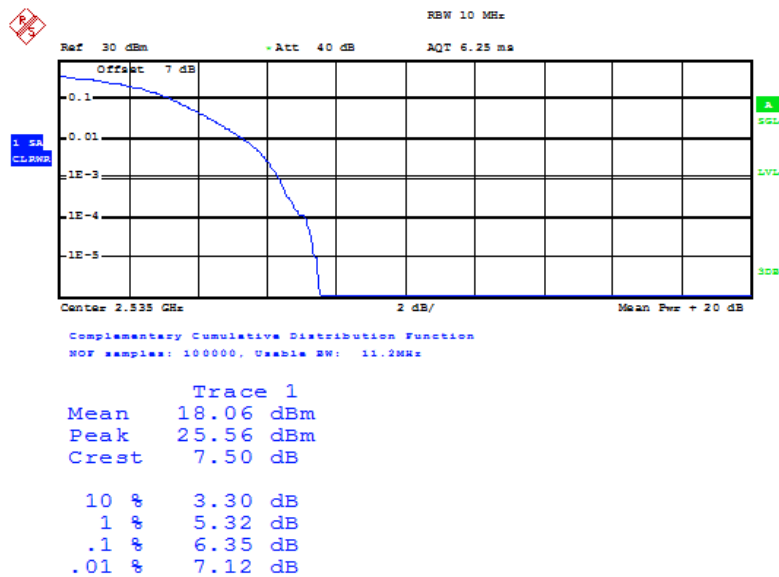
Fig.97 LTE band 7: QPSK
