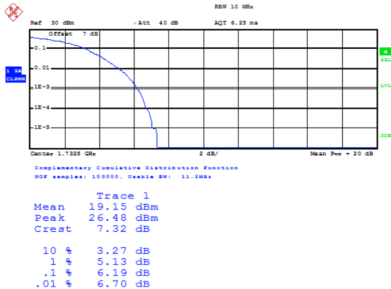
Fig.95 LTE band 4: QPSK
