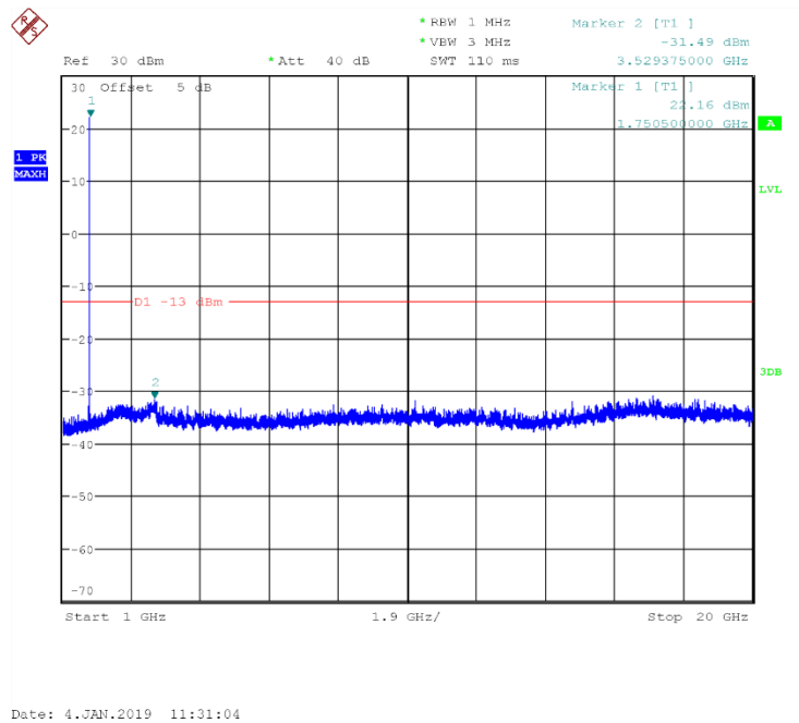
Channel 1513:1GHz~20GHz
