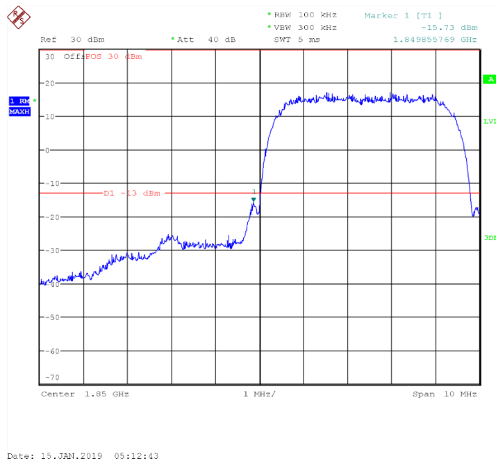
Channel 9262- LOW BAND EDGE BLOCK
