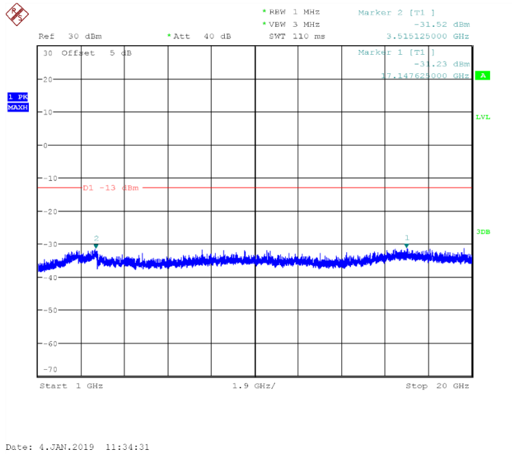
Channel 4233:1GHz~20GHz
