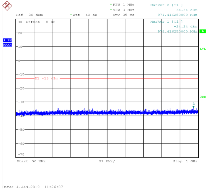
Channel 9262: 30MHz~1GHz
