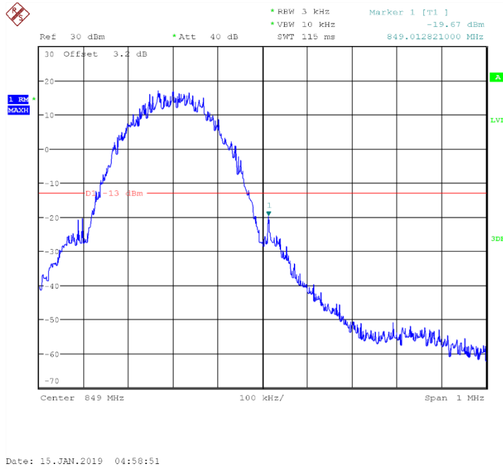
Channel 251- HIGH BAND EDGE BLOCK
