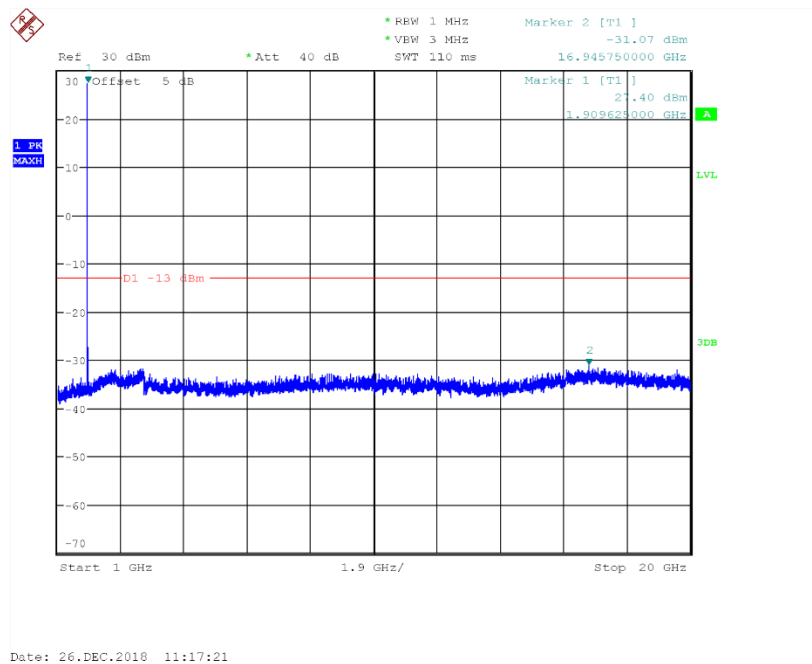
Channel 810: 1GHz~20GHz
