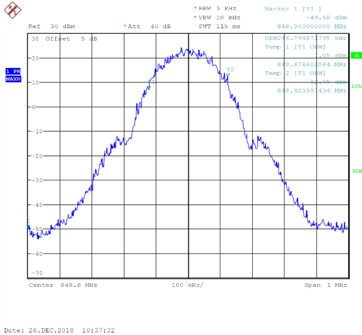
Channel 251-Occupied Bandwidth (99%)
