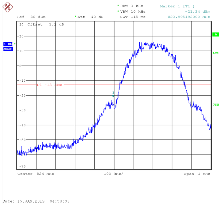
Channel 128- LOW BAND EDGE BLOCK
