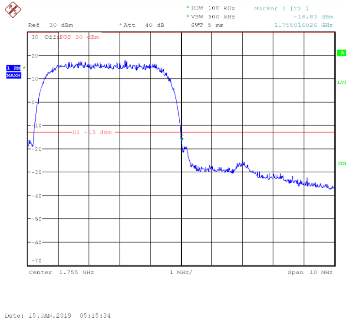
Channel 1513- HIGH BAND EDGE BLOCK
