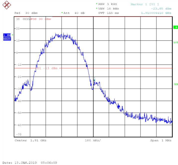
Channel 810- HIGH BAND EDGE BLOCK
