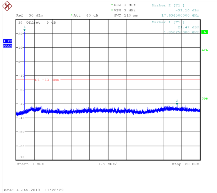
Channel 9262:1GHz~20GHz
