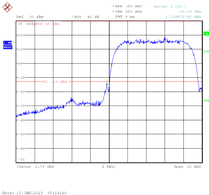
Channel 1312- LOW BAND EDGE BLOCK
