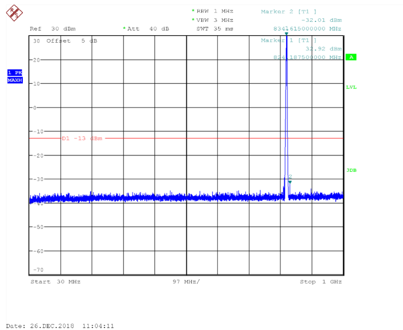
Channel 128: 30MHz~1GHz
