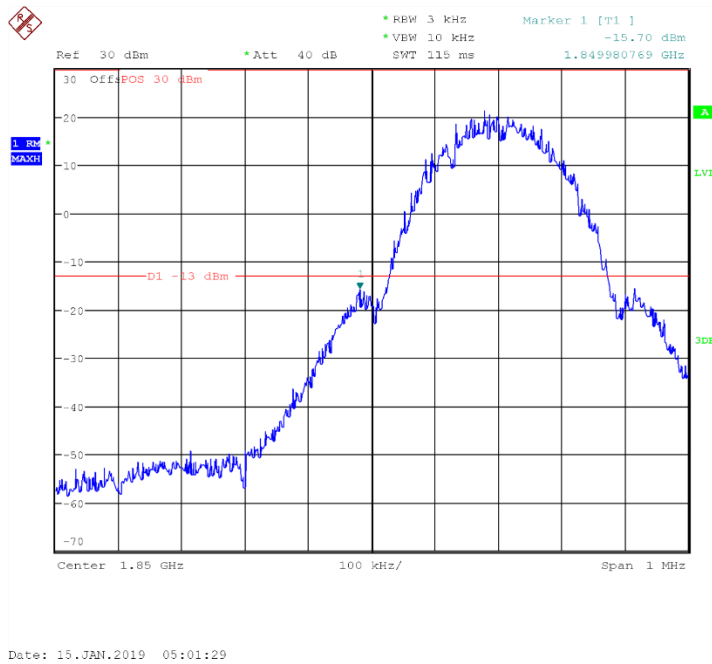
Channel 512- LOW BAND EDGE BLOCK
