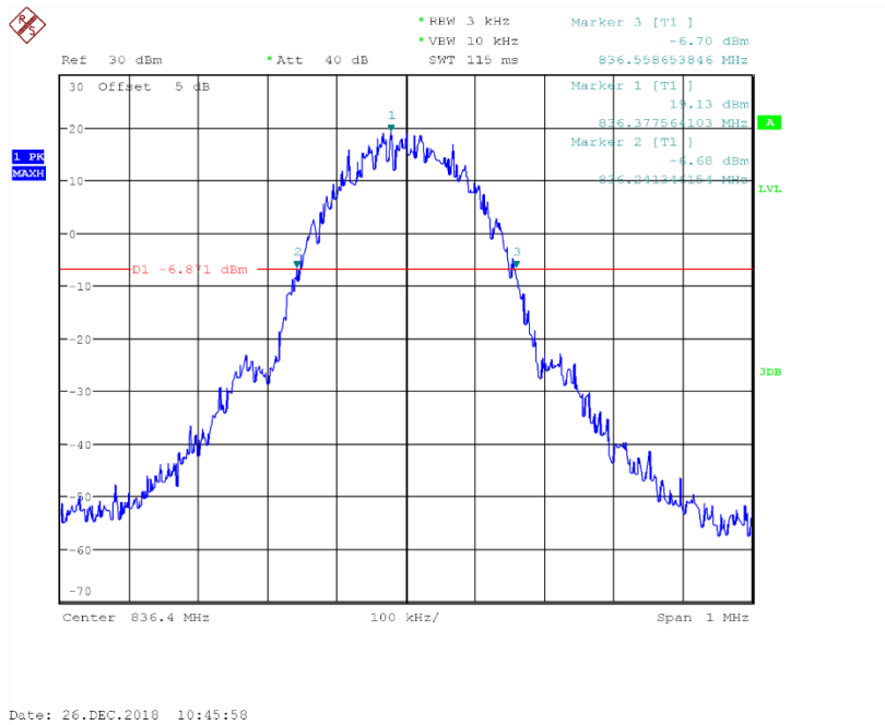
Channel 189- Emission Bandwidth (-26dBc BW)
