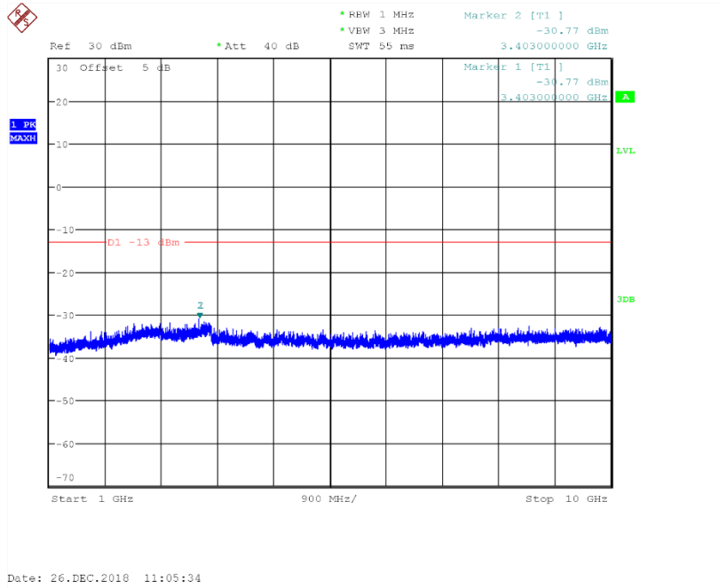
Channel 251: 1GHz~10GHz
