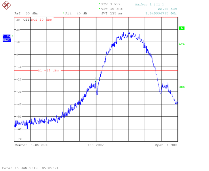
Channel 512- LOW BAND EDGE BLOCK
