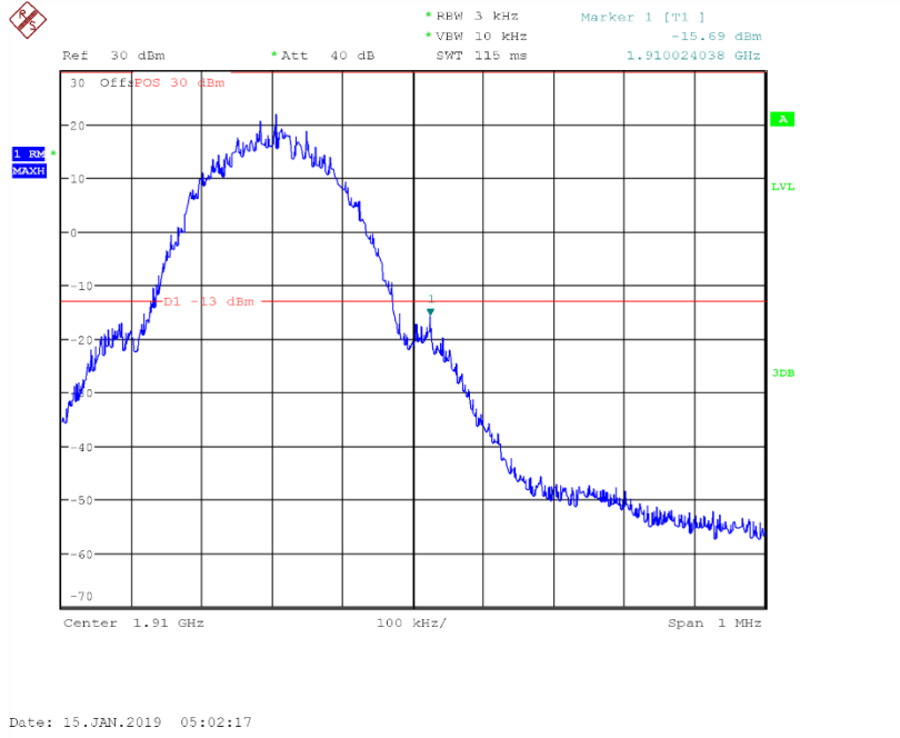
Channel 810- HIGH BAND EDGE BLOCK
