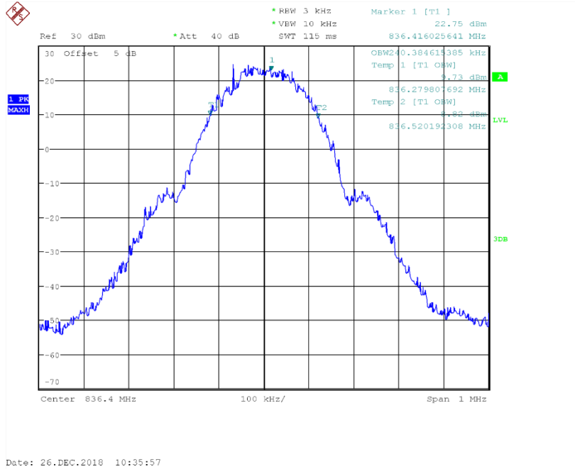
Channel 189-Occupied Bandwidth (99%)
