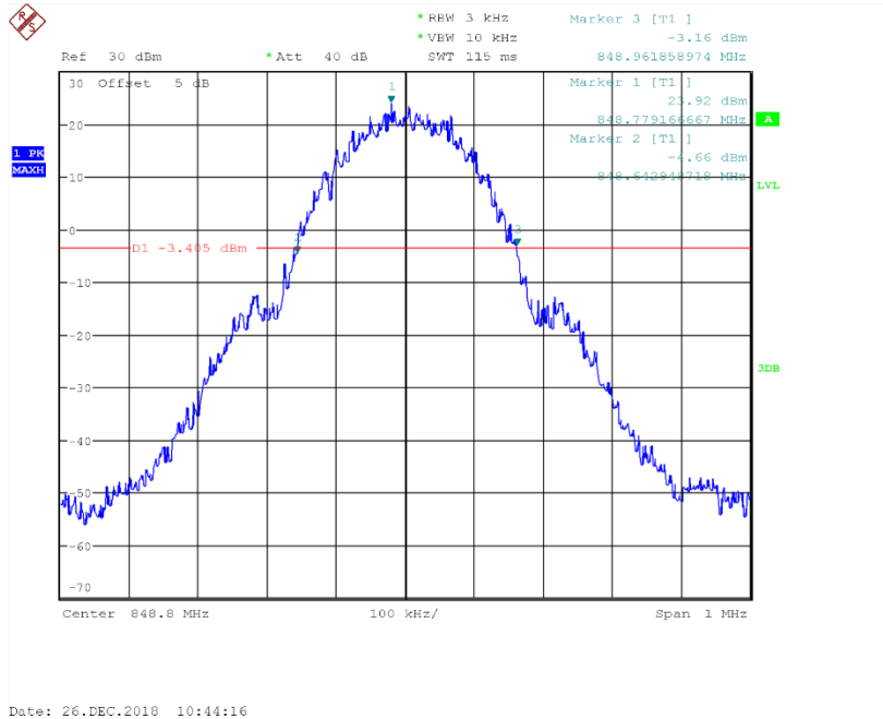
Channel 251- Emission Bandwidth (-26dBc BW)
