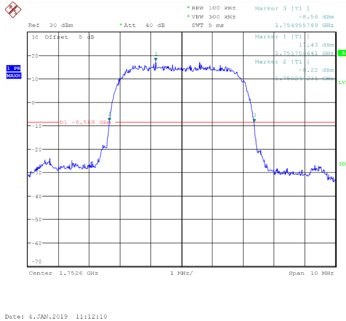
Channel 1513- Emission Bandwidth (-26dBc BW)
