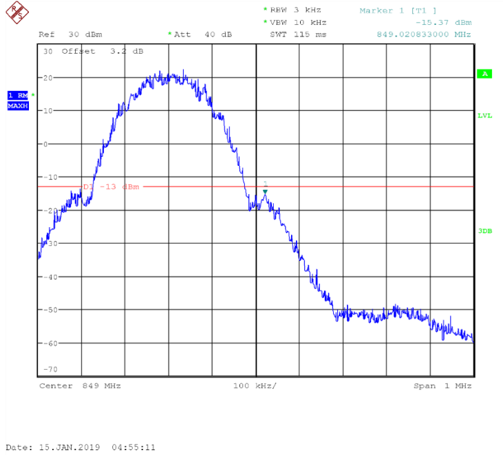
Channel 251- HIGH BAND EDGE BLOCK
