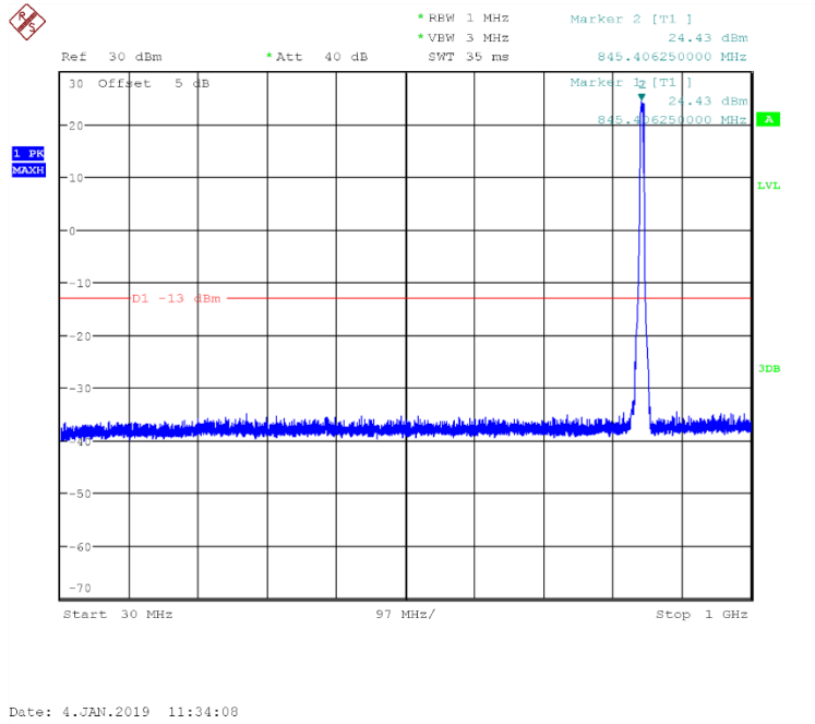
Channel 4233: 30MHz~1GHz
