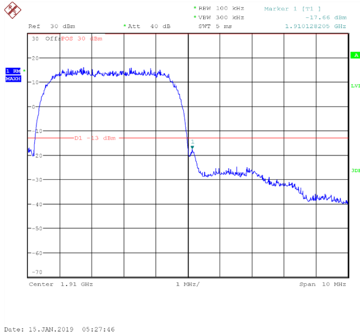
Channel 9538- HIGH BAND EDGE BLOCK
