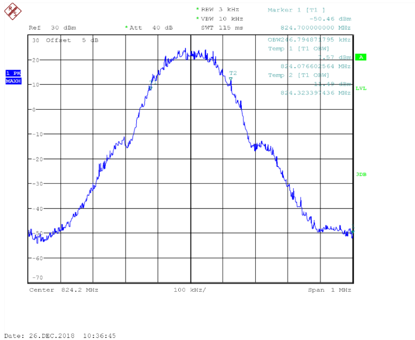
Channel 128-Occupied Bandwidth (99%)
