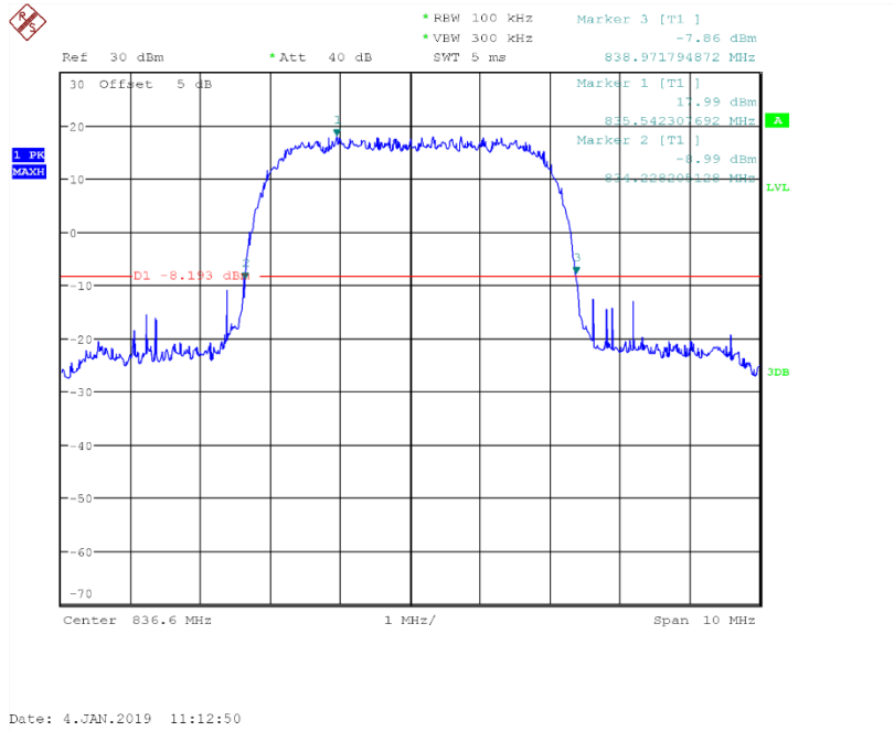
Channel 4183- Emission Bandwidth (-26dBc BW)
