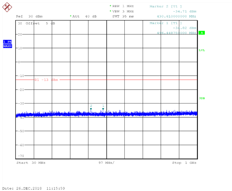
Channel 512: 30MHz~1GHz
