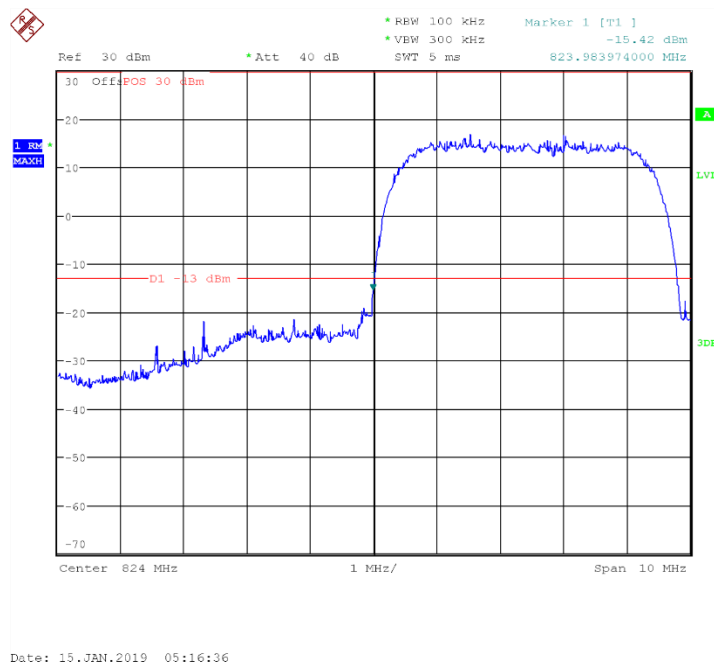
Channel 4132- LOW BAND EDGE BLOCK
