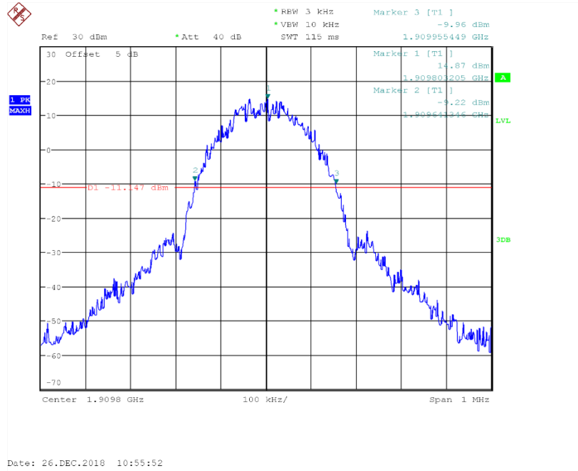
Channel 810- Emission Bandwidth (-26dBc BW)
