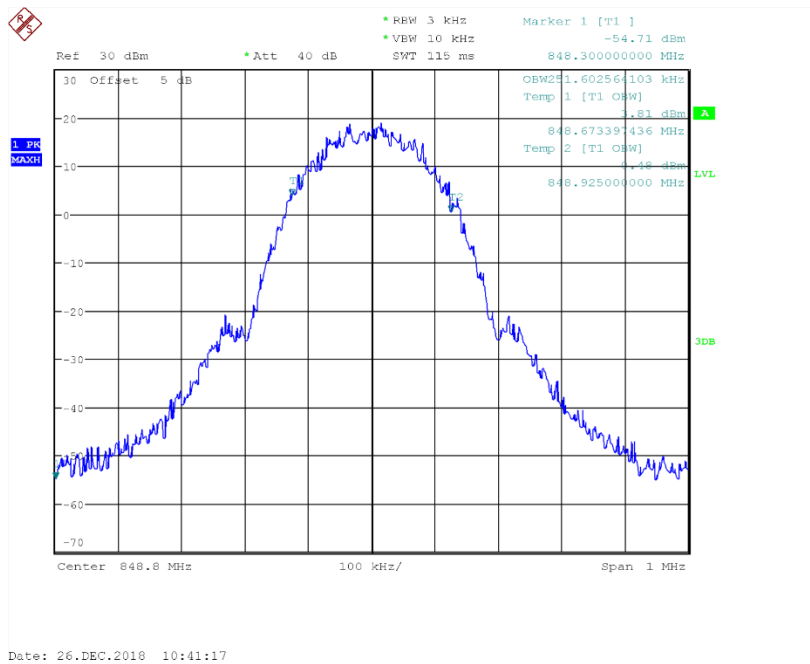
Channel 251-Occupied Bandwidth (99%)
