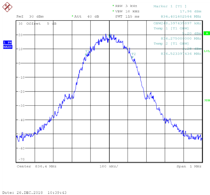
Channel 189-Occupied Bandwidth (99%)
