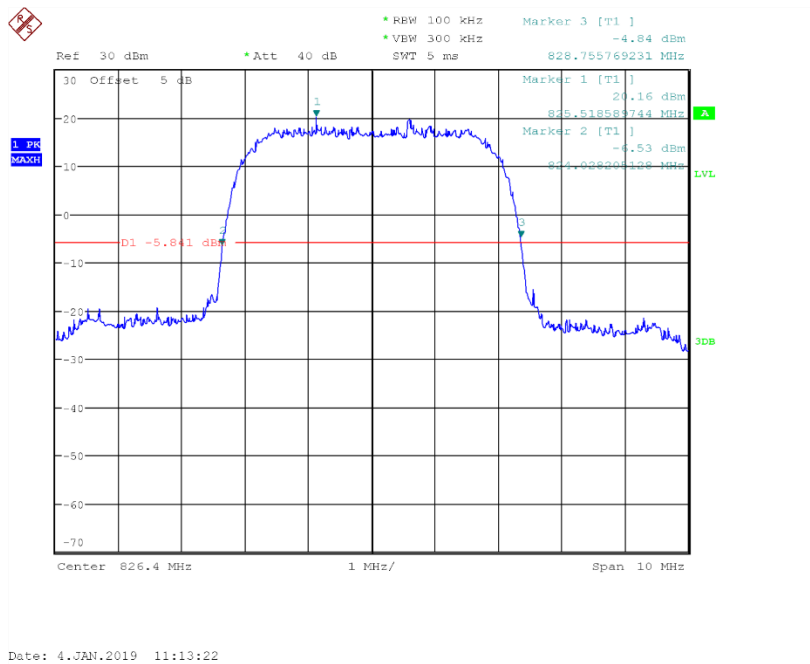
Channel 4132- Emission Bandwidth (-26dBc BW)
