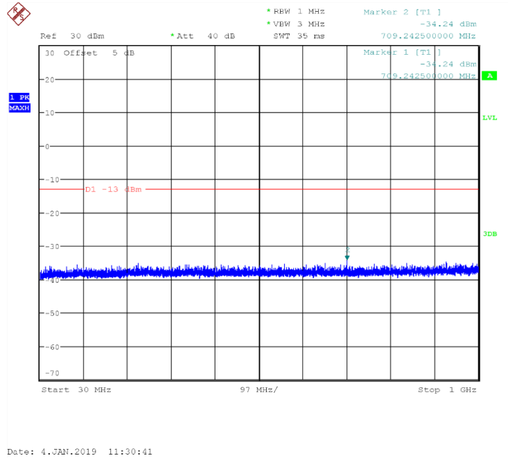
Channel 1513: 30MHz~1GHz
