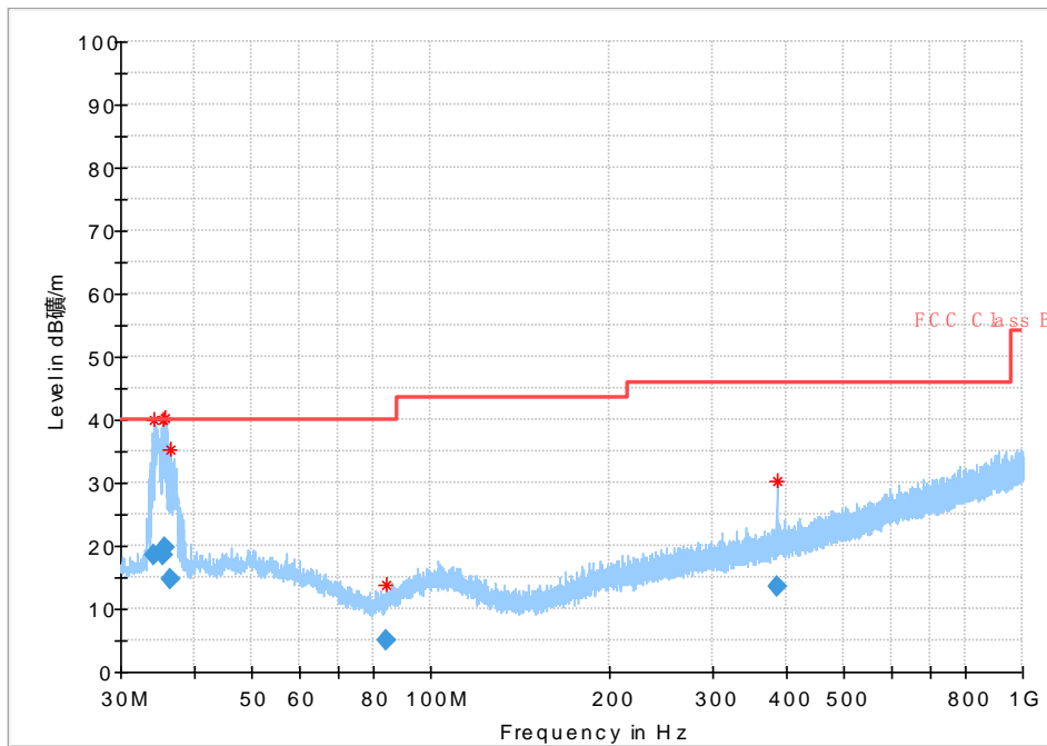
Fig. 42 Radiated Spurious Emission (802.11n-HT40, Ch151, 30 MHz-1 GHz)
