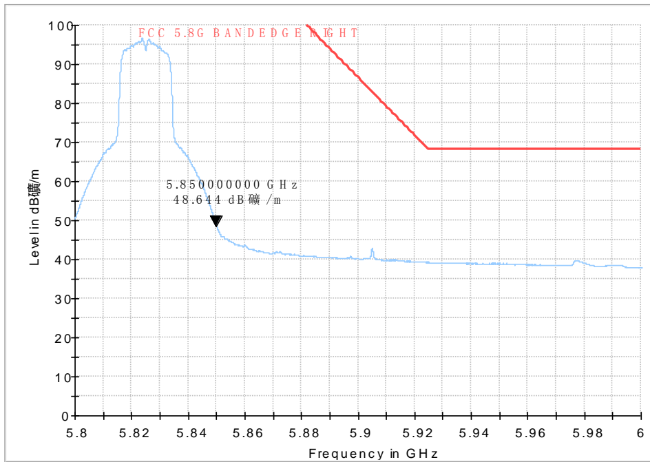
Fig. 50 Band Edges (802.11n-HT20, 5825MHz)
