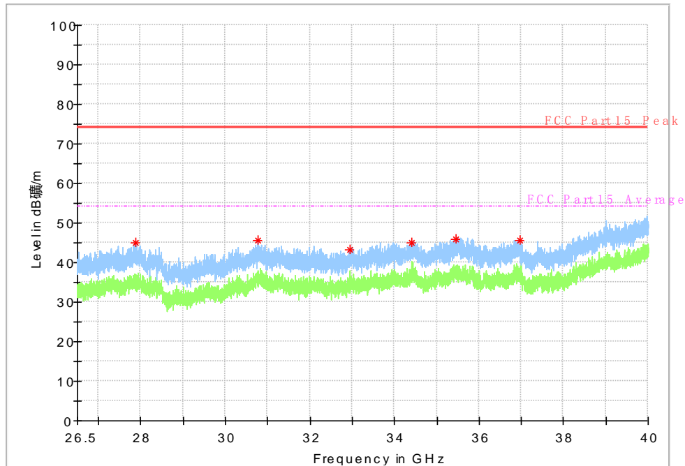
Fig. 46 Radiated emission: 802.11n, (802.11n-HT40, Ch151, 26.5 GHz - 40 GHz)
