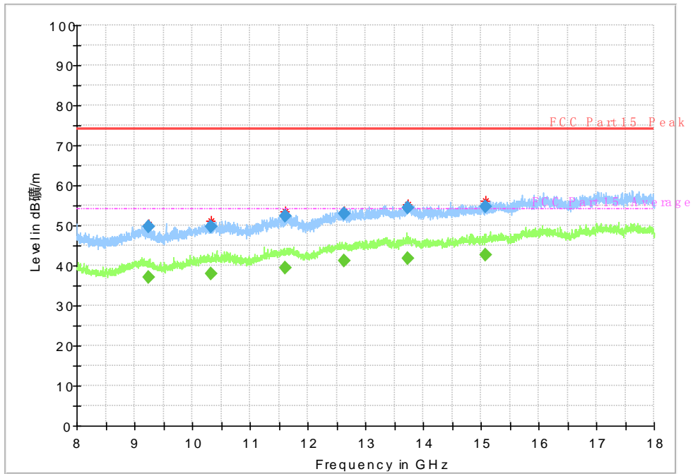
Fig. 44 Radiated Spurious Emission (802.11n-HT40, Ch151, 8 GHz-18 GHz)
