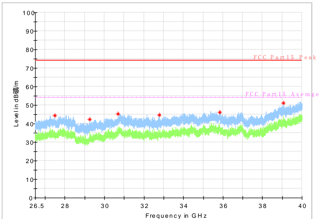
Fig. 48 Radiated Spurious Emission (802.11n-HT20, ch36, 26.5 GHz-40 GHz)
