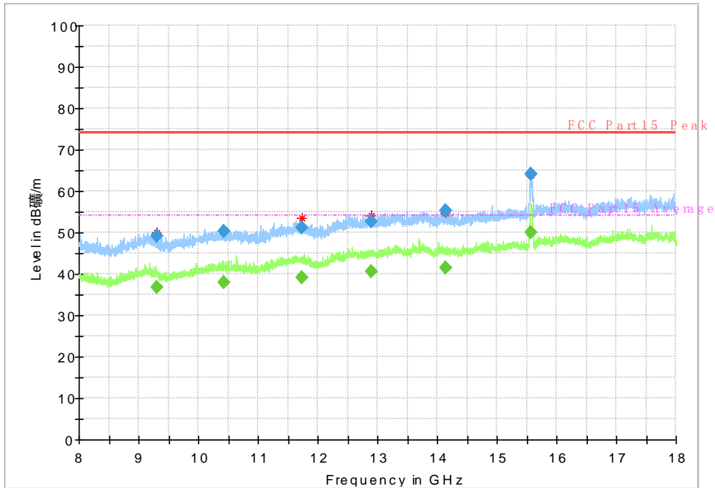
Fig. 57 Radiated Spurious Emission (802.11n-HT40, ch38, 8 GHz-18 GHz)
