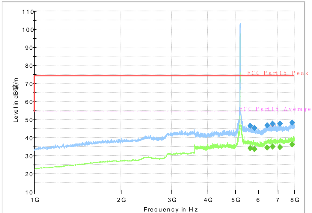
Fig. 45 Radiated Spurious Emission (802.11n-HT20, ch36, 1 GHz-8 GHz)
