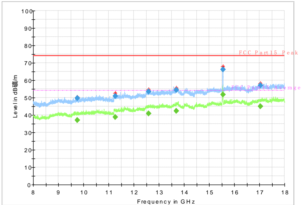
Fig. 41 Radiated Spurious Emission (802.11a, ch36, 8 GHz-18 GHz)
