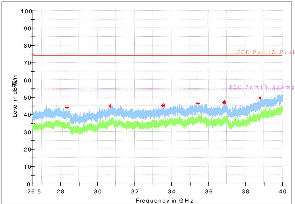
Fig. 43 Radiated Spurious Emission (802.11a, ch36, 26.5 GHz-40 GHz)
