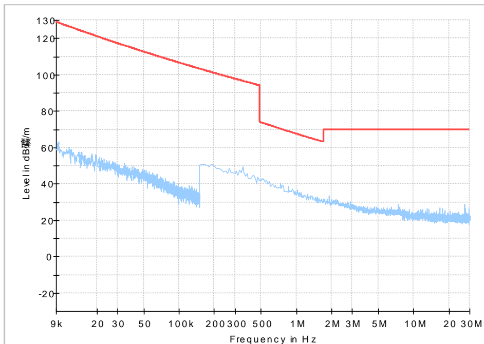
Fig. 54 Radiated Spurious Emission (9kHz-30MHz)
