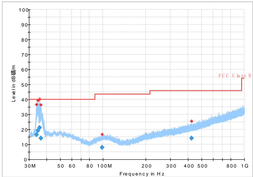
Fig. 55 Radiated Spurious Emission (802.11n-HT40, ch38, 30 MHz-1 GHz)
