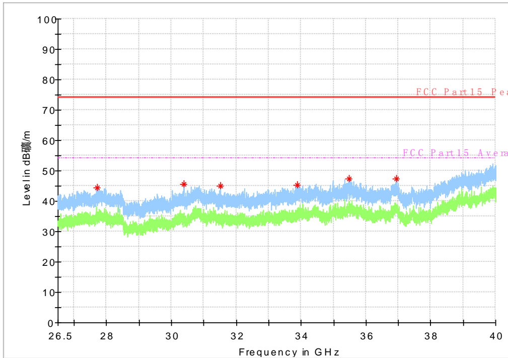
Fig. 53 Radiated Spurious Emission (802.11n-HT40, ch38, 26.5 GHz-40 GHz)
