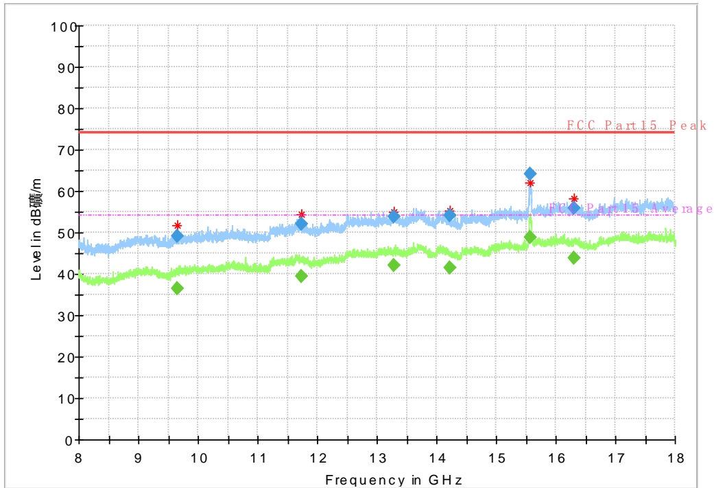
Fig. 51 Radiated Spurious Emission (802.11n-HT40, ch38, 8 GHz-18 GHz)
