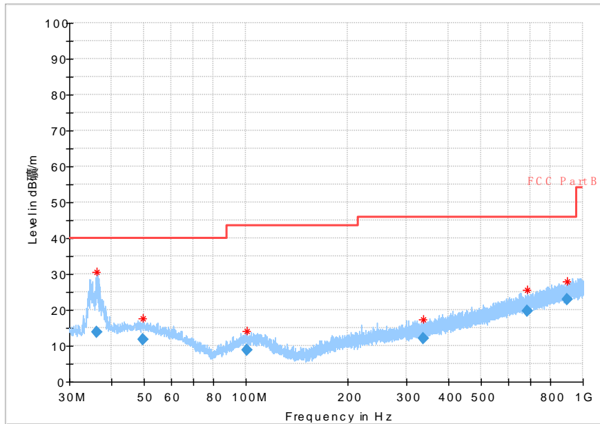
Fig.60 Radiated Spurious Emission (802.11g,Ch11,30MHz~1GHz)
