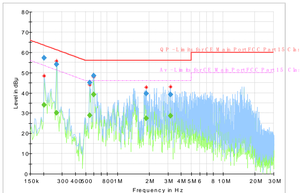
Fig.64 AC Powerline Conducted Emission
