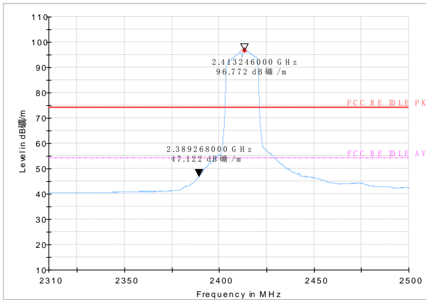
Fig.58 Radiated emission (Power): 802.11g, low channel
