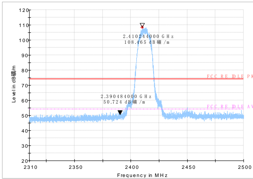
Peak detector
