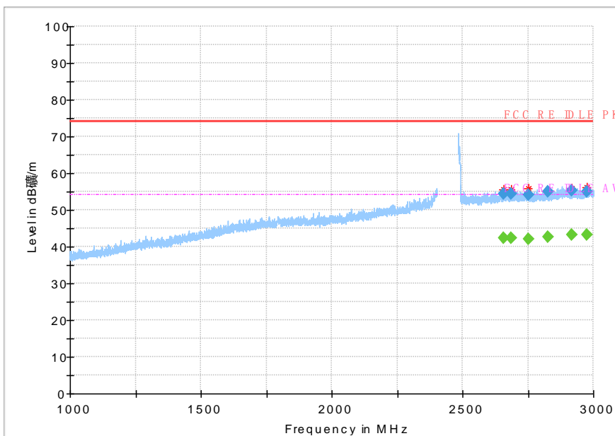
Fig.61 Radiated Spurious Emission (802.11g,Ch11,1GHz~3GHz)
