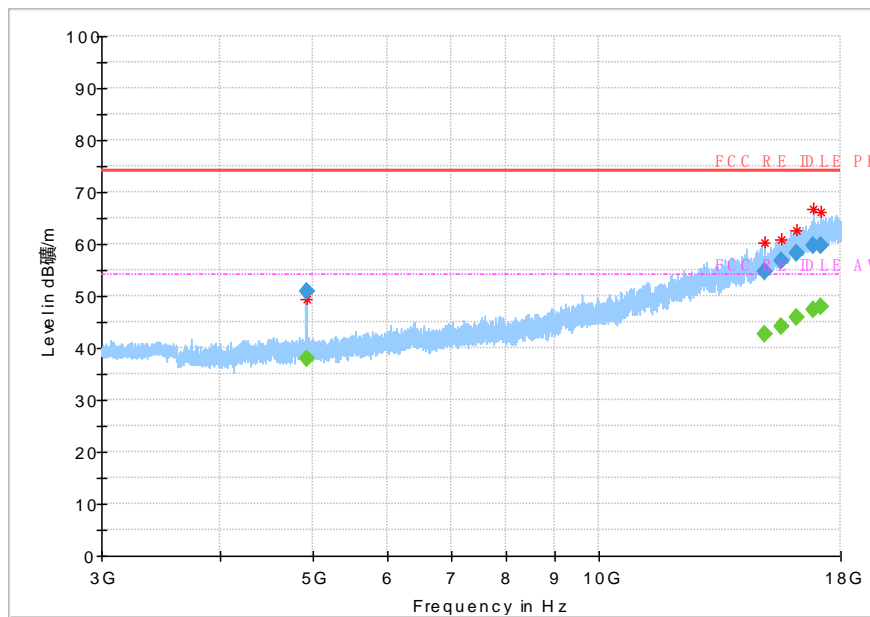
Fig.62 Radiated Spurious Emission (802.11g,Ch11,3GHz~18GHz)
