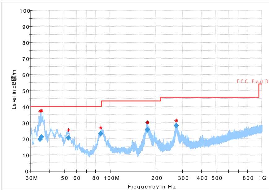
Fig.55 Radiated Spurious Emission (802.11 n-20MHz,Ch11,30MHz~1GHz)
