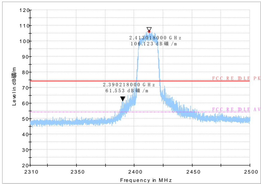
Peak detector
