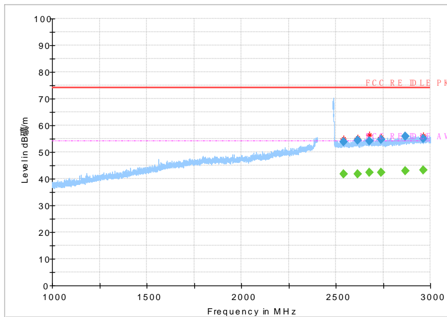
Fig.56 Radiated Spurious Emission (802.11 n-20MHz,Ch11,1GHz~3GHz)
