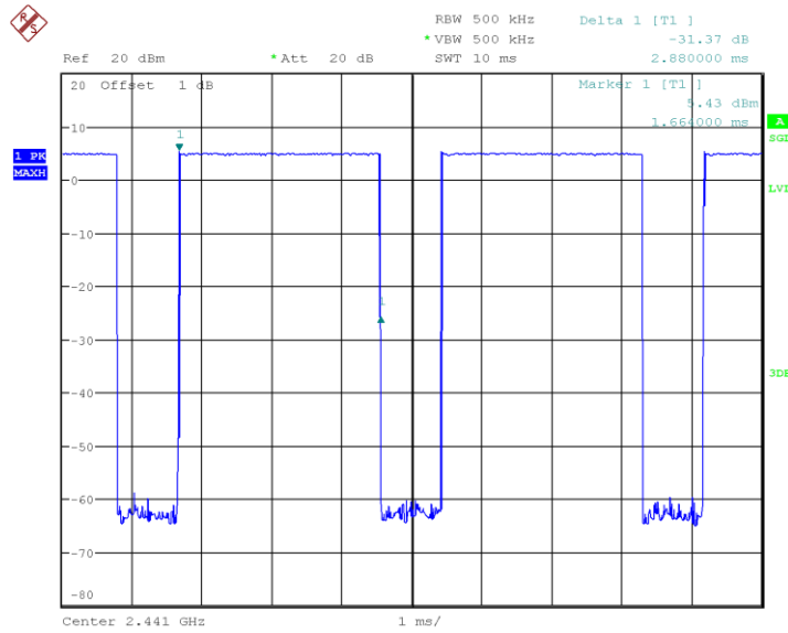
Fig.63 Number of Transmissions Measurement: Ch39, Packet DH3
