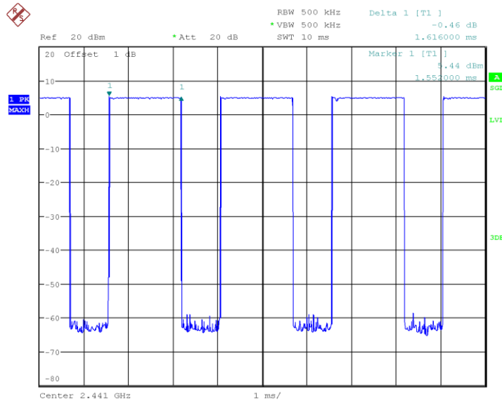
Fig.61 Number of Transmissions Measurement: Ch39, Packet DH1
