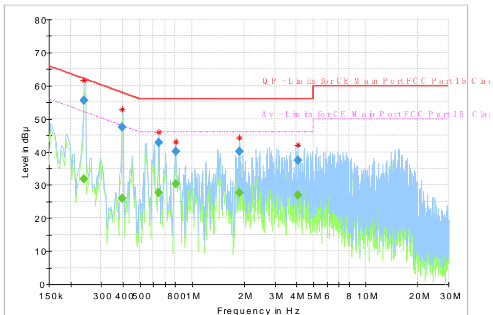
Fig.97 AC Powerline Conducted Emission
