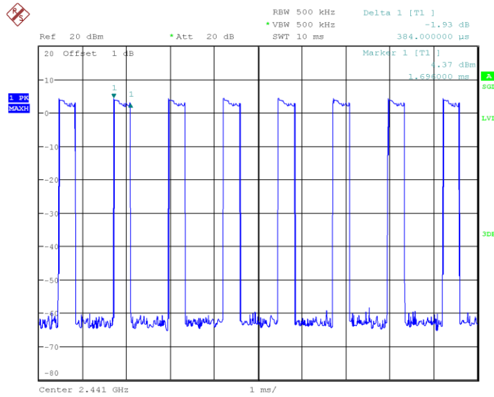
Fig.71 Number of Transmissions Measurement: Ch39, Packet 2-DH5
