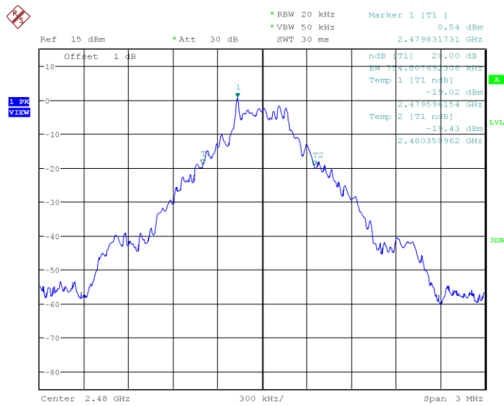
Fig.79 20dB Bandwidth: GFSK, Ch39
