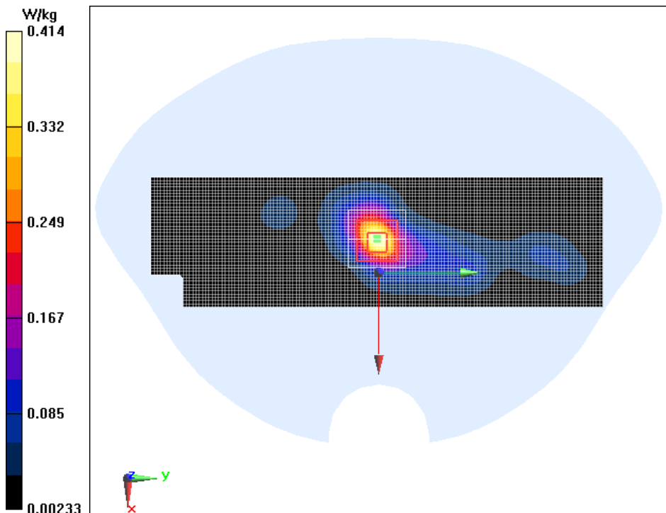
Fig.5 WIFI2450 Right Mode High 0mm
