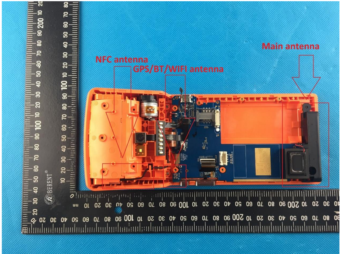
Main antenna
