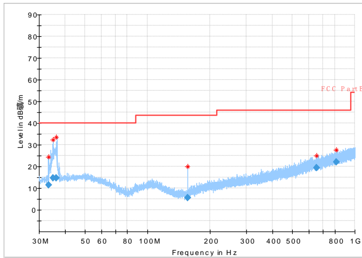
Fig.1 Radiated emission: Ch0, 30MHz~1GHz
