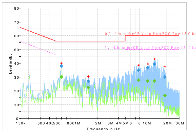
Fig.4 AC Power line Conducted Emission
