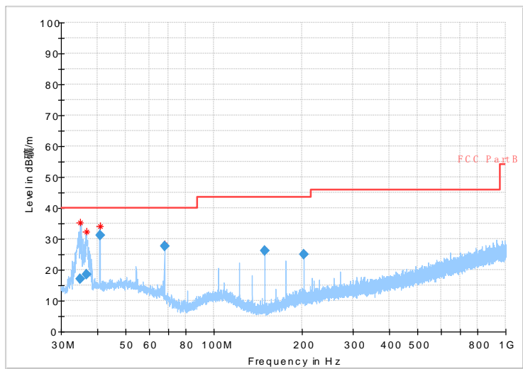
Fig 11 Radiated emission: 8DPSK, Ch0, 30MHz~1GHz
