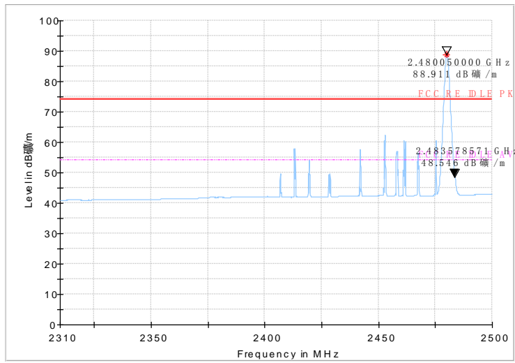
Average Detector
