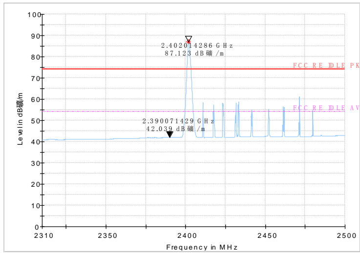
Fig 4 Radiated emission (Power): GFSK, low channel
