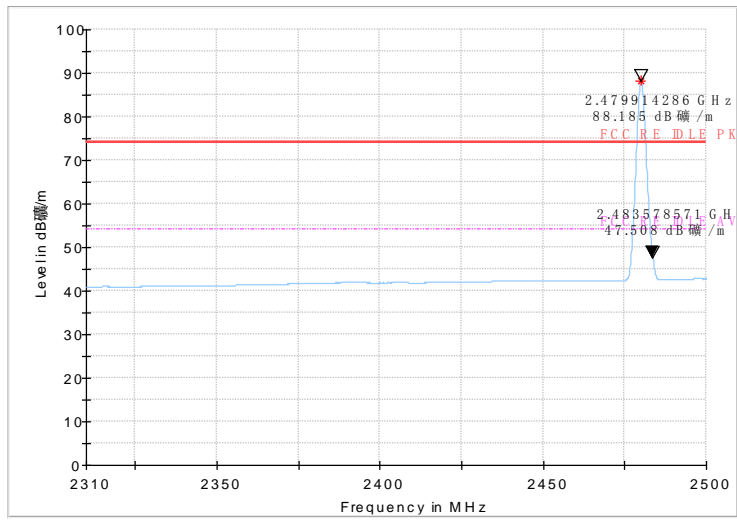
Fig 10 Radiated emission (Power): \pi/4 DQPSK, high channel
