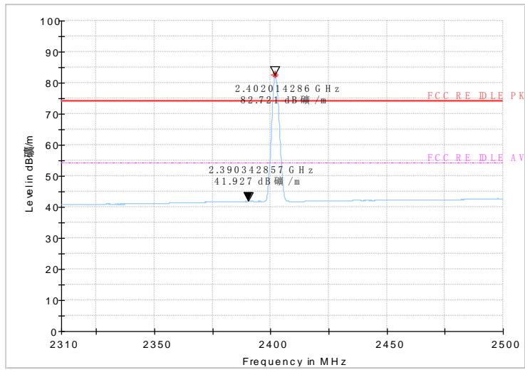
Fig 14 Radiated emission (Power): 8DPSK, low channel
