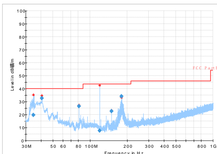
Fig 1 Radiated emission: GFSK, Ch0, 30MHz~1GHz
