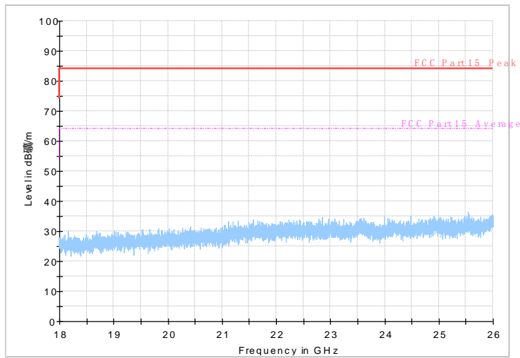
Fig 15 Radiated emission (Power): 8DPSK, high channel
