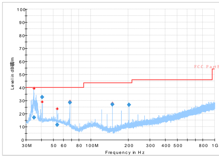
Fig 6 Radiated emission: \pi/4 DQPSK, Ch0, 30MHz~1GHz
