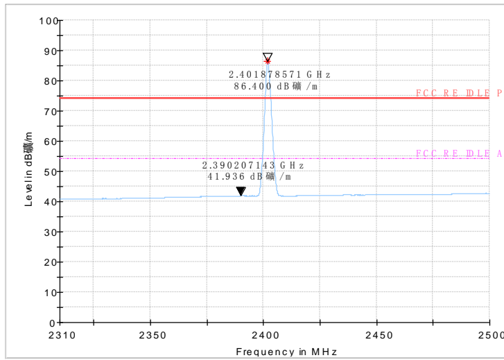
Fig 9 Radiated emission (Power): \pi/4 DQPSK, low channel
