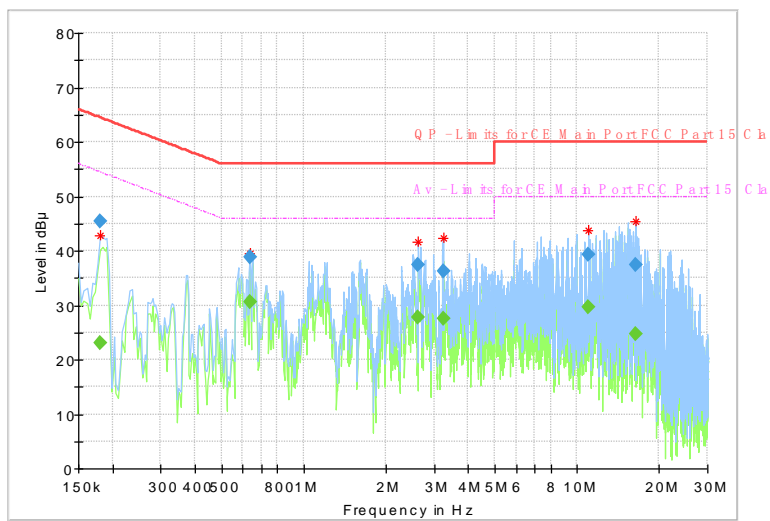
Fig 16 AC Power line Conducted Emission
