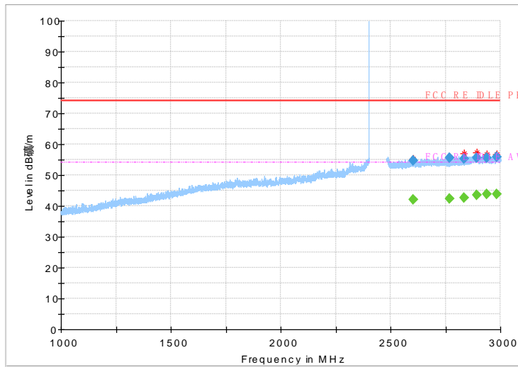
Fig 7 Radiated emission: \pi/4 DQPSK, Ch0, 1GHz~3GHz
