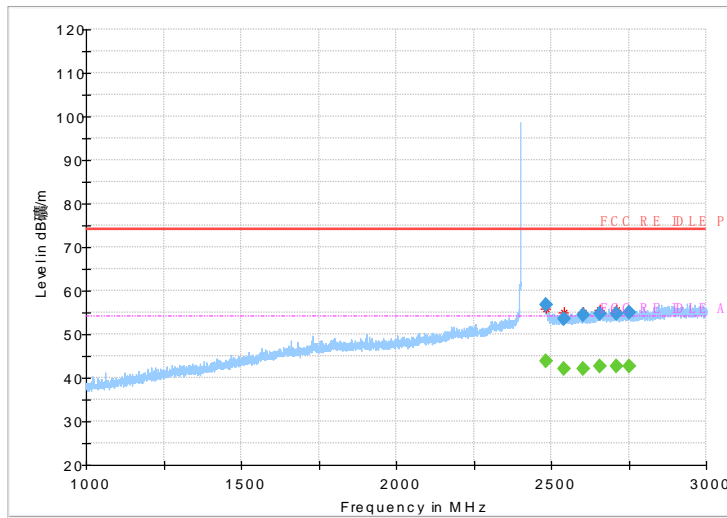
Fig 2 Radiated emission: GFSK, Ch0, 1GHz~3GHz
