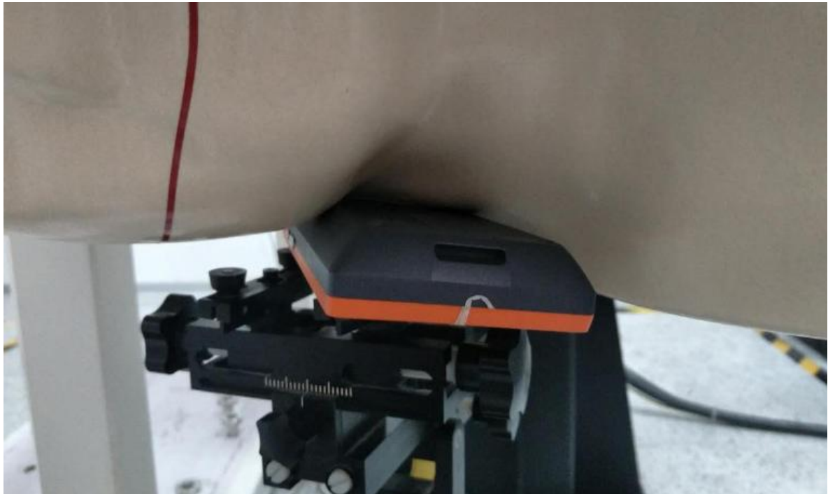
POSITION OF BODY BACK FOR WLAN WITH 0mm DISTANCE
