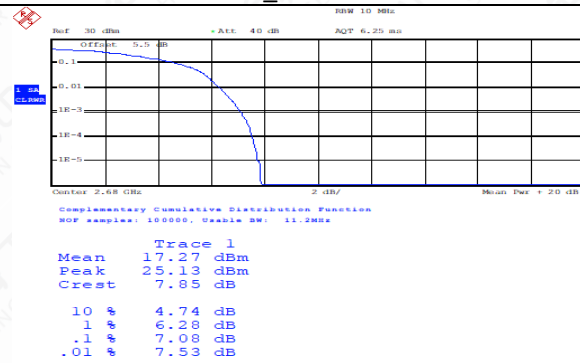
TDD41_HighRange_20MHz_2680_fullIRB_QPSK
