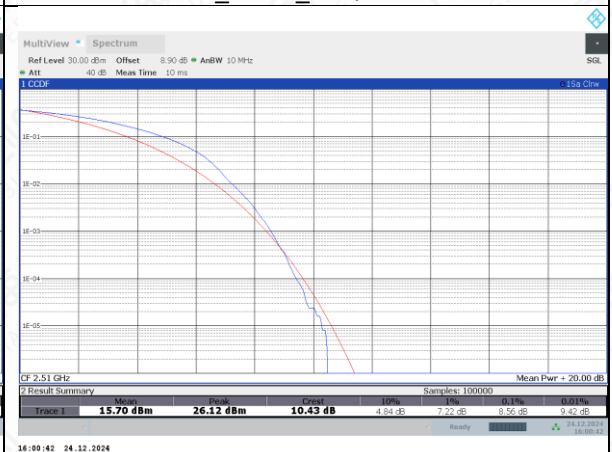
TDD41_Normal_LowRange_20MHz_2510_fullIRB_64QAM
