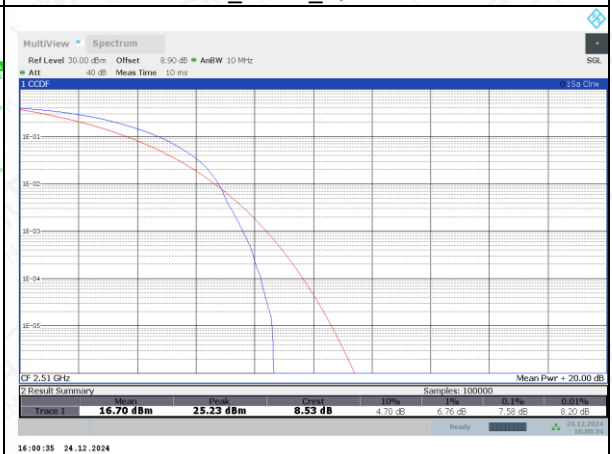
TDD41_Normal_LowRange_20MHz_2510_fullIRB_64QAM
