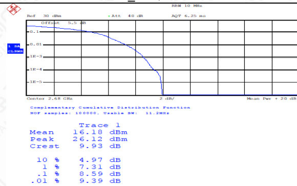
TDD41_HighRange_20MHz_2680_fullIRB_64QAM
