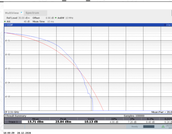
TDD41_Normal_LowRange_20MHz_2510_fullIRB_16QAM
