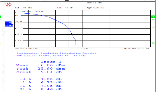
TDD41_HighRange_20MHz_2680_fullIRB_16QAM
