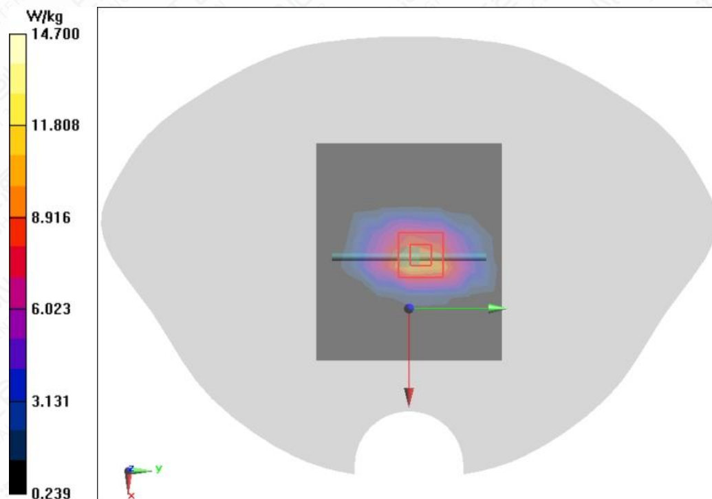
Figure A.2-7 System Check 1750MHz
