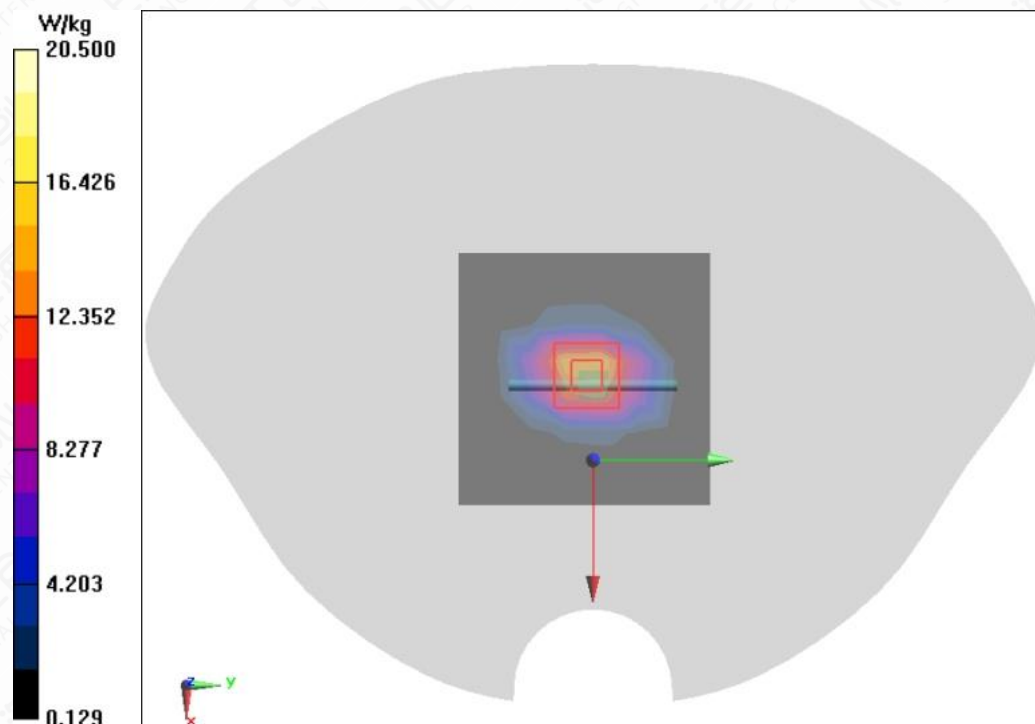
Figure A.2-12 System Check 2300MHz
