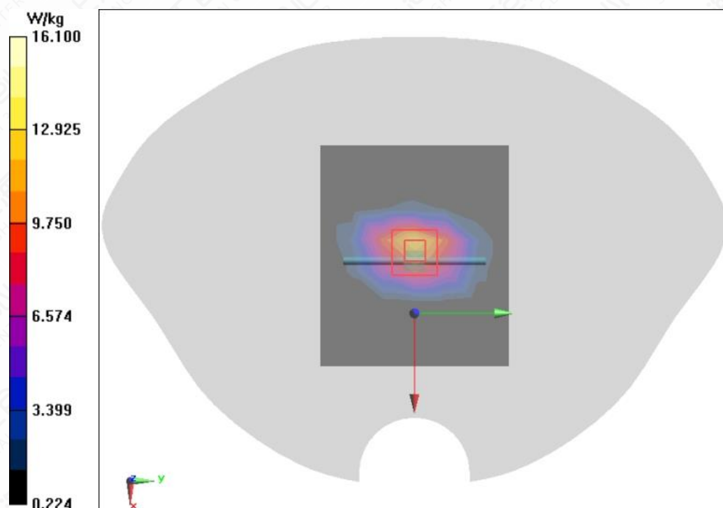
Figure A.2-10 System Check 1900MHz
