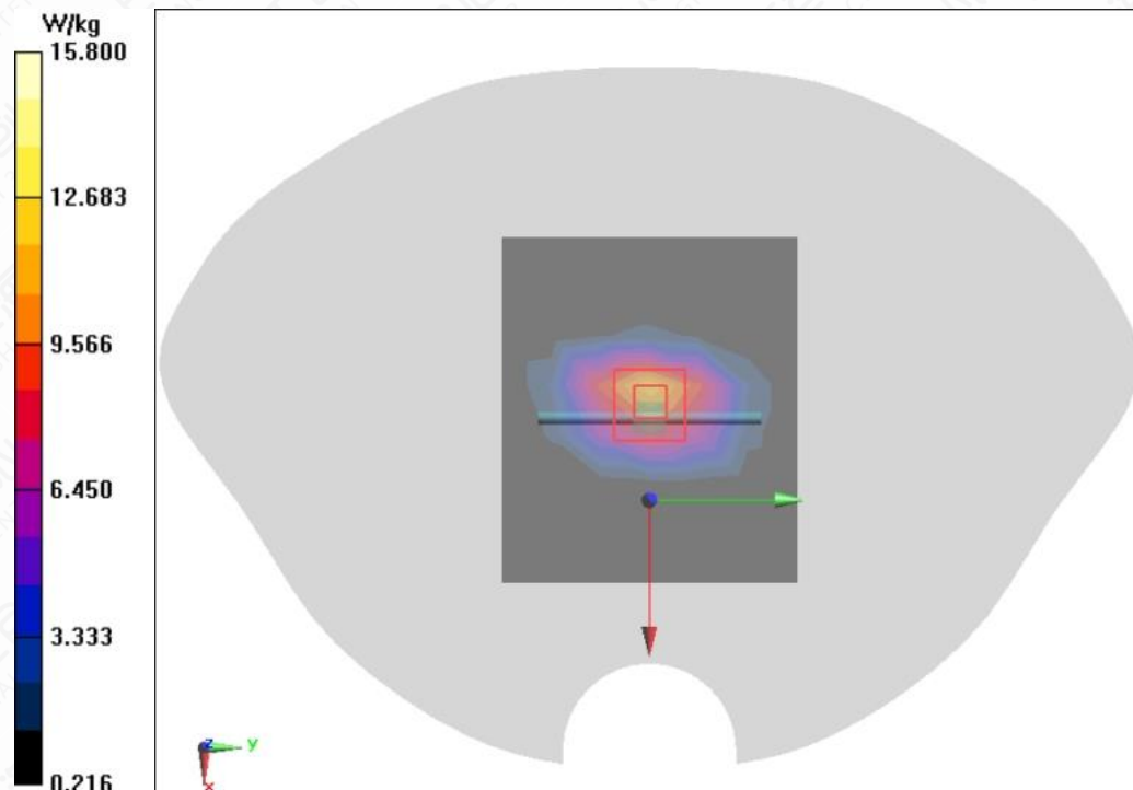
Figure A.2-11 System Check 1900MHz
