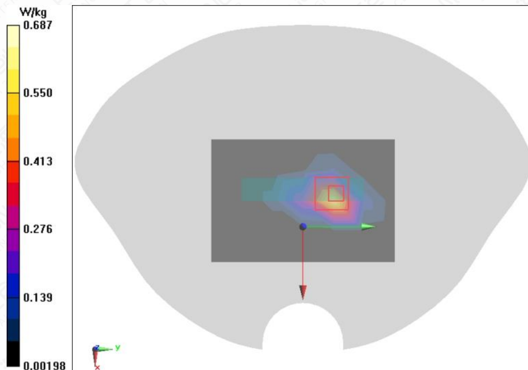
Figure A.1-76 BT DH5 Top Side Mode Low 0mm
