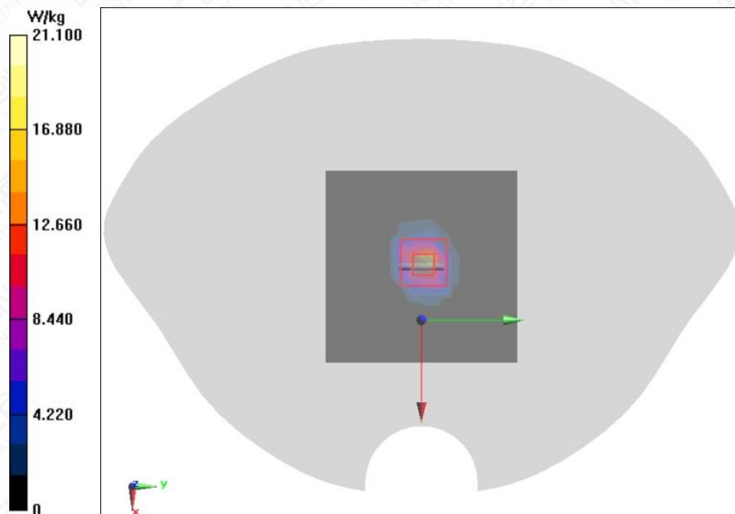
Figure A.2-19 System Check 5800MHz
