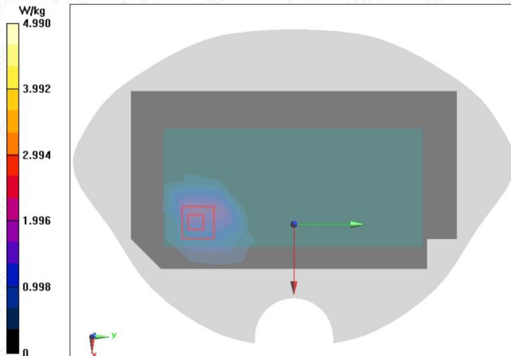
Figure A.1-69 Wi-Fi5G U-NII-2C 802.11a Back Side Mode High 0mm
