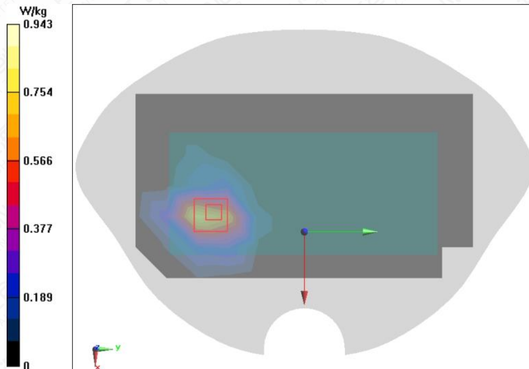
Figure A.1-68 Wi-Fi5G U-NII-2C 802.11a Back Side Mode High 10mm
