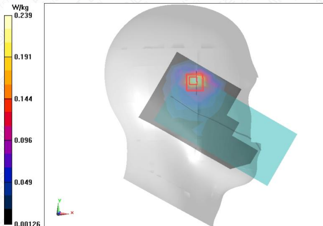
Figure A.1-73 BT DH5 Left Touch Mode Low
