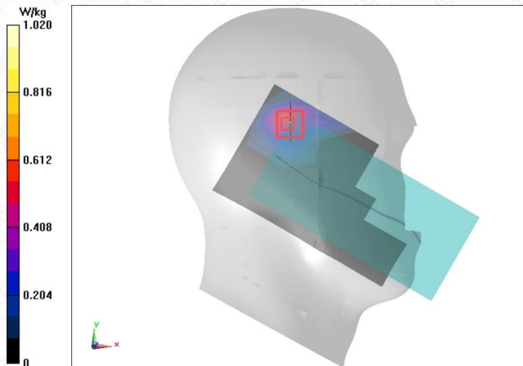
Figure A.1-70 Wi-Fi5G U-NII-3 802.11a Left Touch Mode Middle
