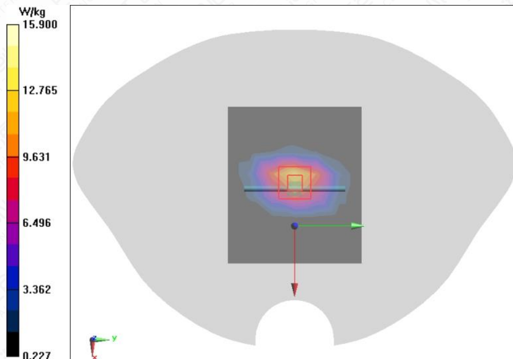
Figure A.2-9 System Check 1900MHz
