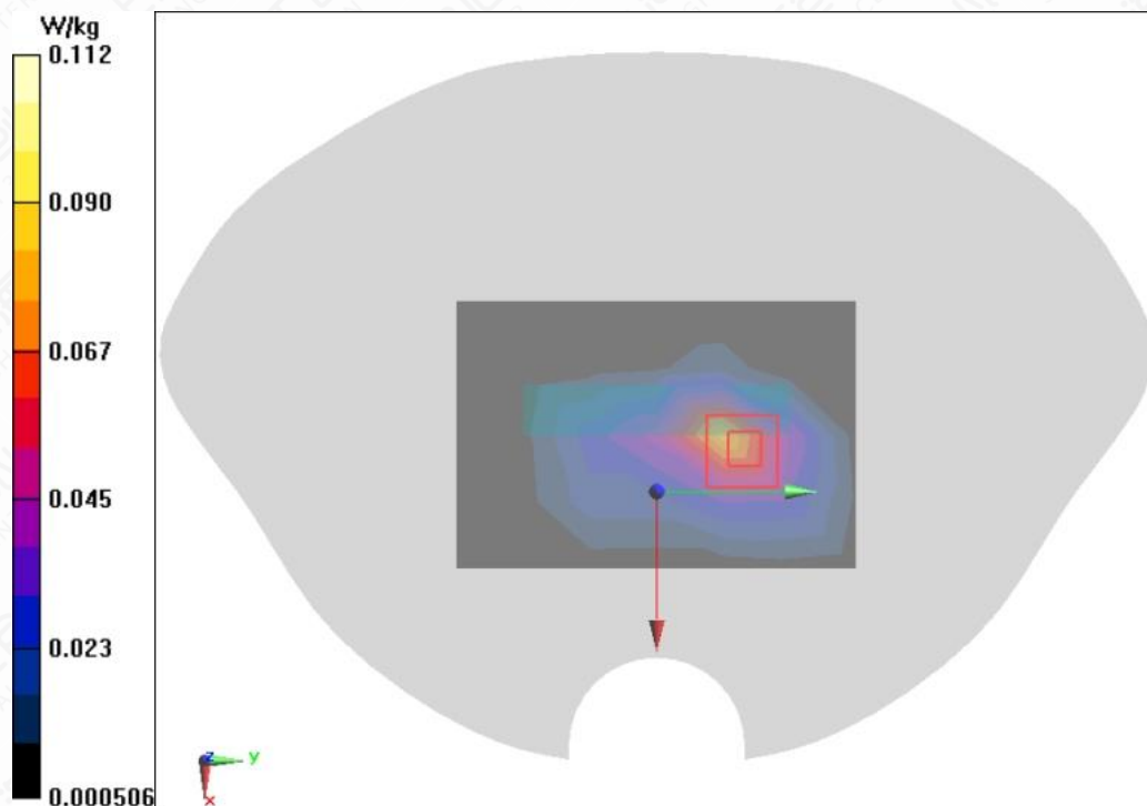
Figure A.1-75 BT DH5 Top Side Mode Middle 10mm
