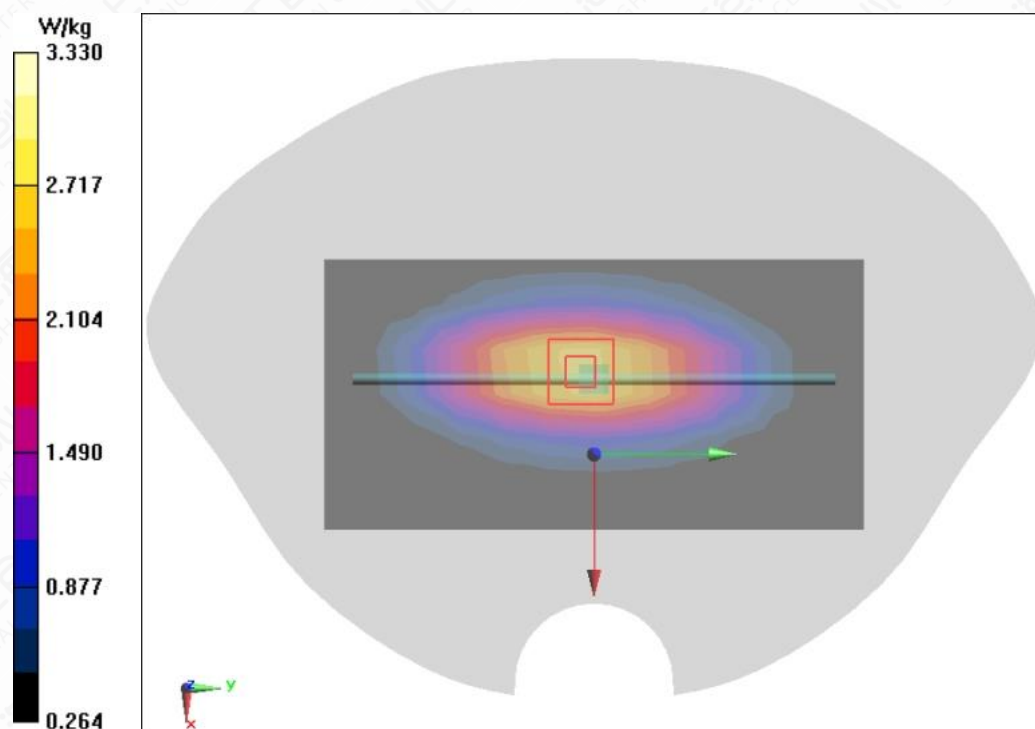
Figure A.2-5 System Check 835MHz
