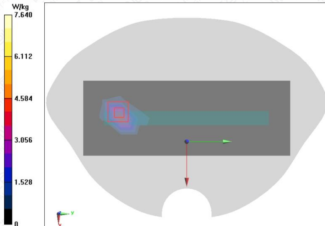
Figure A.1-72 Wi-Fi5G U-NII-3 802.11a Right Side Mode Middle 0mm
