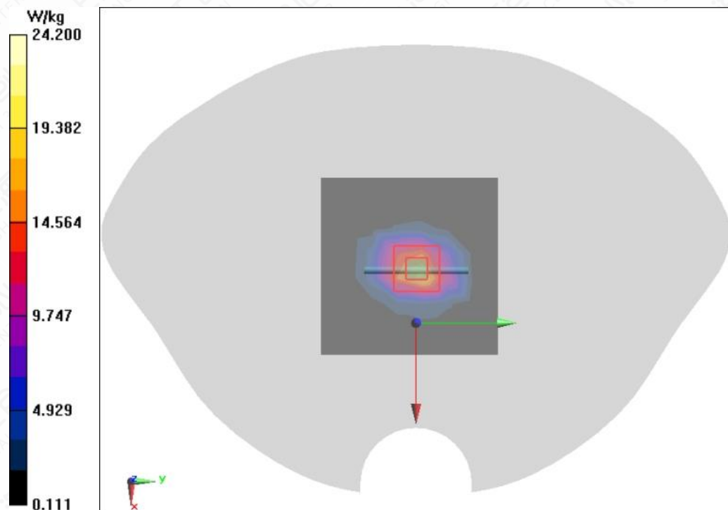
Figure A.2-15 System Check 2600MHz
