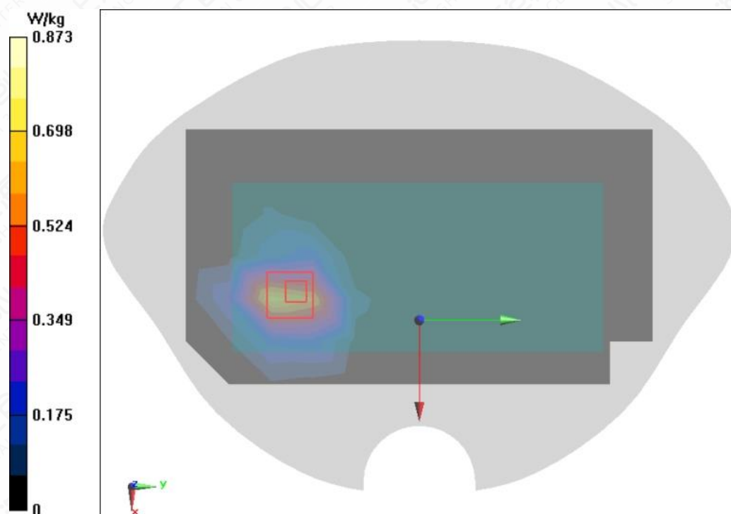
Figure A.1-71 Wi-Fi5G U-NII-3 802.11a Back Side Mode Middle 10mm
