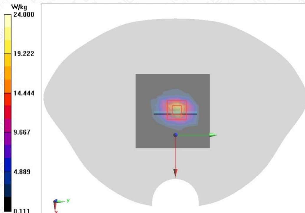
Figure A.2-14 System Check 2600MHz
