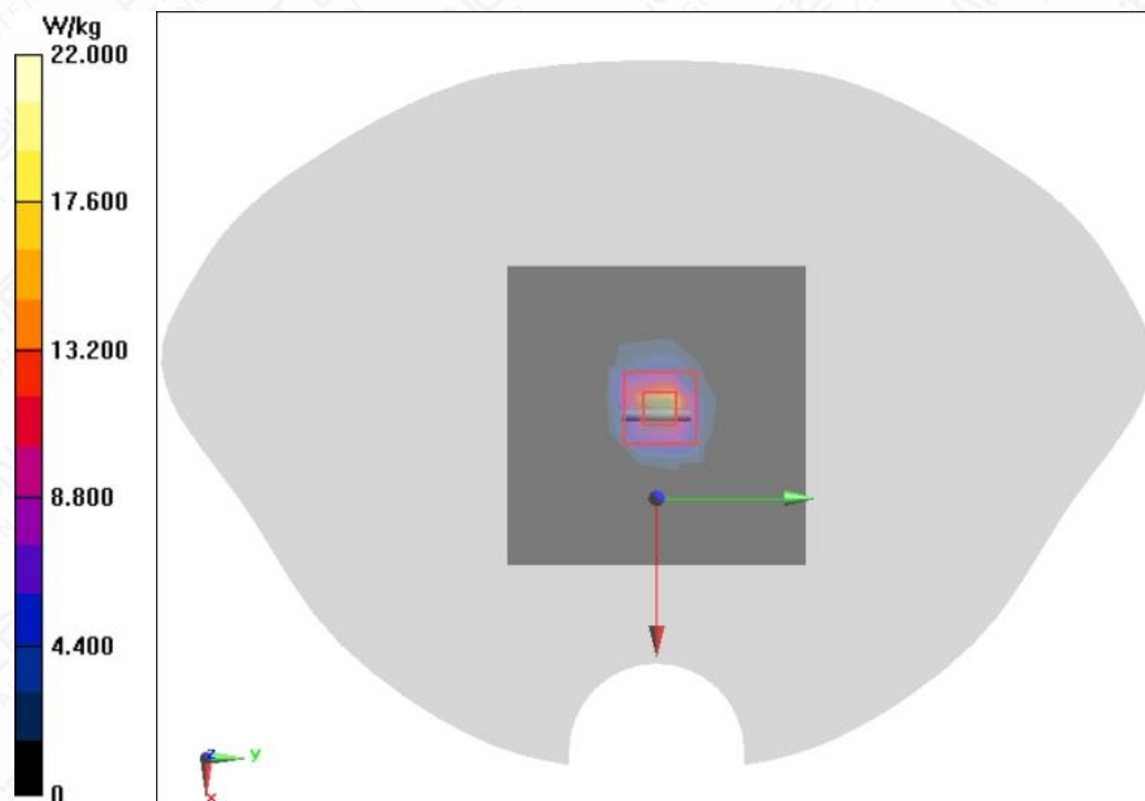
Figure A.2-18 System Check 5600MHz
