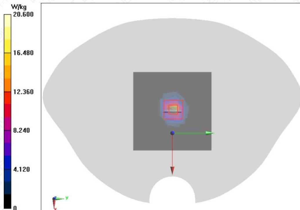
Figure A.2-17 System Check 5300MHz
