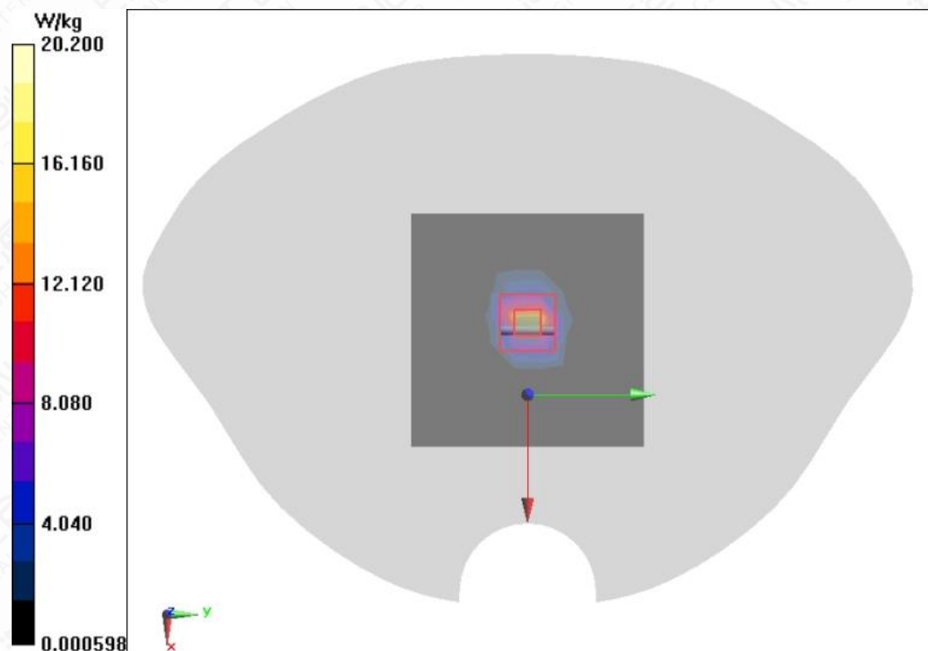
Figure A.2-16 System Check 5200MHz
