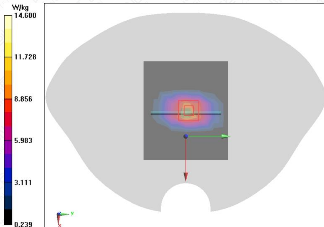
Figure A.2-8 System Check 1750MHz
