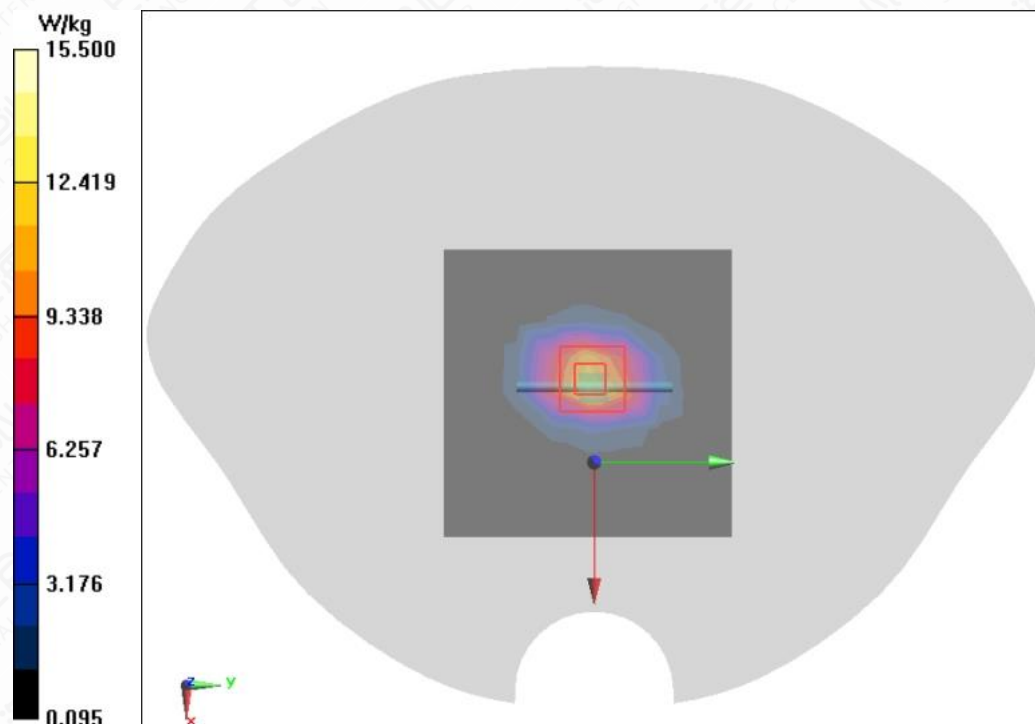
Figure A.2-13 System Check 2450MHz
