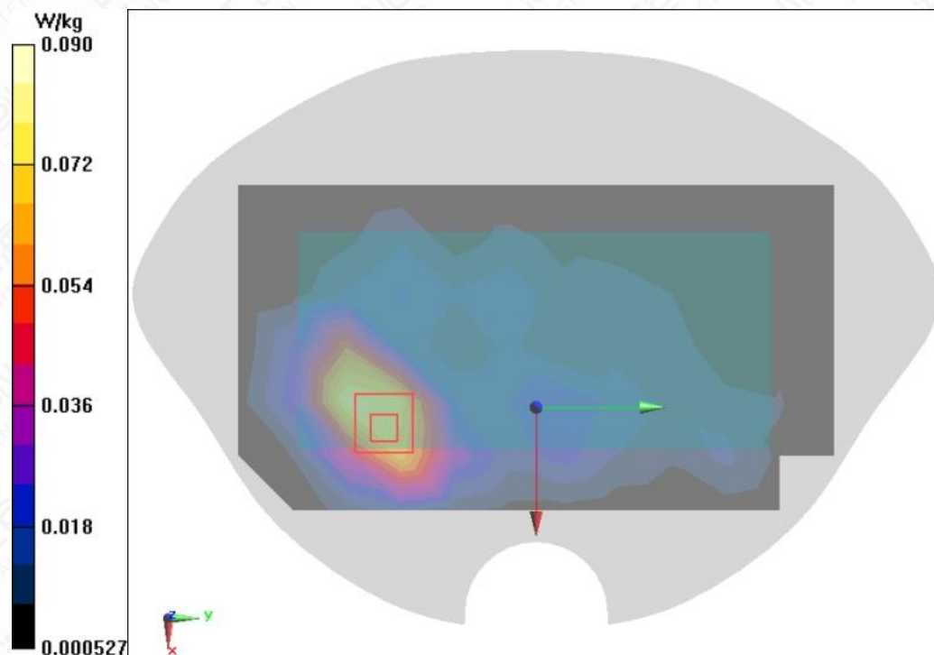
Figure A.1-74 BT DH5 Back Side Mode Low 10mm
