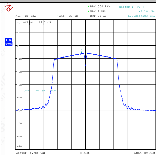
11AC40SISO-Ant1-5755-PASS
