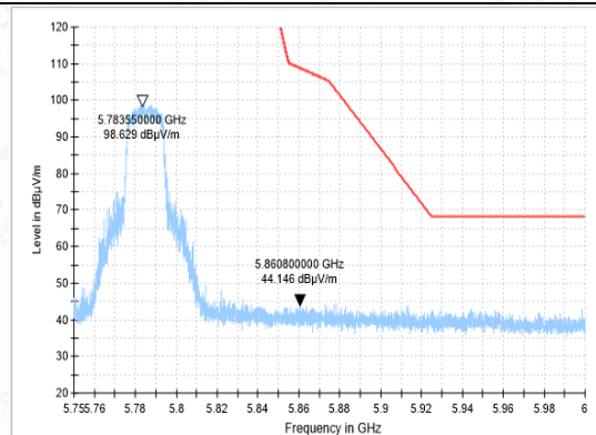
BANDEGE-11AC-CH157-PK
