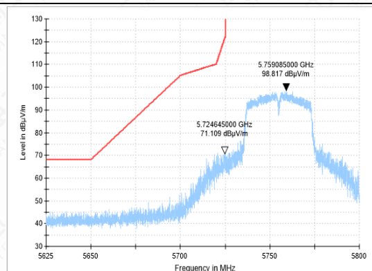
BANDEGE-11AC(40M)-CH151-PK
