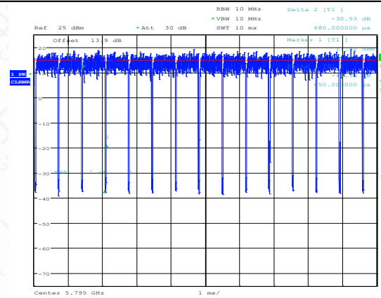
NTNV-11N40SISO-Ant1-5795
