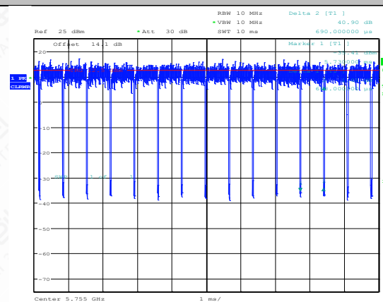
NTNV-11AC40SISO-Ant1-5755
