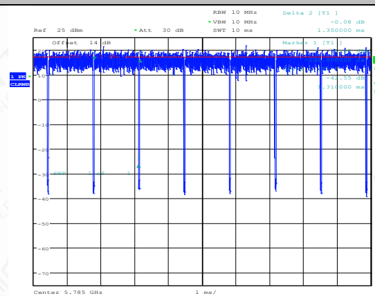
NTNV-11AC20SISO-Ant1-5785
