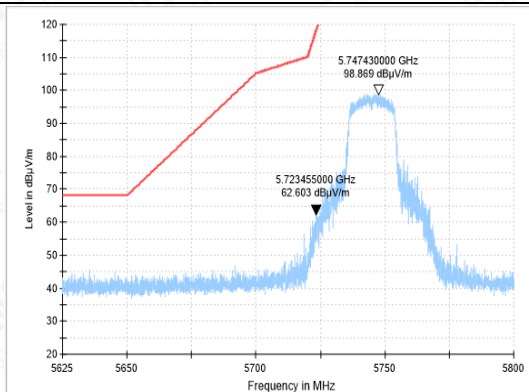
BANDEGE-11AC-CH149-PK
