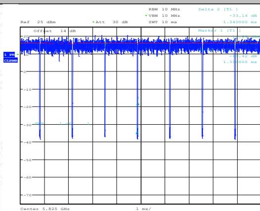
NTNV-11AC20SISO-Ant1-5825
