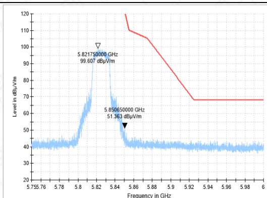
BANDEGE-11AC-CH165-PK
