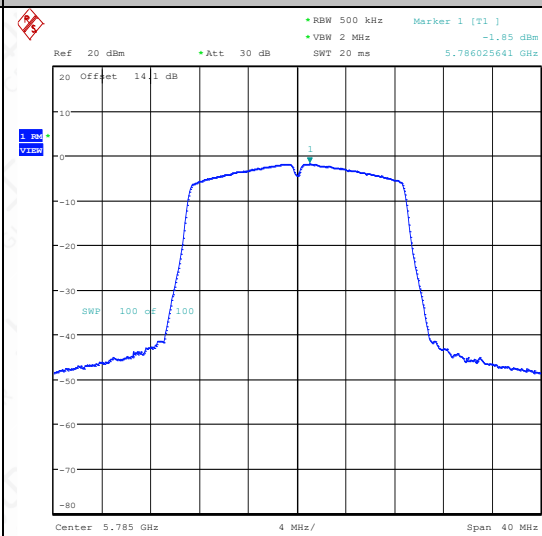
11AC20SISO-Ant1-5785-PASS
