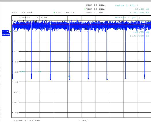
NTNV-11AC20SISO-Ant1-5745
