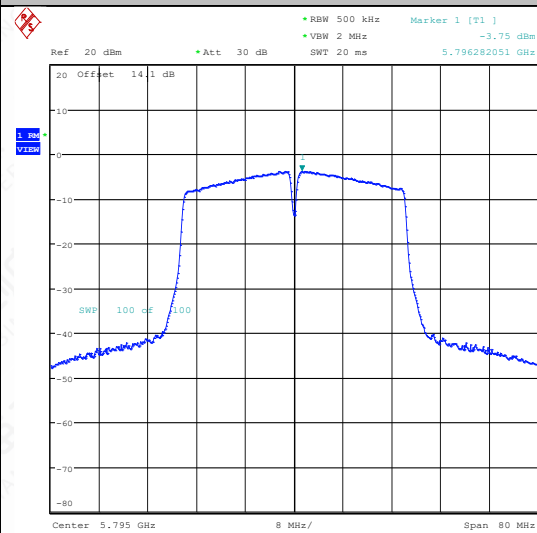
11N40SISO-Ant1-5795-PASS
