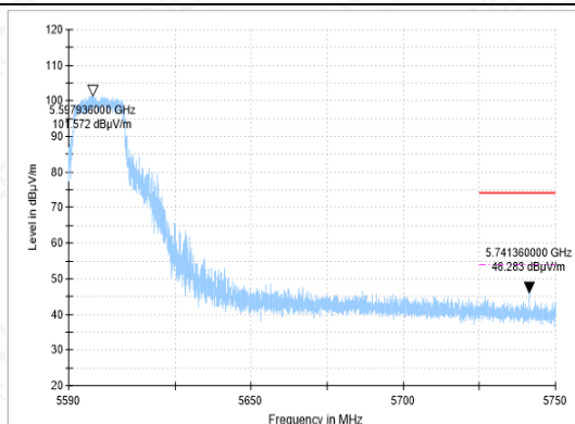
BANEDGE-11A-CH120-PK
