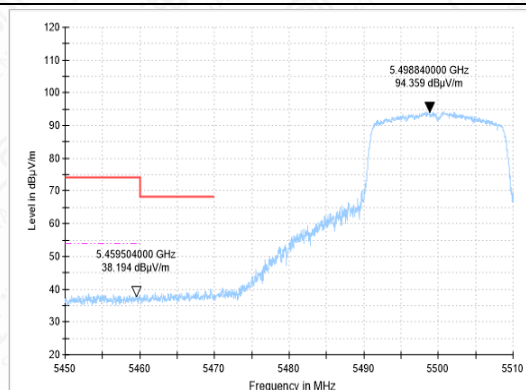
BANDEGE-11AC-CH100-AV
