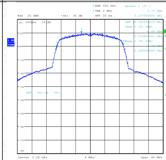
11N20SISO-Ant1-5280
