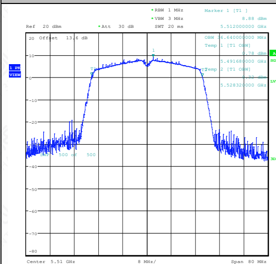
11AC40SISO-Ant1-5510
