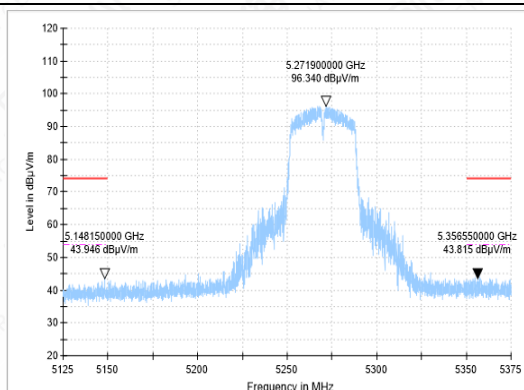
BANDEDGE-11AC(40M)-CH54-PK
