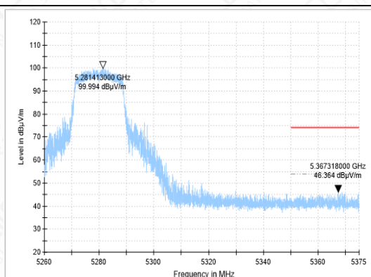
BANDEGE-11AC-CH56-PK
