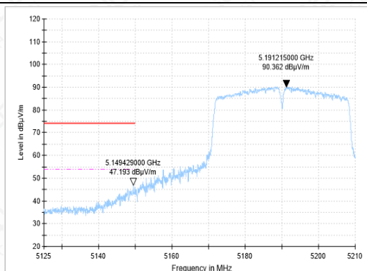
BANDEDGE-11AC(40M)-CH38-AV
