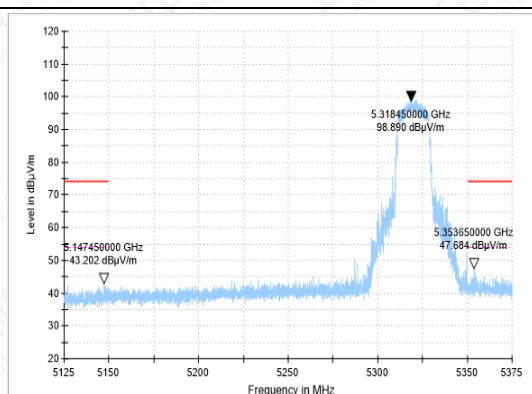
BANEDGE-11N-CH64-PK
