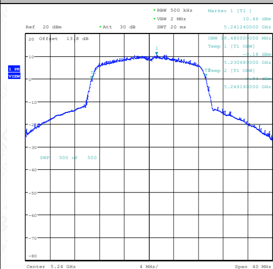
11N20SISO-Ant1-5240
