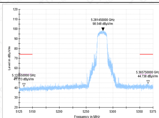
BANEDGE-11N-CH56-PK
