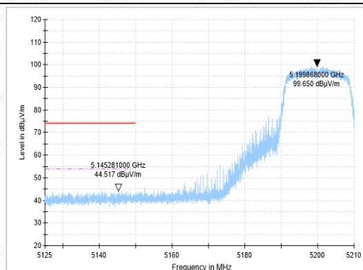
BANEDGE-11N-CH40-PK
