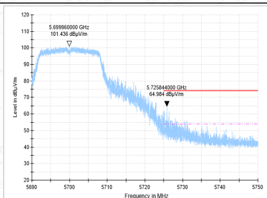
BANEDGE-11A-CH140-PK
