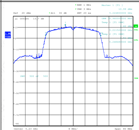
11N40SISO-Ant1-5230
