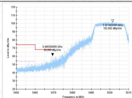
BANDEDGE-11A-CH100-PK
