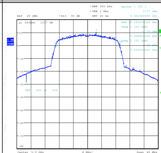
11N20SISO-Ant1-5500
