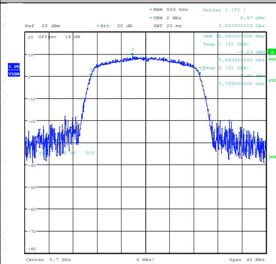
11AC20SISO-Ant1-5700
