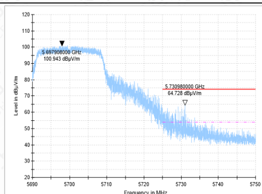
BANDEGE-11N-CH140-PK
