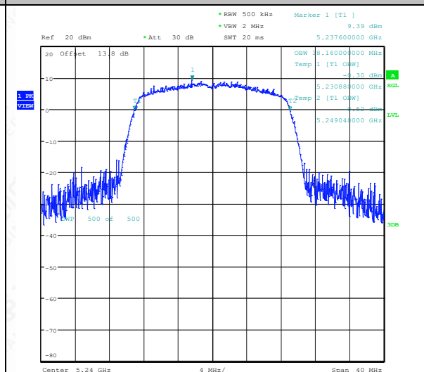
11AC20SISO-Ant1-5240
