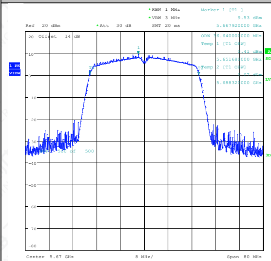
11AC40SISO-Ant1-5670
