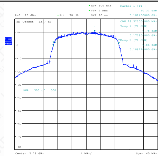
11N20SISO-Ant1-5180
