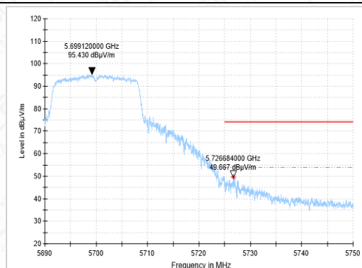
BANEDGE-11A-CH140-AV
