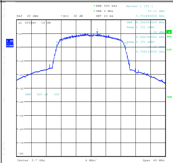
11N20SISO-Ant1-5700
