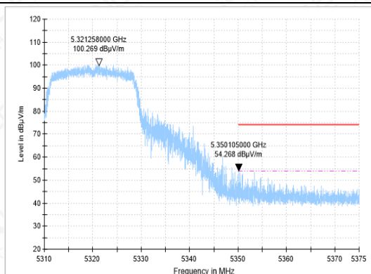
BANDEGE-11AC-CH64-PK
