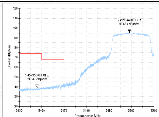
BANDEDGE-11A-CH100-AV
