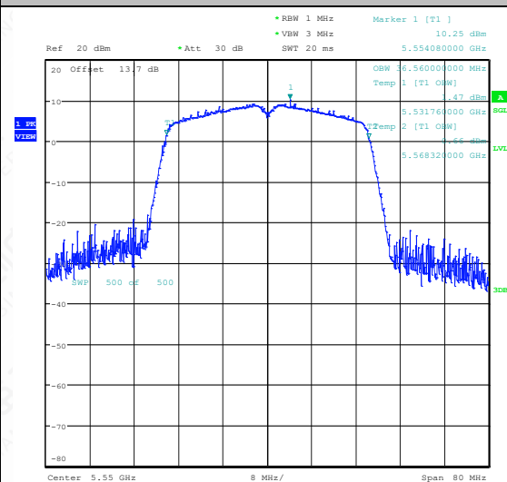
11AC40SISO-Ant1-5550
