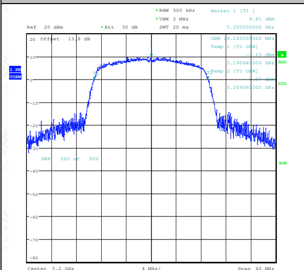
11AC20SISO-Ant1-5200
