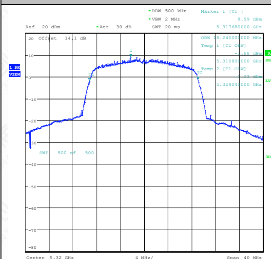
11N20SISO-Ant1-5320
