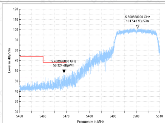
BANDEGE-11AC-CH100-PK
