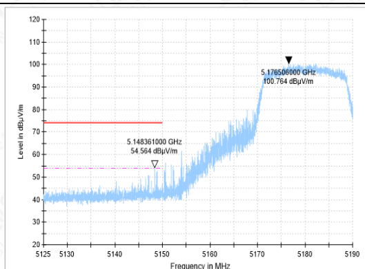
BANEDGE-11N-CH36-PK
