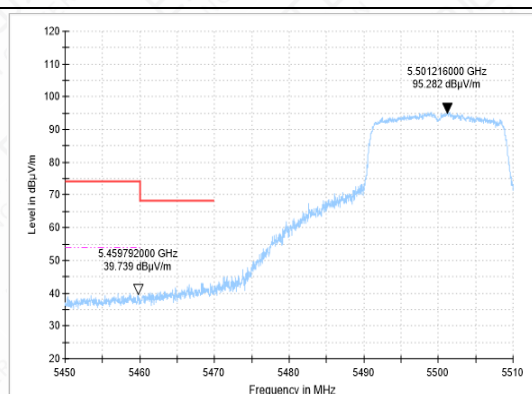
BANEDGE-11N-CH100-AV
