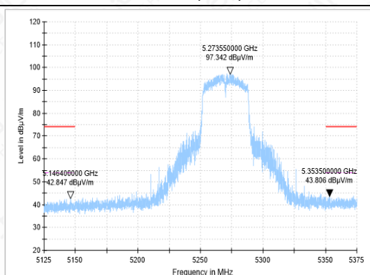
BANDEGE-11N(40M)-CH54-PK
