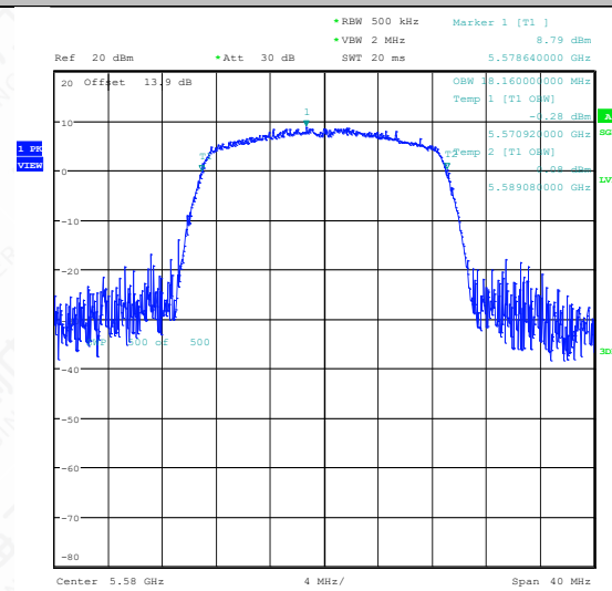
11AC20SISO-Ant1-5580
