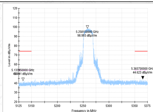
BANEDGE-11N-CH52-PK
