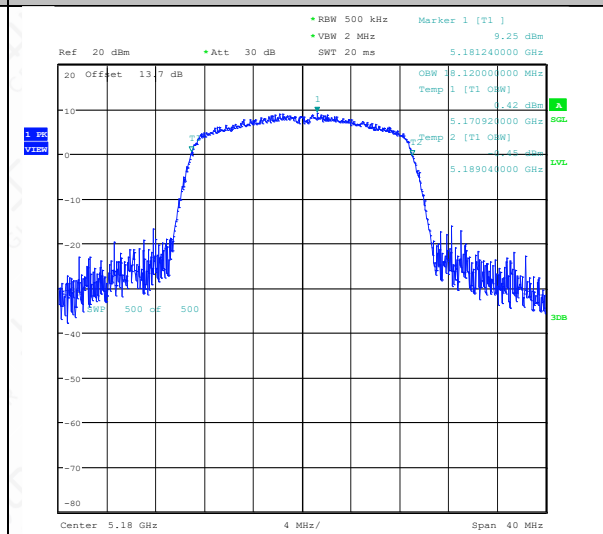
11AC20SISO-Ant1-5180
