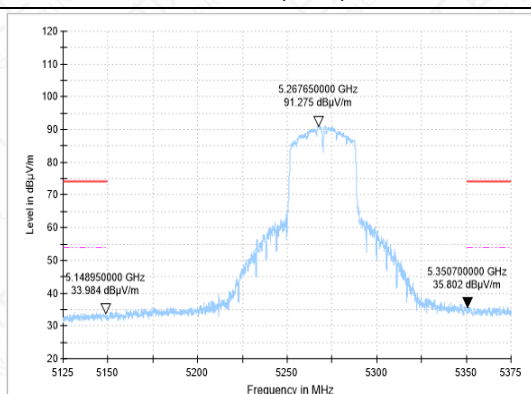
BANDEGE-11N(40M)-CH54-AV
