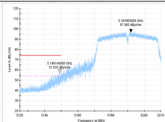
BANDEDGE-11AC(40M)-CH38-PK
