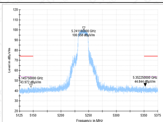
BANDEGE-11AC-CH48-PK
