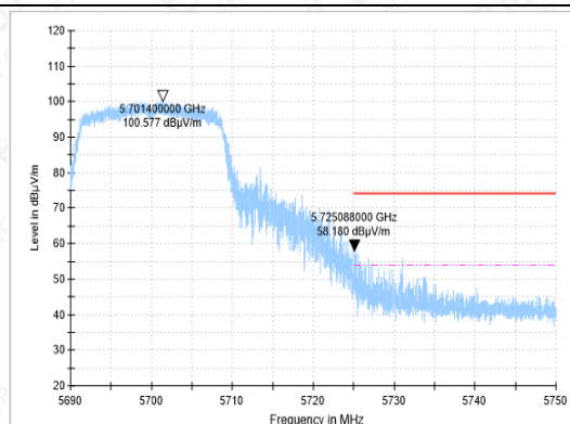
BANDEGE-11AC-CH140-PK
