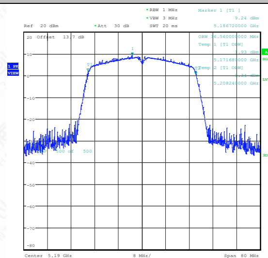
11AC40SISO-Ant1-5190
