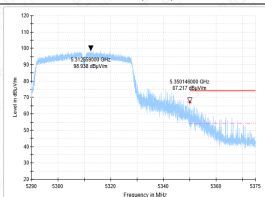
BANDEGE-11N(40M)-CH62-PK
