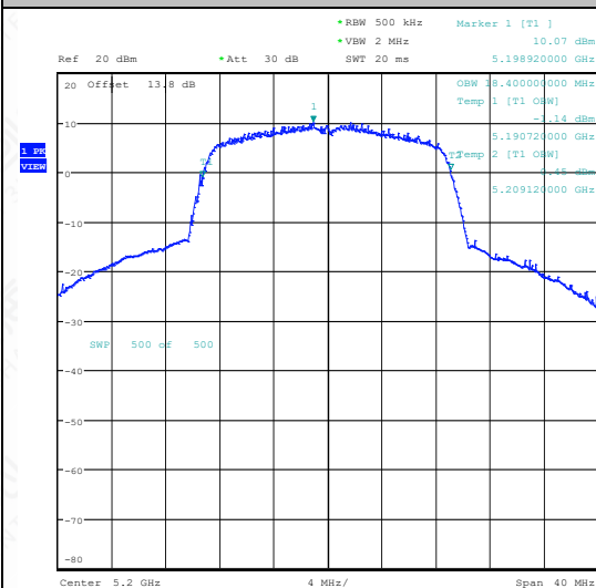
11N20SISO-Ant1-5200
