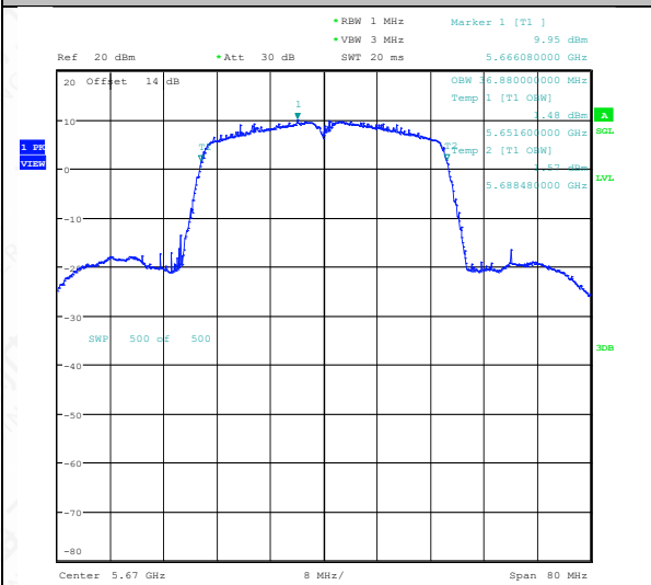
11N40SISO-Ant1-5670
