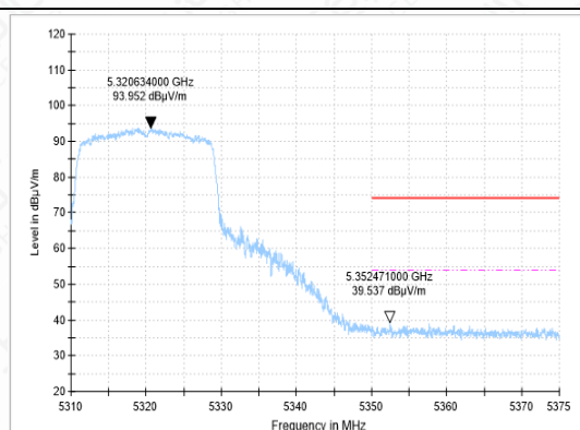
BANEDGE-11N-CH64-AV
