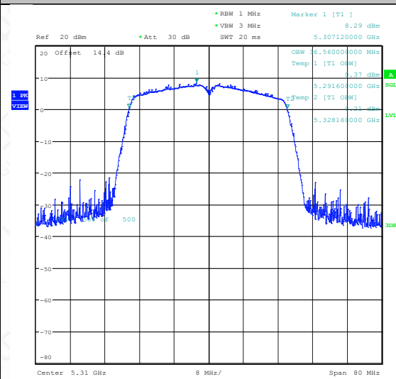
11AC40SISO-Ant1-5310
