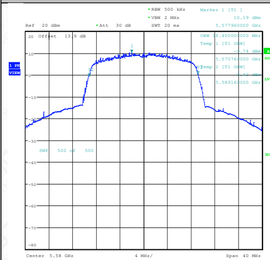
11N20SISO-Ant1-5580
