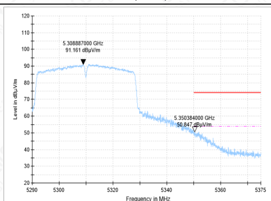
BANDEGE-11N(40M)-CH62-AV-17
