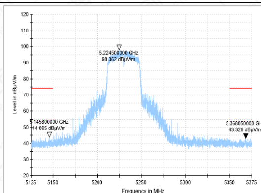
BANDEGE-11N(40M)-CH46-PK
