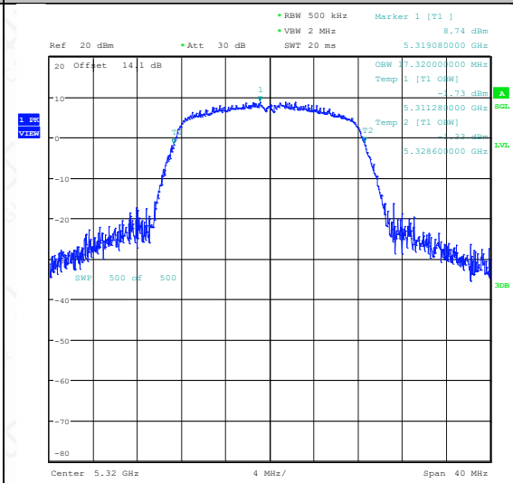
11A-Ant1-5320
