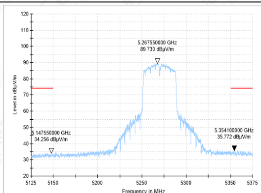
BANDEDGE-11AC(40M)-CH54-AV
