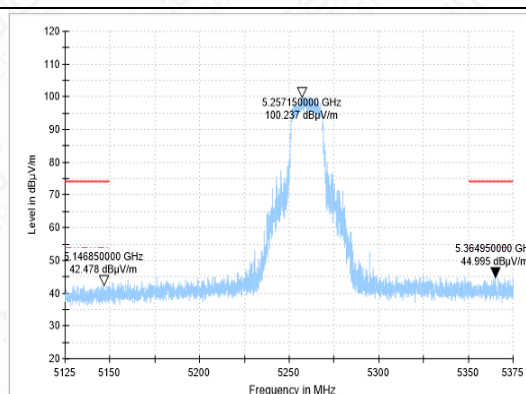
BANDEGE-11AC-CH52-PK
