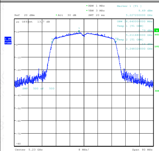
11AC40SISO-Ant1-5230
