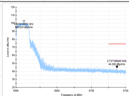
BANDEGE-11AC-CH120-PK
