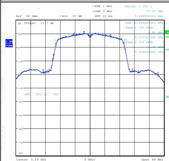
11N40SISO-Ant1-5190
