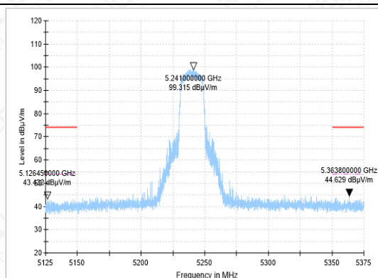
BANEDGE-11N-CH48-PK
