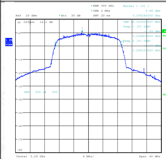
11N20SISO-Ant1-5260
