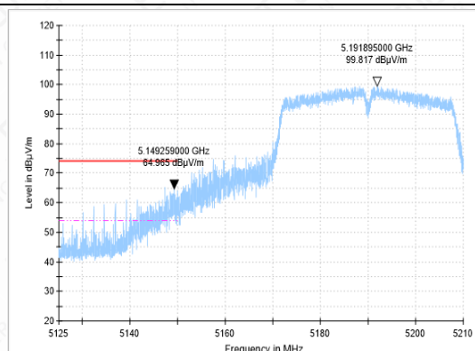
BANDEGE-11N(40M)-CH38-PK
