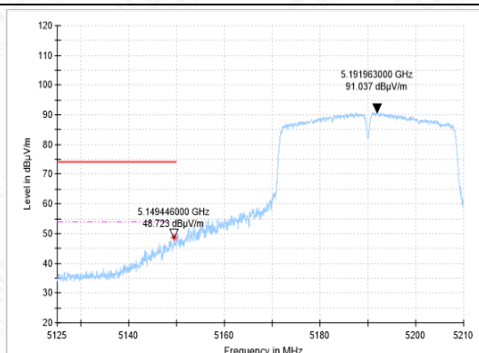
BANDEGE-11N(40M)-CH38-AV-16
