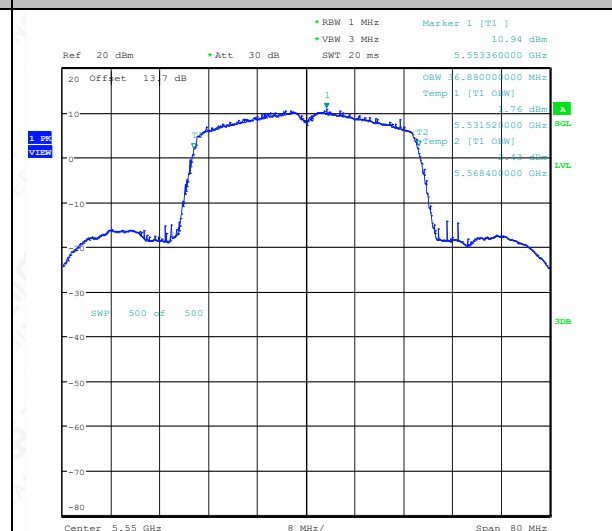
11N40SISO-Ant1-5550
