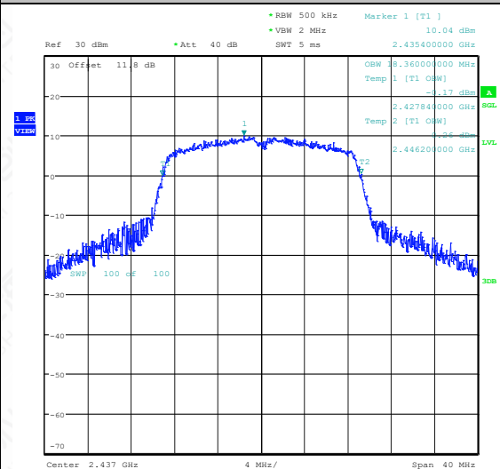
11N20SISO-Ant1-2437
