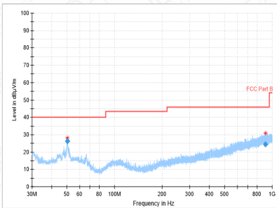
RSE-11G-CH6-30MHz-1GHz
