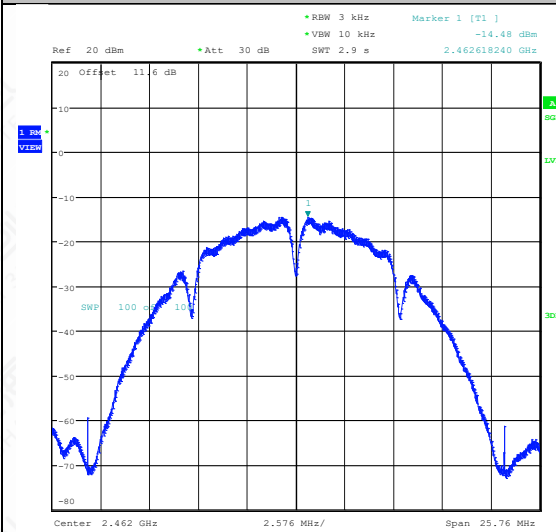
11B-Ant1-2462-PASS
