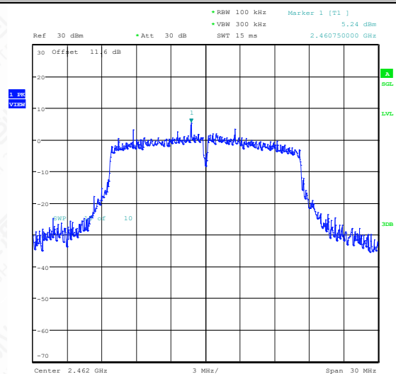
11G-Ant1-2462-0~Reference-PASS
