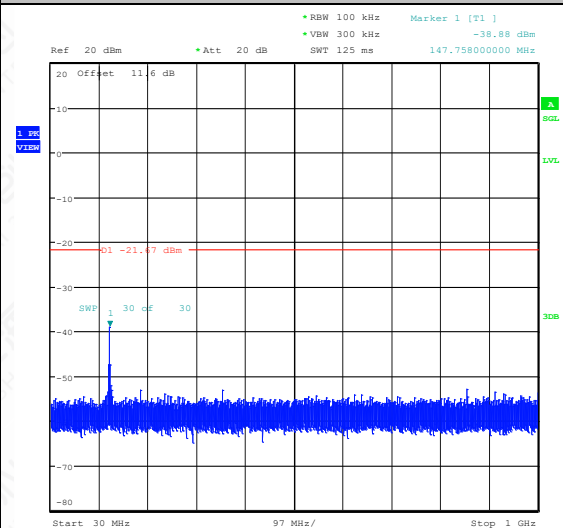
11B-Ant1-2462-30~1000-PASS
