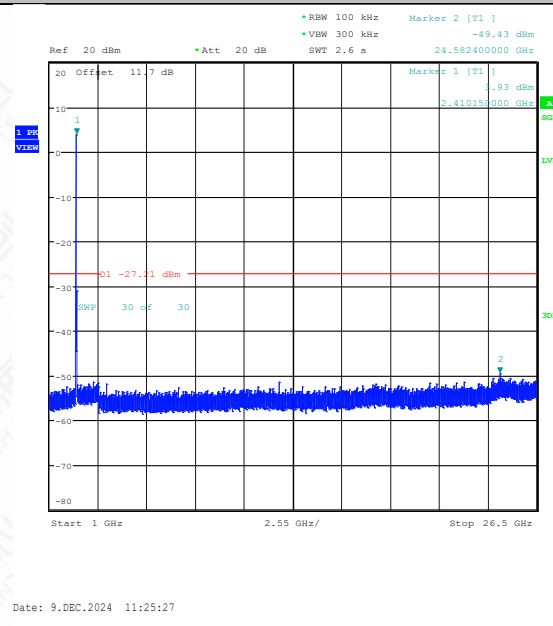
11N20SISO-Ant1-2412-1000~26500-PASS
