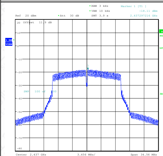
11G-Ant1-2437-PASS
