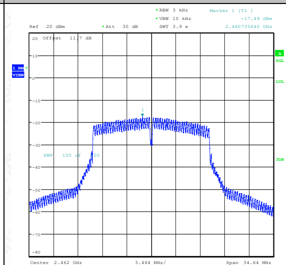
11G-Ant1-2462-PASS
