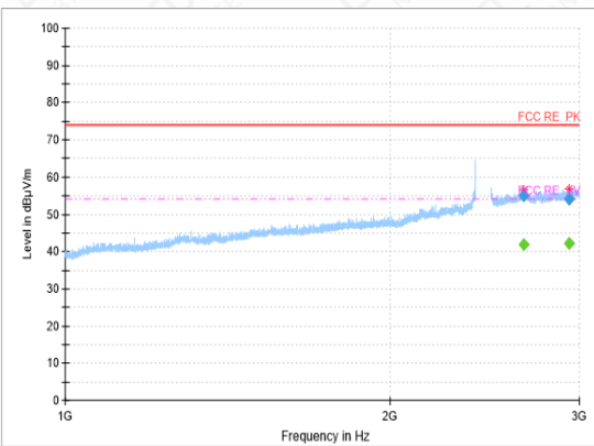
RSE-11G-CH6-1GHz-3GHz
