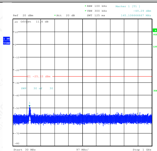
11N20SISO-Ant1-2462-30~1000-PASS
