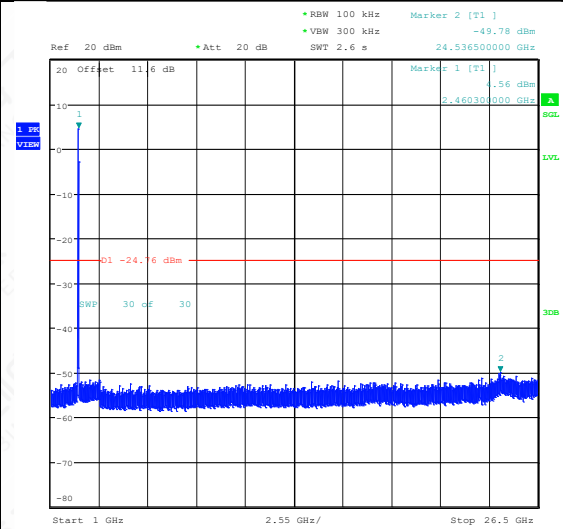
11G-Ant1-2462-1000~26500-PASS
