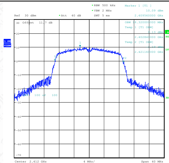
11N20SISO-Ant1-2412
