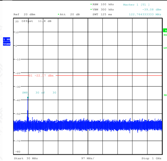
11B-Ant1-2437-30~1000-PASS
