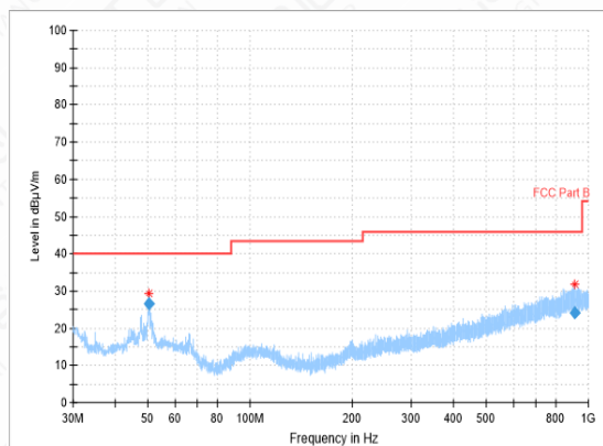
RSE-11G-CH1-30MHz-1GHz
