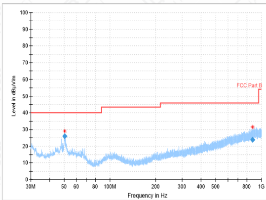
RSE-11N-CH1-30MHz-1GHz
