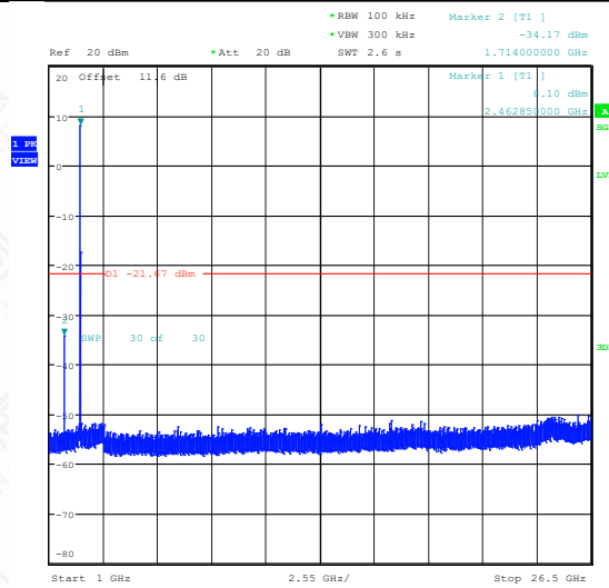
11B-Ant1-2462-1000~26500-PASS
