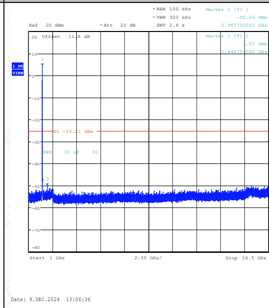
11N20SISO-Ant1-2437-1000~26500-PASS
