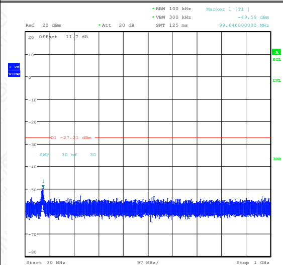
11N20SISO-Ant1-2412-30~1000-PASS
