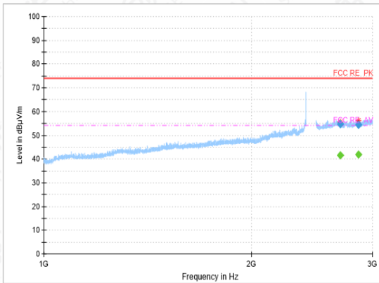
RSE-11B-CH6-1GHz-3GHz
