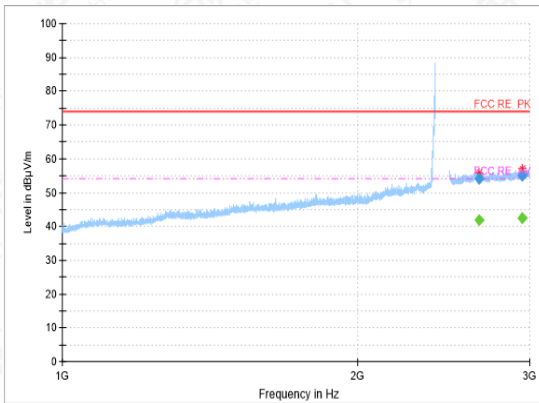
RSE-11G-CH1-1GHz-3GHz
