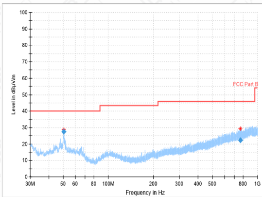
RSE-11B-CH11-30MHz-1GHz
