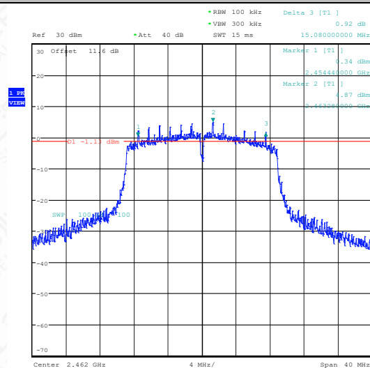
11N20SISO-Ant1-2462-PASS
