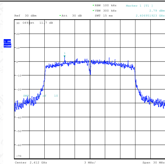
11N20SISO-Ant1-2412-0~Reference-PASS
