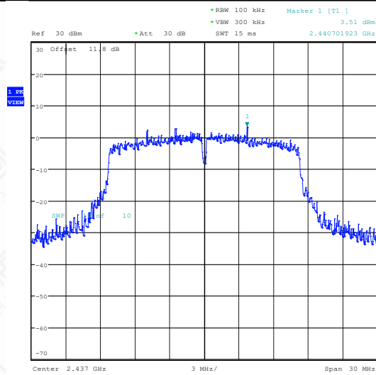
11G-Ant1-2437-0~Reference-PASS
