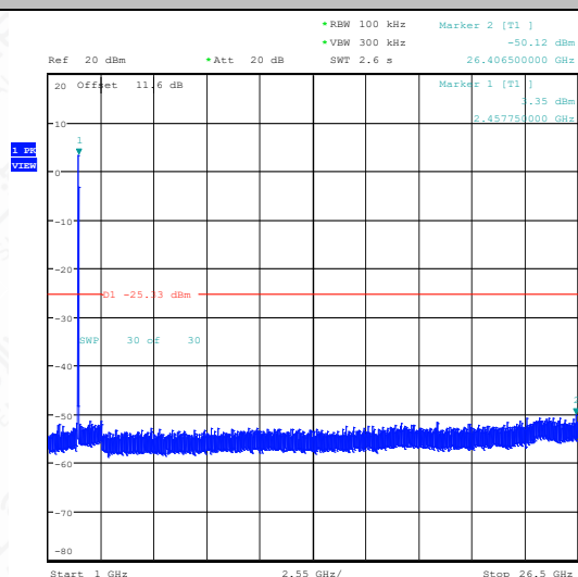
11N20SISO-Ant1-2462-1000~26500-PASS
