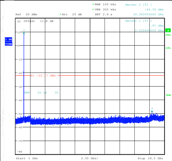
11B-Ant1-2437-1000~26500-PASS
