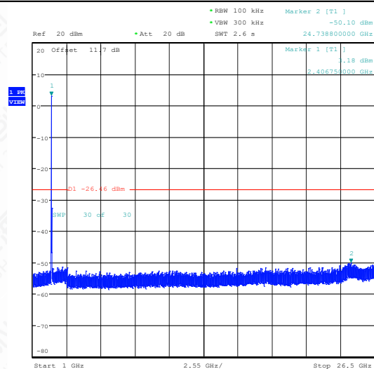
11G-Ant1-2412-1000~26500-PASS
