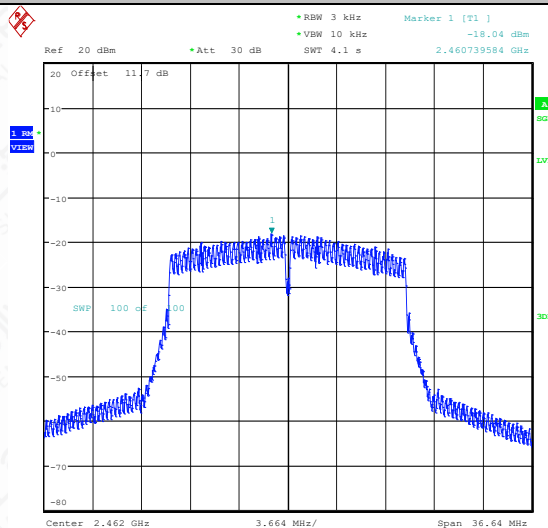
11N20SISO-Ant1-2462-PASS
