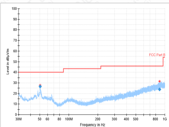
RSE-11G-CH11-30MHz-1GHz
