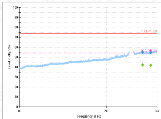
RSE-11B-CH11-1GHz-3GHz
