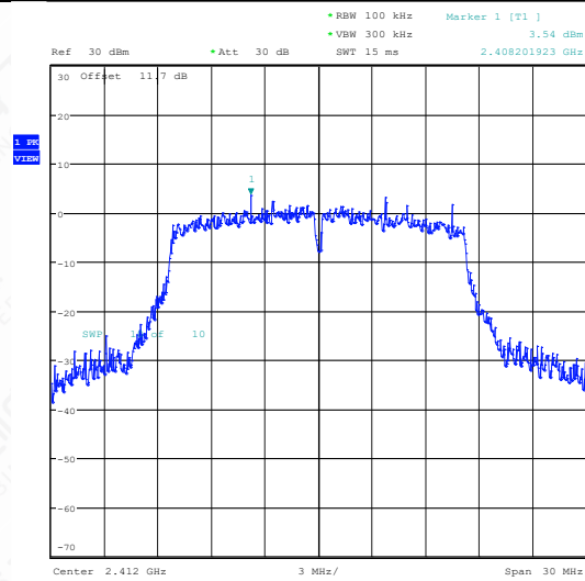
11G-Ant1-2412-0~Reference-PASS
