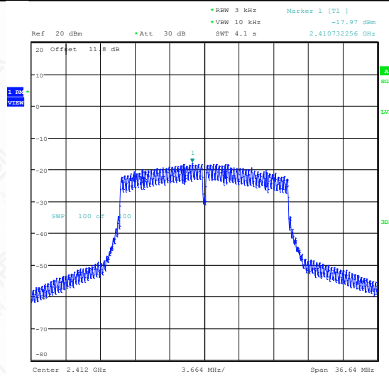
11N20SISO-Ant1-2412-PASS
