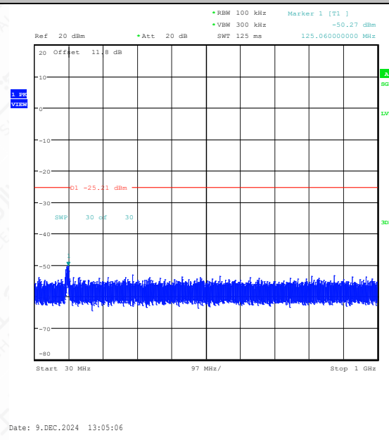
11N20SISO-Ant1-2437-30~1000-PASS
