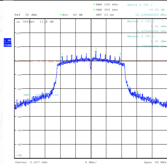
11N20SISO-Ant1-2437-PASS
