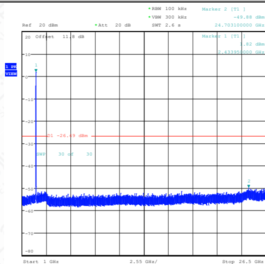
11G-Ant1-2437-1000~26500-PASS
