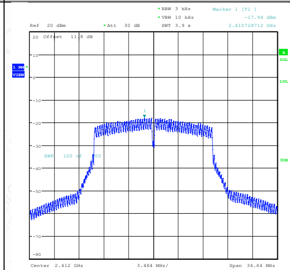
11G-Ant1-2412-PASS
