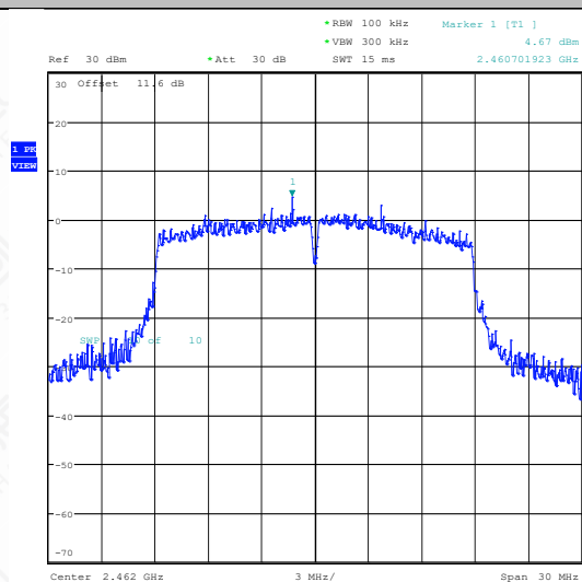
11N20SISO-Ant1-2462-0~Reference-PASS
