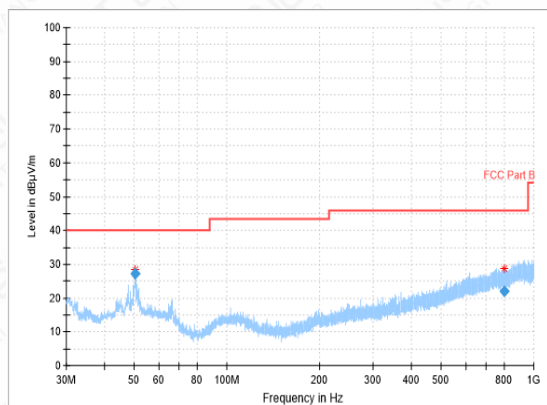
RSE-11N-CH6-30MHz-1GHz
