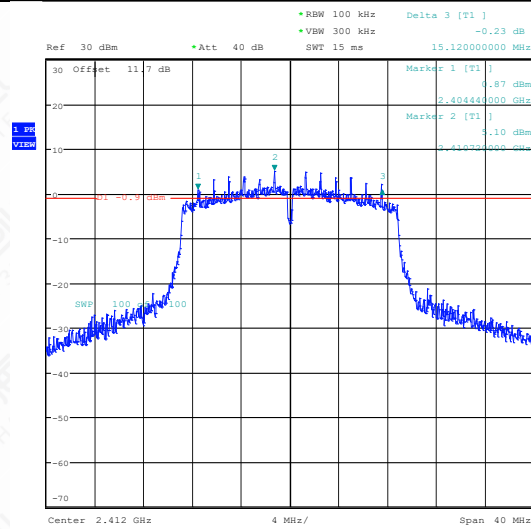
11N20SISO-Ant1-2412-PASS
