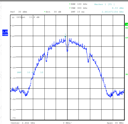
11B-Ant1-2462-0~Reference-PASS
