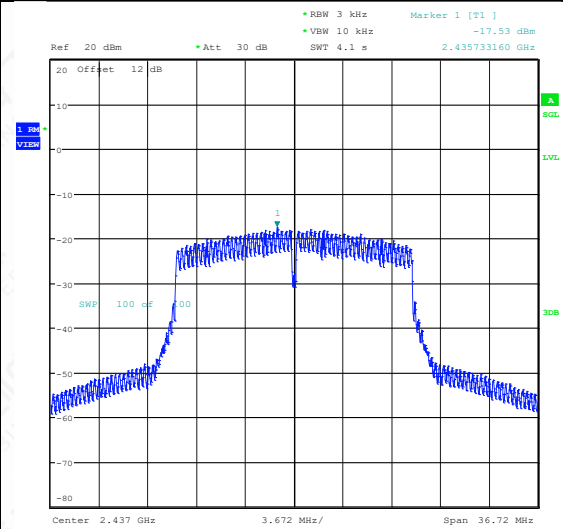
11N20SISO-Ant1-2437-PASS
