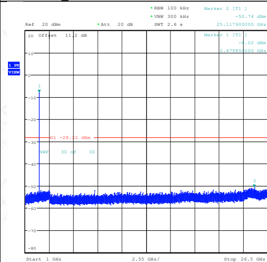
BLE_500K-Ant1-2480-1000~26500-PASS
