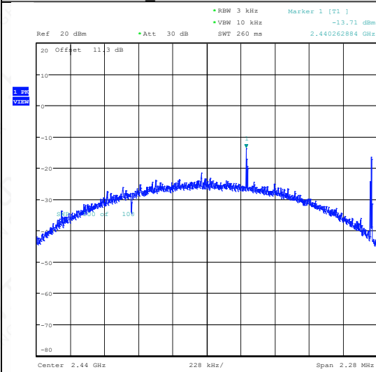
BLE_2M-Ant1-2440-PASS
