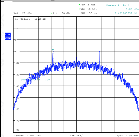
BLE_125K-Ant1-2402-PASS
