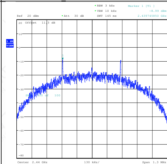
BLE_125K-Ant1-2440-PASS
