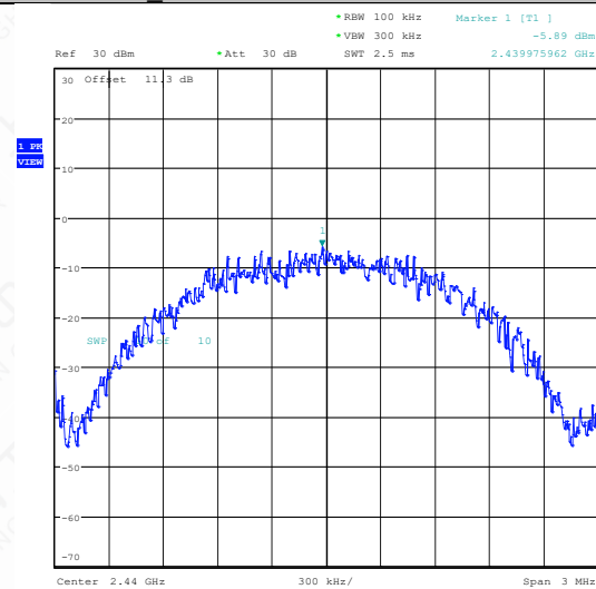
BLE_2M-Ant1-2440-0~Reference-PASS
