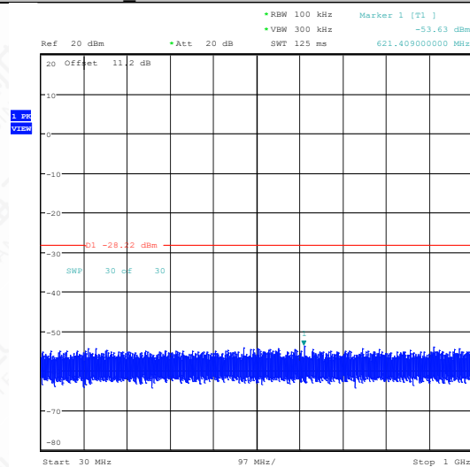
BLE_500K-Ant1-2480-30~1000-PASS
