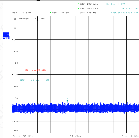
BLE_125K-Ant1-2480-30~1000-PASS
