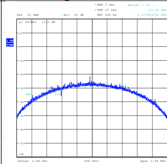
BLE_2M-Ant1-2480-PASS
