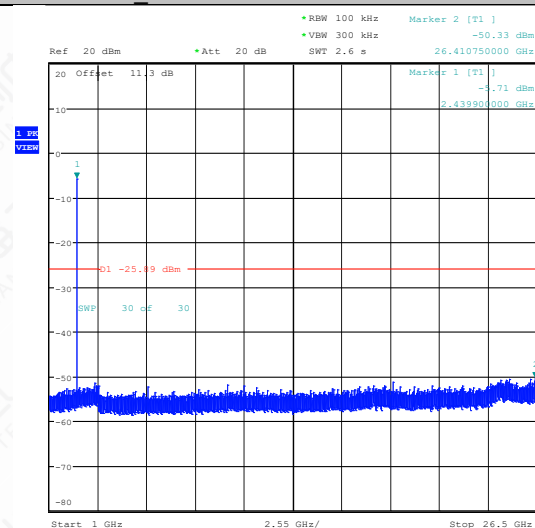
BLE_2M-Ant1-2440-1000~26500-PASS
