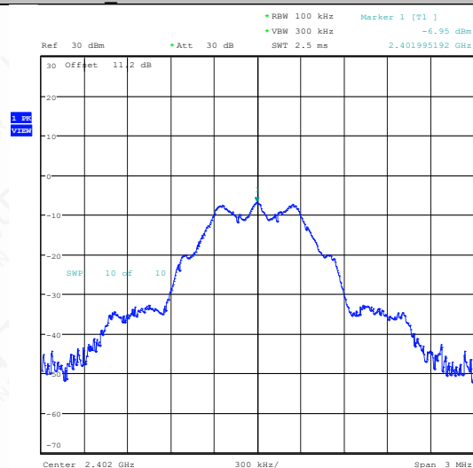
BLE_500K-Ant1-2402-0~Reference-PASS
