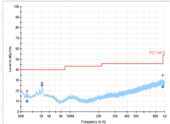
RSE-2DH5-CH0-30MHz-1GHz
