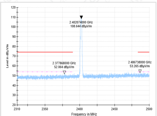
BANDEGE-3DH5-CH0-PK
