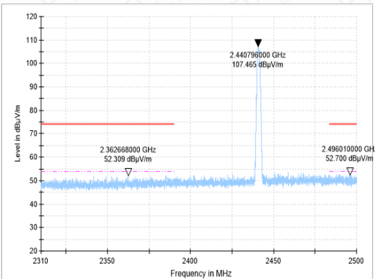
BANDEGE-2DH5-CH39-PK
