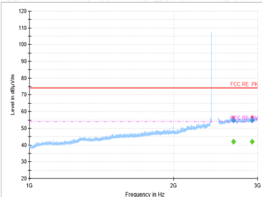
RSE-2DH5-CH0-1GHz-3GHz
