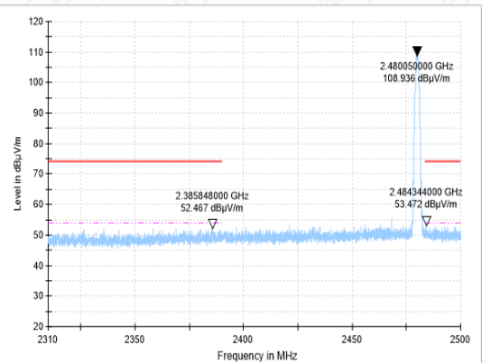
BANDEGE-2DH5-CH78-PK
