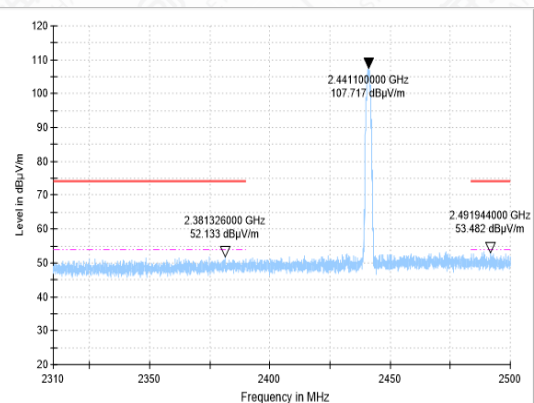
BANDEGE-3DH5-CH39-PK
