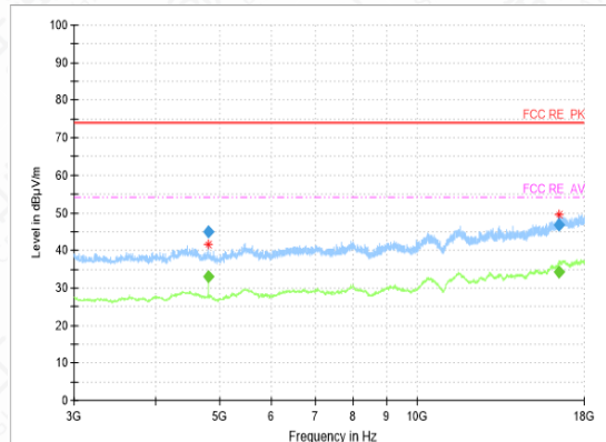
RSE-2DH5-CH0-3GHz-18GHz
