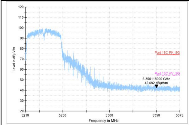
Peak detector
