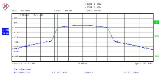
Output Power-Conducted (802.11n-HT20, Ch40)
