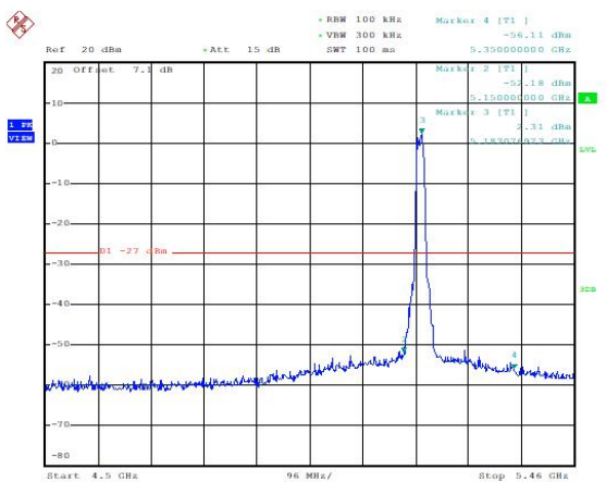
Band Edges (802.11ac-VHT20), 5180MHz
