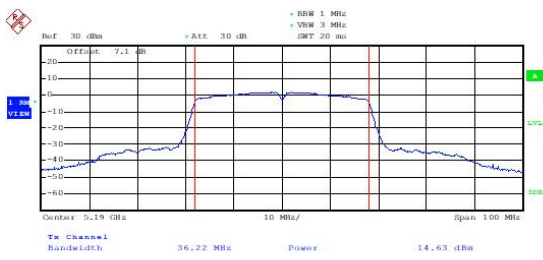
Output Power-Conducted (802.11n-HT40, Ch38)
