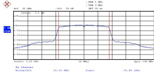
Output Power-Conducted (802.11n-HT40, Ch46)
