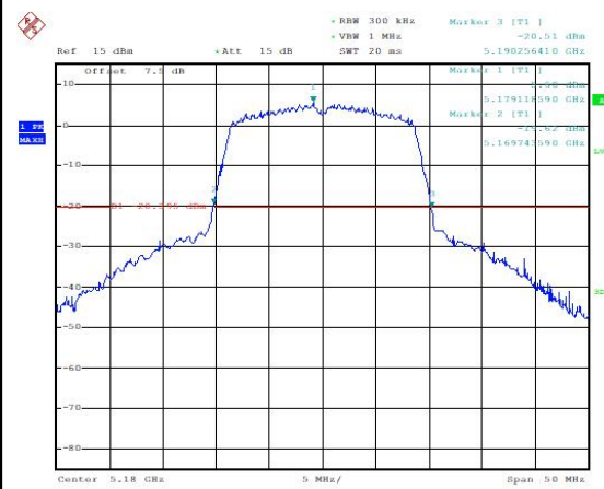
Occupied 26dB Bandwidth (MHz) (802.11n-HT20, 5180MHz)
