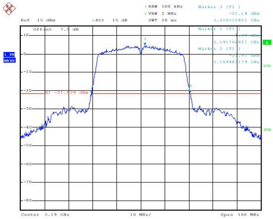
Occupied 26dB Bandwidth (MHz) (802.11n-HT40, 5190MHz)
