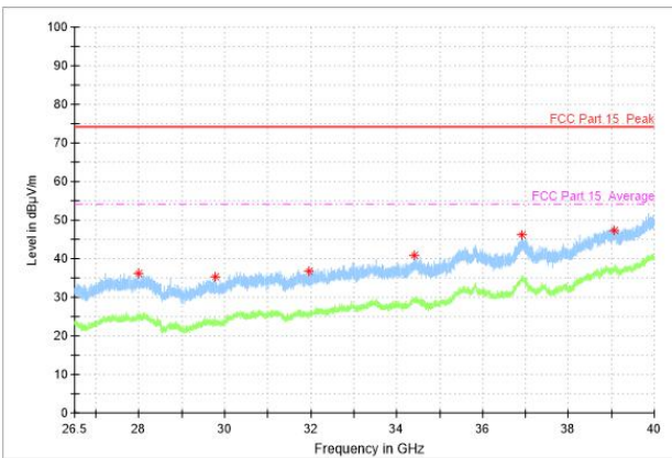
Radiated Spurious Emission (802.11n-HT20, ch48, 26.5 GHz-40 GHz)
