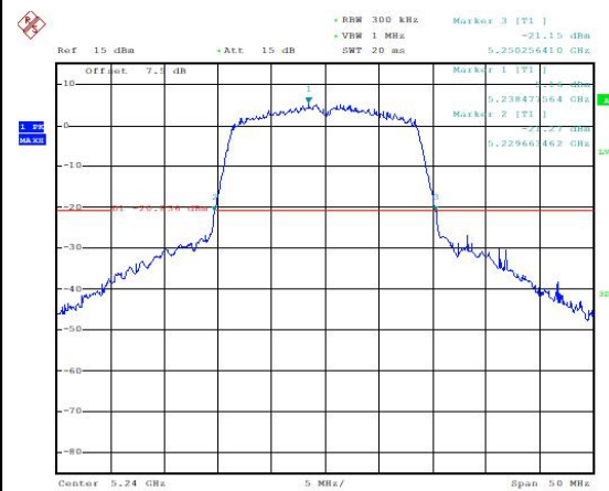
Occupied 26dB Bandwidth (MHz) (802.11n-HT20, 5240MHz)
