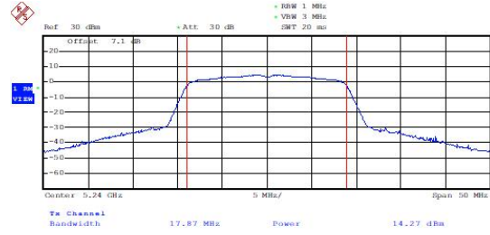
Output Power-Conducted (802.11n-HT20, Ch48)
