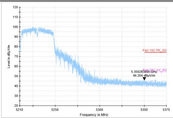
Peak detector
