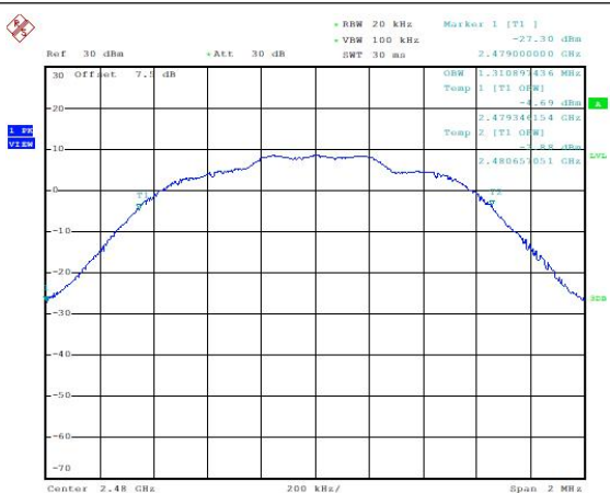
99% Bandwidth: 8DPSK, Ch78
