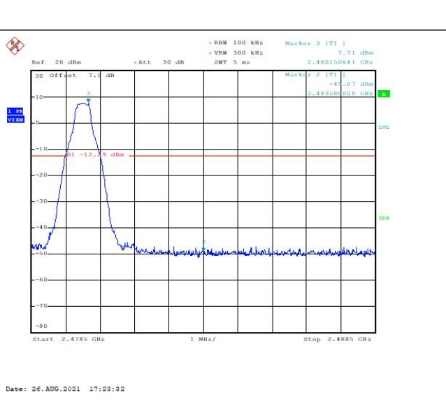
Frequency Band Edge: GFSK, Ch78, Hopping OFF
