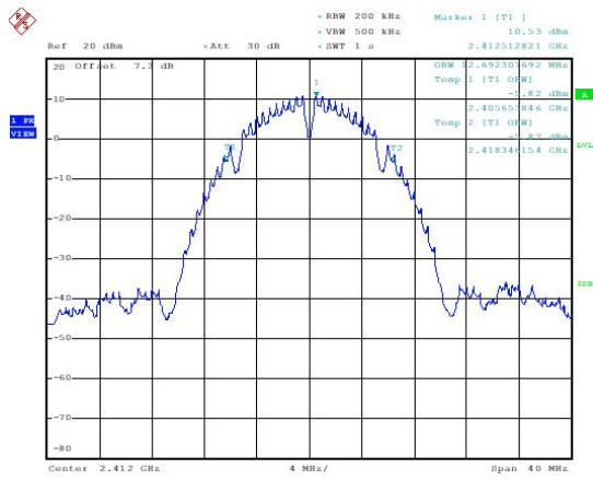
99% Occupied Bandwidth (802.11b, Ch1)
