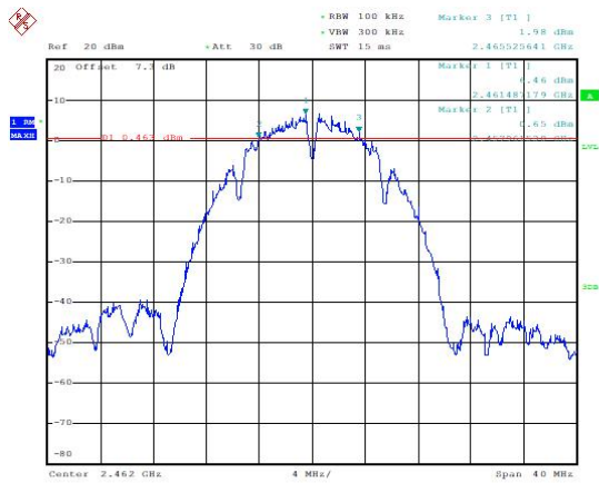
Occupied 6dB Bandwidth (MHz) (802.11b, Ch11)
