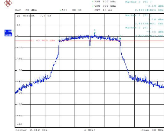
Occupied 6dB Bandwidth (MHz) (802.11g, Ch1)
