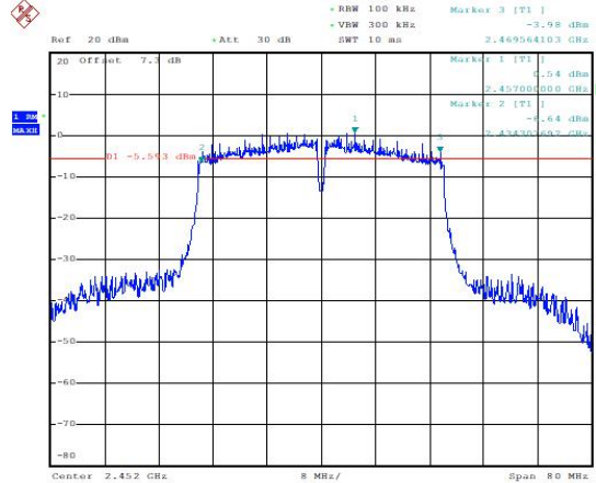
Occupied 6dB Bandwidth (MHz) (802.11n-40MHz, Ch9)
