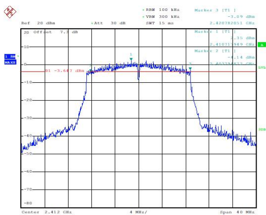
Occupied 6dB Bandwidth (MHz) (802.11n-20MHz, Ch1)
