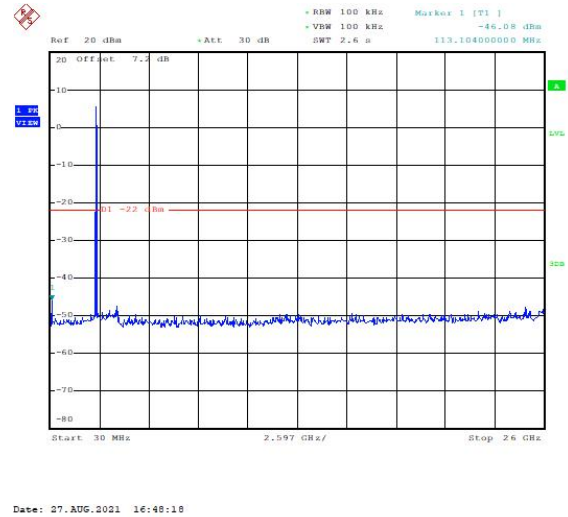
Conducted Spurious Emission (802.11b, Ch6, 30MHz~26GHz)
