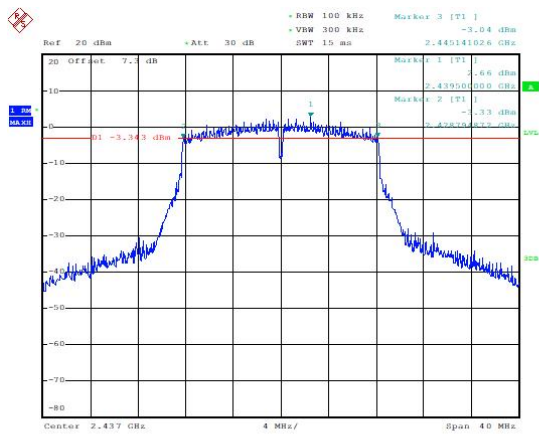
Occupied 6dB Bandwidth (MHz) (802.11g, Ch6)
