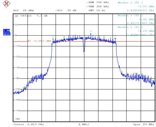
Occupied 6dB Bandwidth (MHz) (802.11n-40MHz, Ch3)
