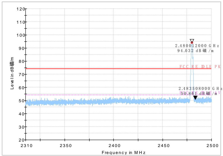
Fig.25 Bandedge:ch39
