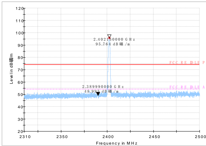
Fig.21 Bandedge:ch0
