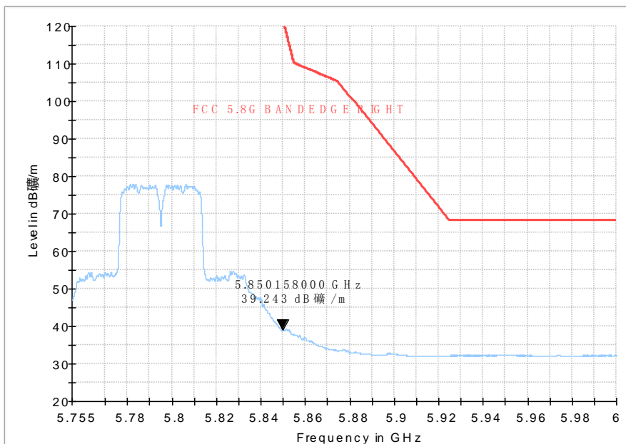
Average Fig. 47 Band Edges (802.11n-HT40, 5795MHz)
