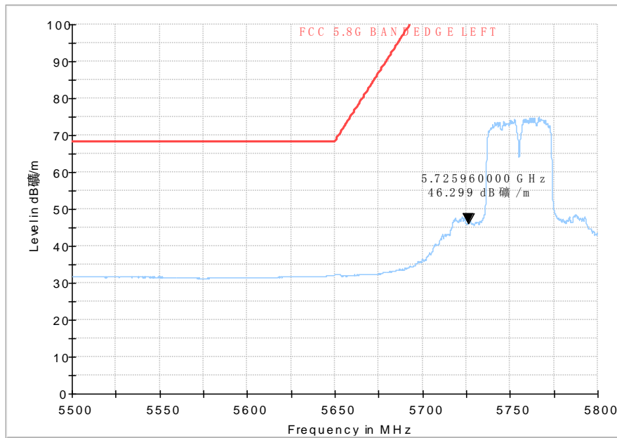
Average Fig. 46 Band Edges (802.11n-HT40, 5755MHz)
