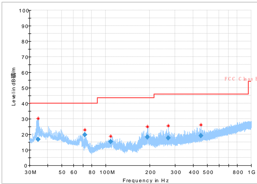
Fig. 31 Radiated Spurious Emission (802.11n-HT20, Ch149, 30 MHz-1 GHz)
