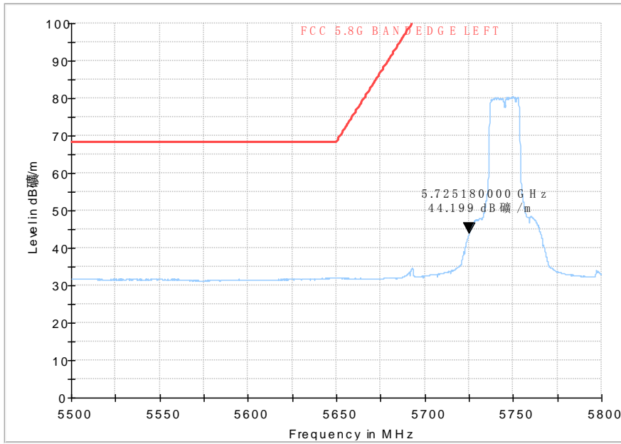
Average Fig. 42 Band Edges (802.11a, 5745MHz)
