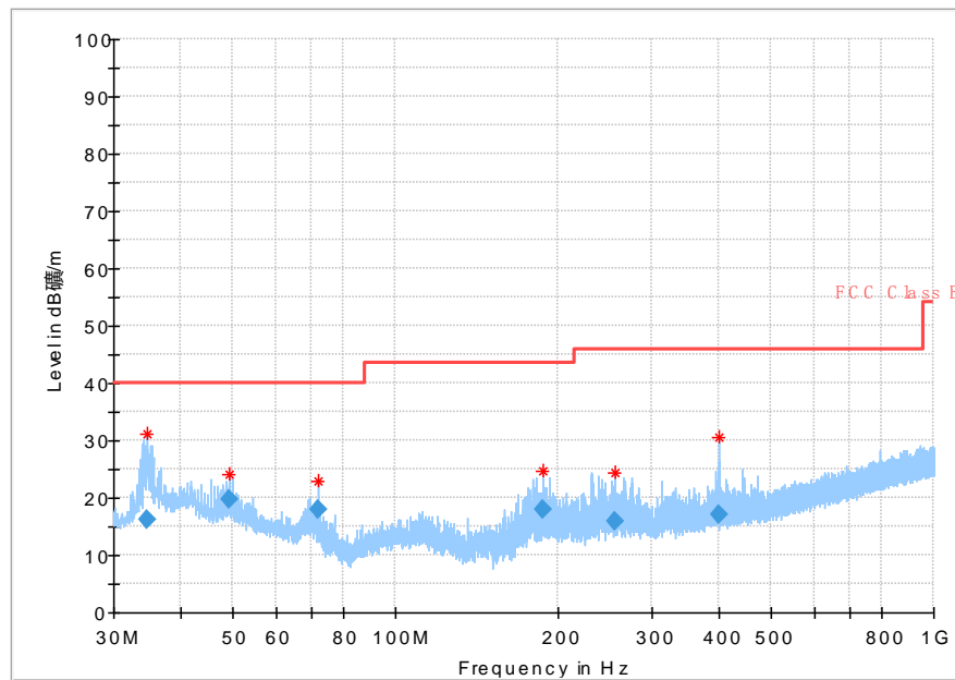
Fig. 34 Radiated Spurious Emission (802.11n-HT20, ch36, 30 MHz-1 GHz)
