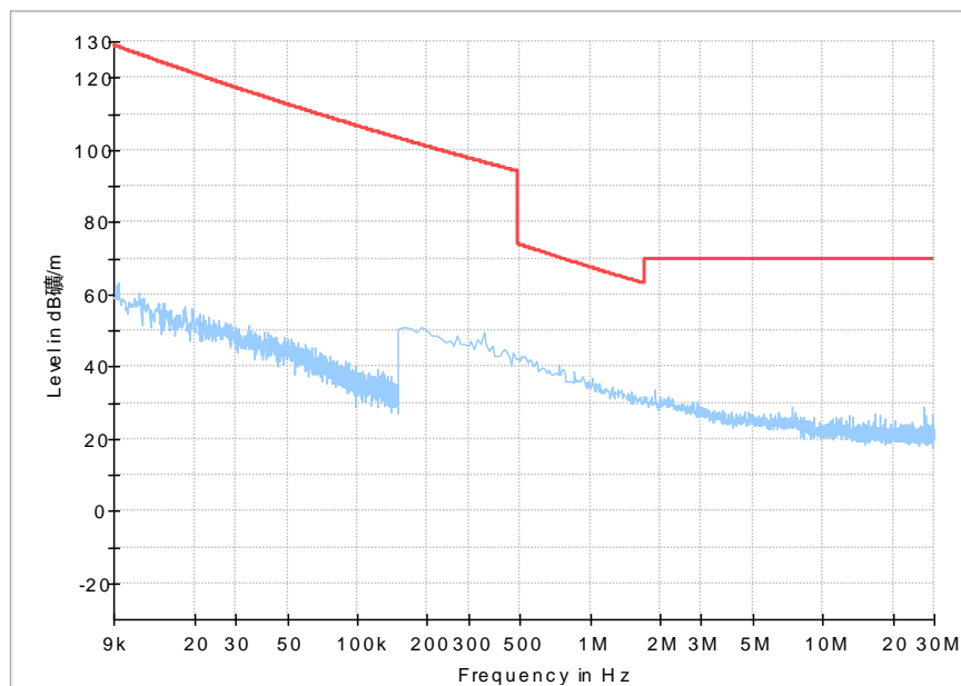
Fig. 44 Radiated Spurious Emission (9kHz-30MHz)
