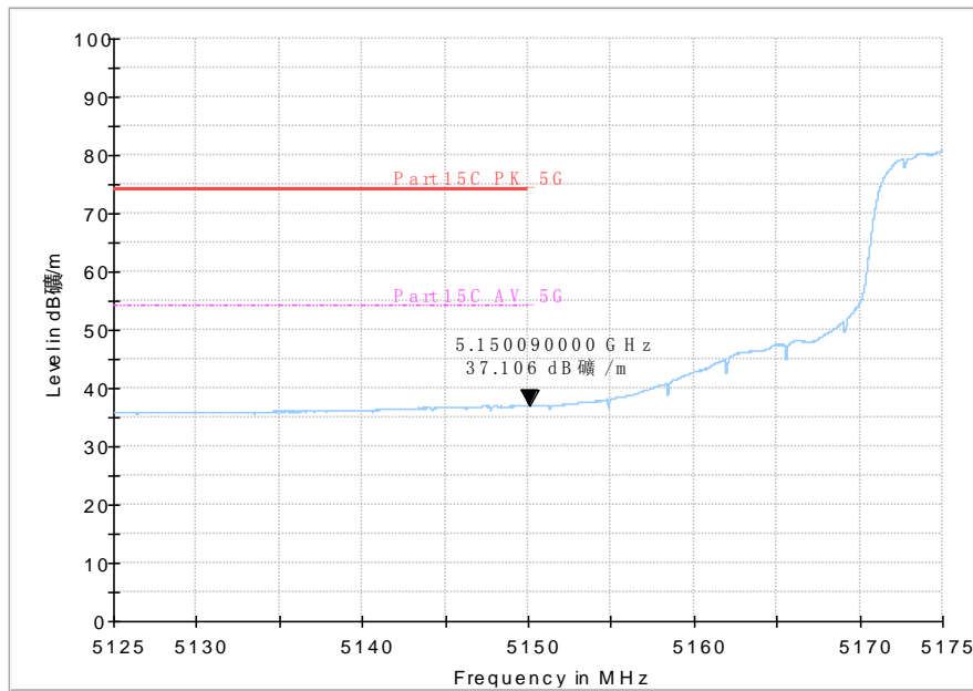
Average Fig. 27 Band Edges (802.11n-HT40, 5190MHz)
