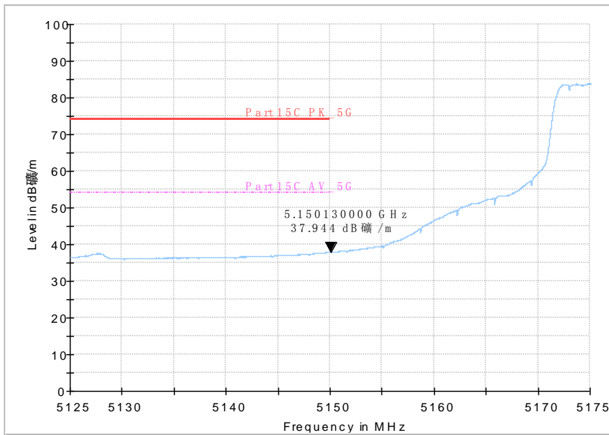
Average Fig. 23 Band Edges (802.11a, 5180MHz)
