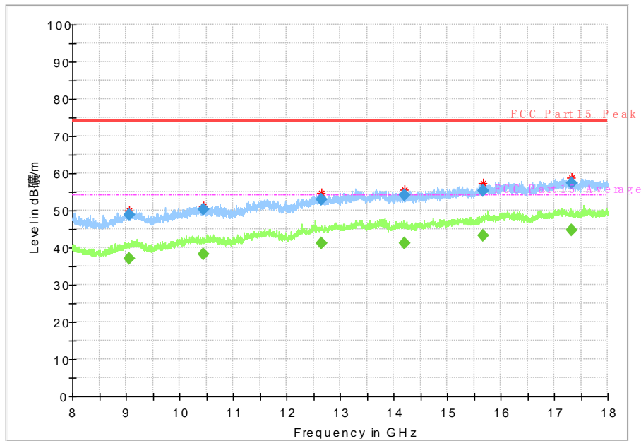
Fig. 31 Radiated Spurious Emission (802.11a, ch36, 8 GHz-18 GHz)
