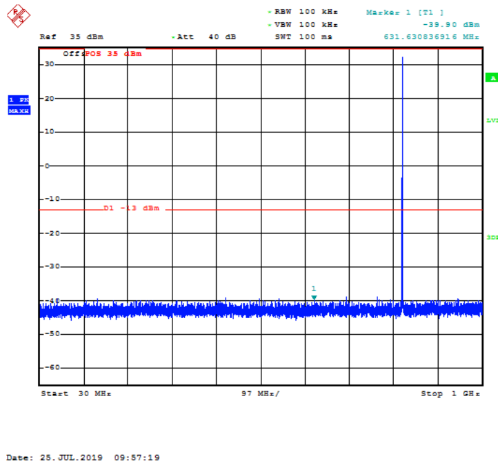
Fig.73 Channel 128: 30MHz~1GHz
