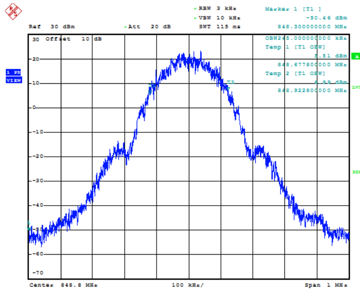
Fig.5 Channel 189-Occupied Bandwidth (99%)
