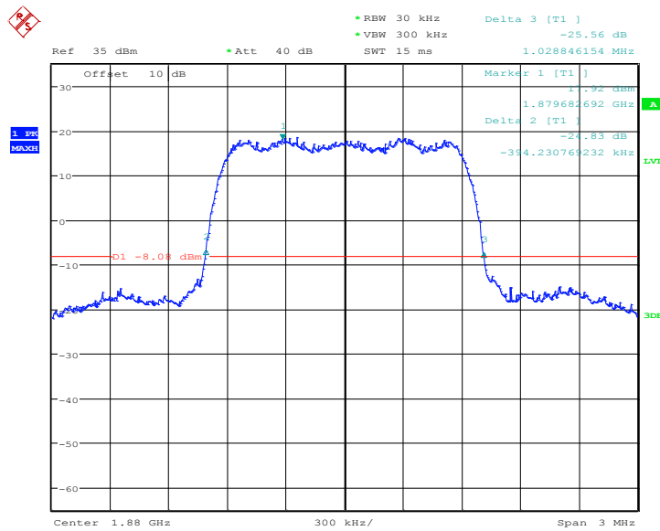
Fig.10 Channel 25- Emission Bandwidth (-26dBc BW)
