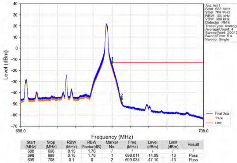
Band71_10MHz_64QAM_HCH_693MHz_RB_1_49_NTNV
