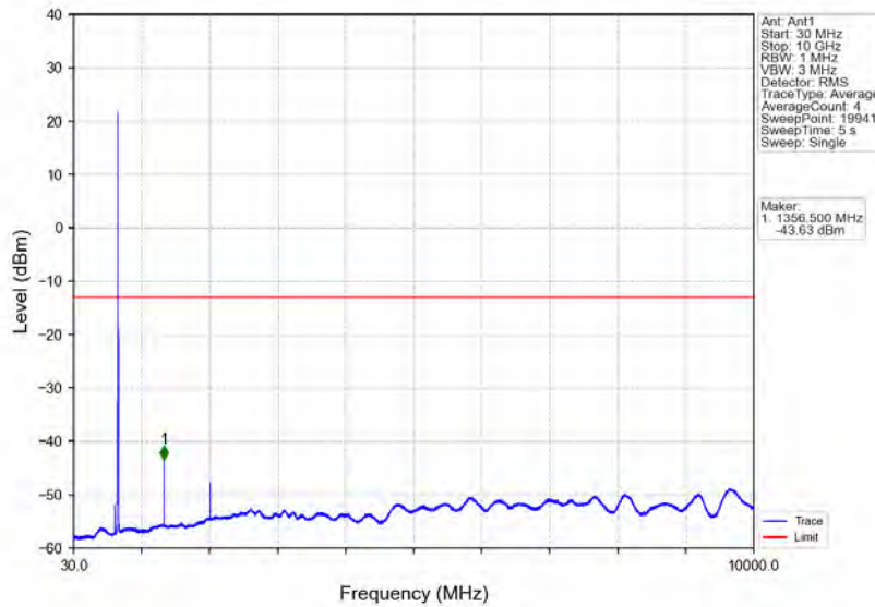
Band71_5MHz_16QAM_HCH_695.5MHz_RB_1_0_NTNV
