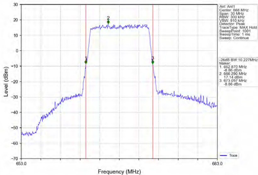
Band71_10MHz_64QAM_LCH_668MHz_RB_50_0_NTNV
