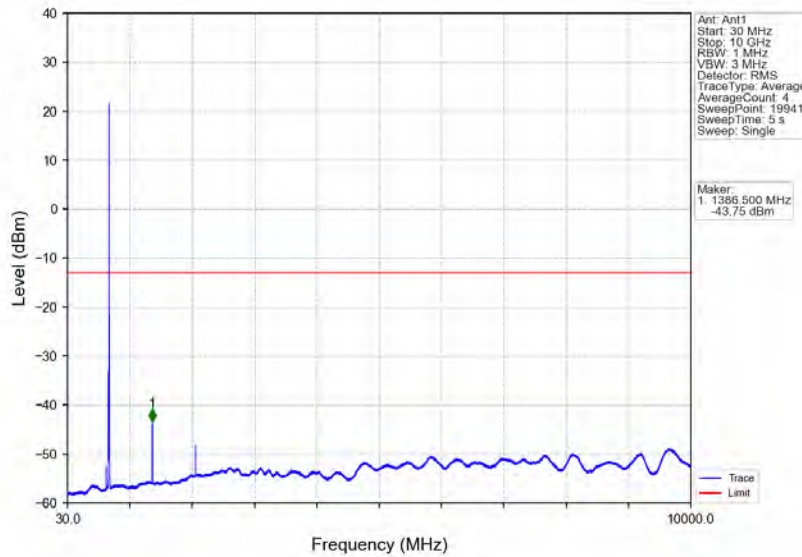
Band71_5MHz_64QAM_HCH_695.5MHz_RB_1_24_NTNV
