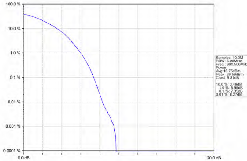
Band71_15MHz_64QAM_HCH_690.5MHz_RB_75_0_NTNV
