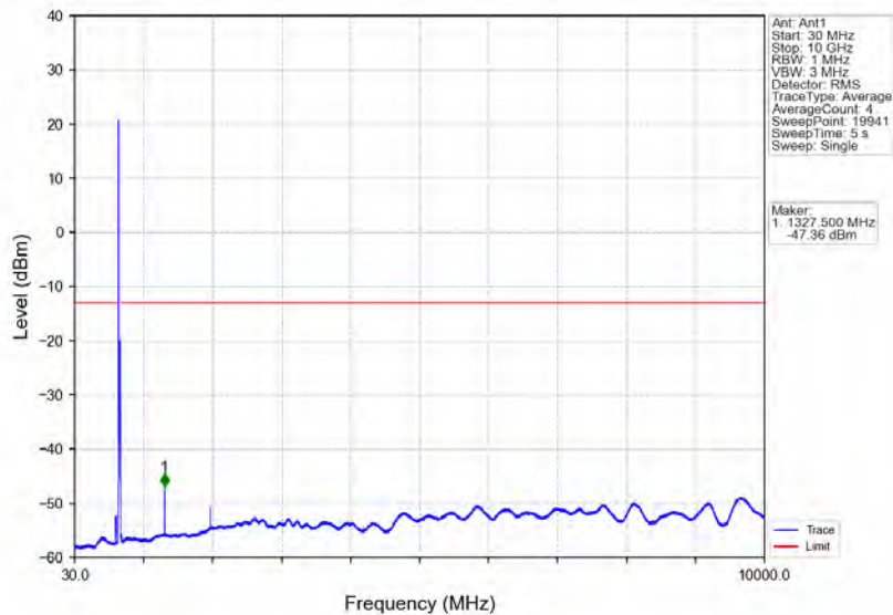
Band71_15MHz_64QAM_LCH_670.5MHz_RB_1_0_NTNV
