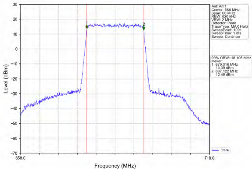
Band71_20MHz_64QAM_HCH_688MHz_RB_100_0_NTNV
