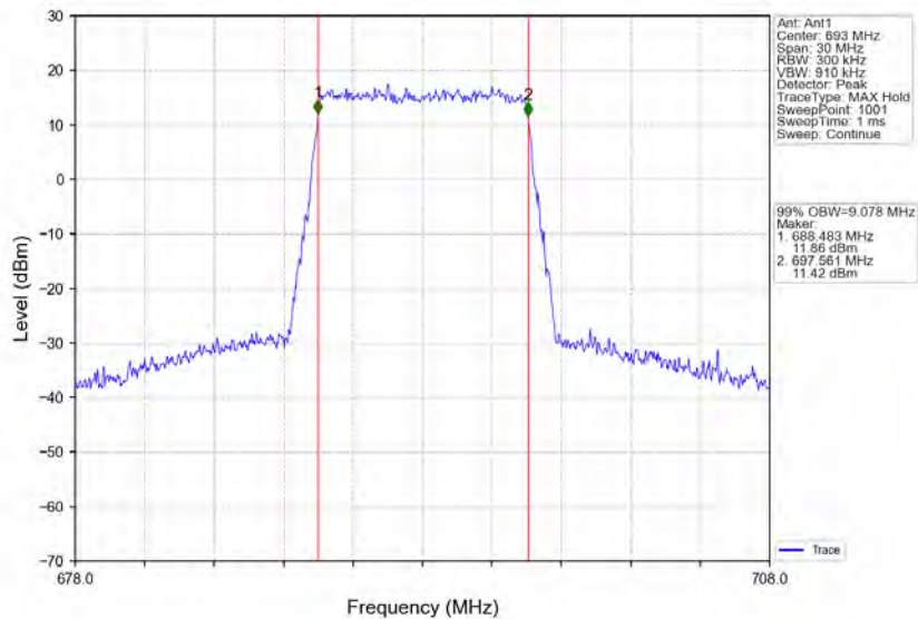
Band71_10MHz_64QAM_HCH_693MHz_RB_50_0_NTNV
