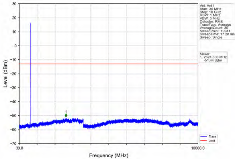
Band71_5MHz_16QAM_LCH_665.5MHz_RB_25_0_NTNV
