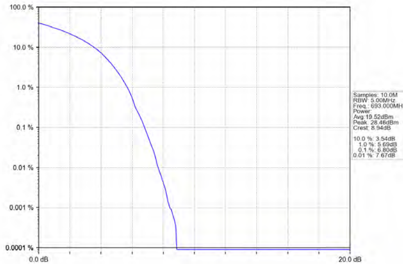
Band71_10MHz_16QAM_HCH_693MHz_RB_50_0_NTNV
