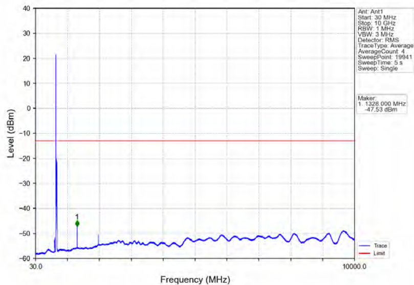
Band71_20MHz_64QAM_LCH_673MHz_RB_1_0_NTV
