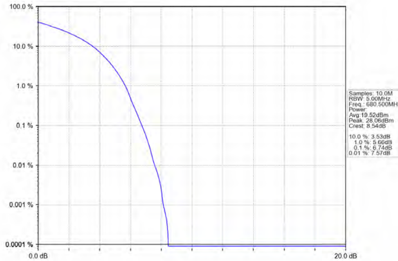
Band71_10MHz_16QAM_MCH_680.5MHz_RB_50_0_NTNV
