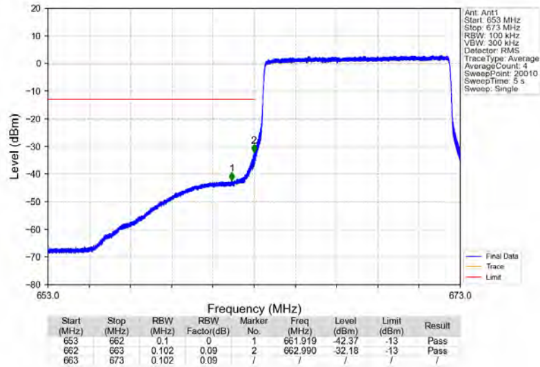
Band71_10MHz_64QAM_LCH_668MHz_RB_50_0_NTNV
