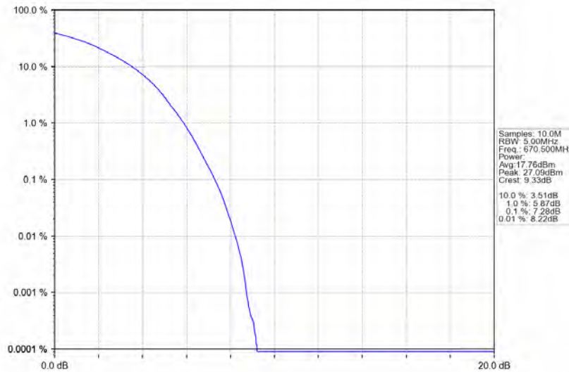
Band71_15MHz_16QAM_LCH_670.5MHz_RB_75_0_NTNV
