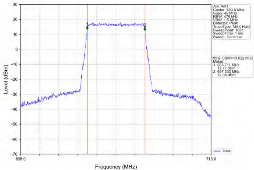
Band71_15MHz_16QAM_HCH_690.5MHz_RB_75_0_NTNV
