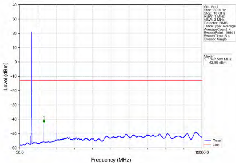
Band71_15MHz_64QAM_MCH_680.5MHz_RB_1_0_NTNV
