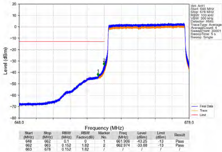
Band71_15MHz_64QAM_LCH_670.5MHz_RB_75_0_NTNV
