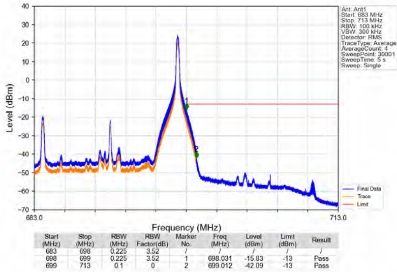
Band71_15MHz_64QAM_HCH_690.5MHz_RB_1_74_NTNV
