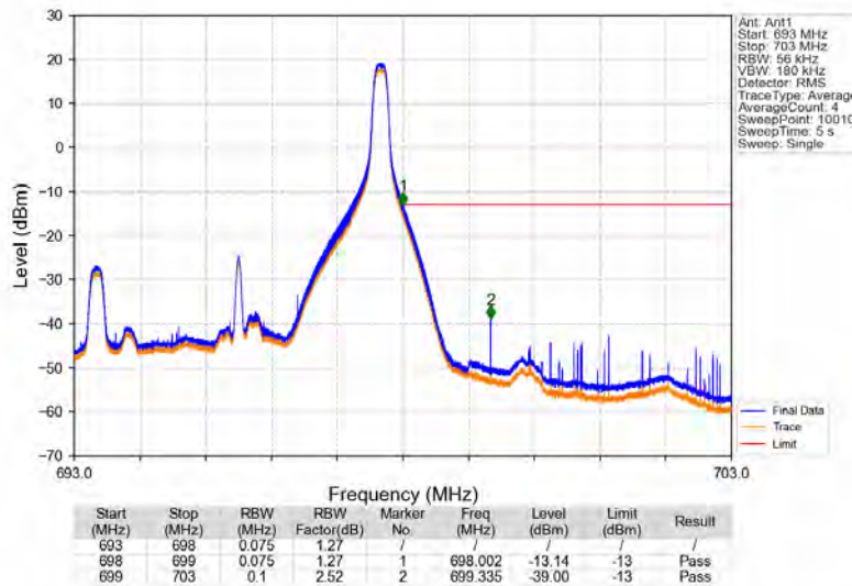
Band71_5MHz_64QAM_HCH_695.5MHz_RB_1_24_NTNV
