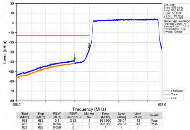
Band71_5MHz_16QAM_LCH_665.5MHz_RB_25_0_NTNV
