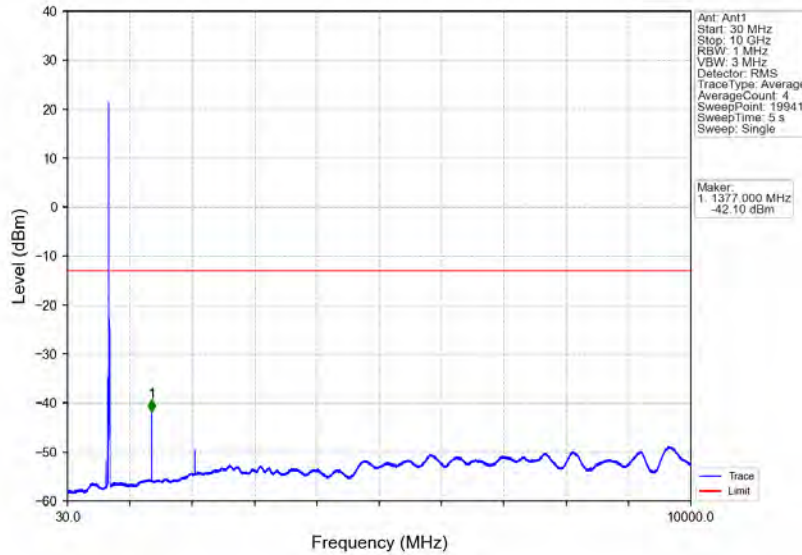
Band71_10MHz_64QAM_HCH_693MHz_RB_1_49_NTNV
