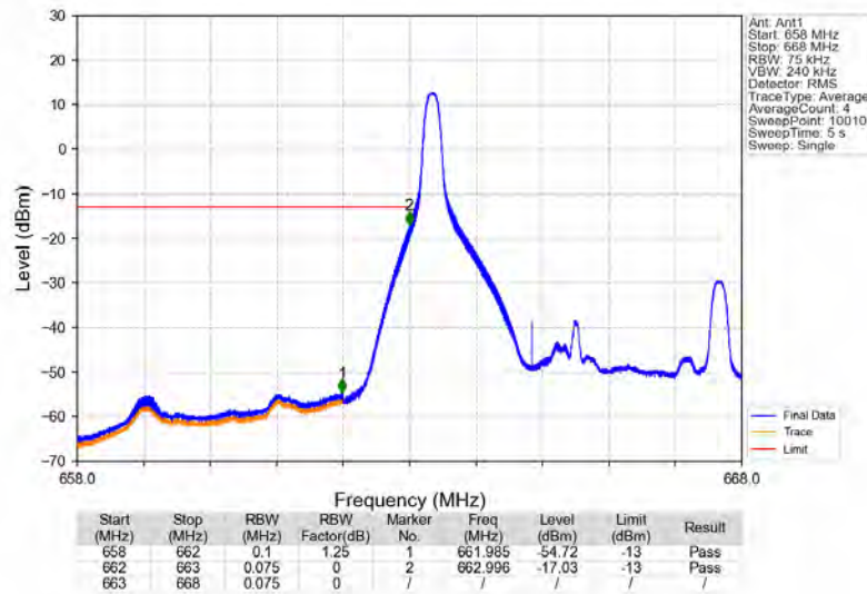
Band71_5MHz_64QAM_LCH_665.5MHz_RB_1_0_NTNV
