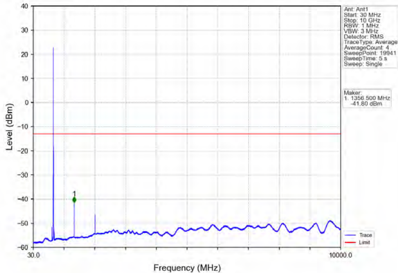
Band71_5MHz_QPSK_MCH_680.5MHz_RB_1_0_NTNV
