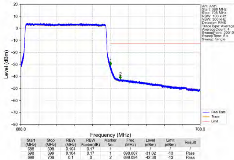
Band71_10MHz_16QAM_HCH_693MHz_RB_50_0_NTV
