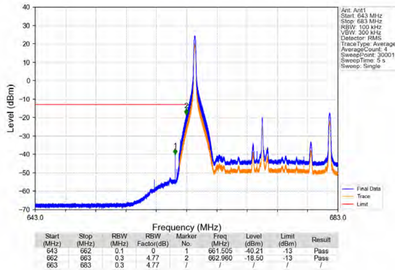
Band71_20MHz_64QAM_LCH_673MHz_RB_1_0_NTV
