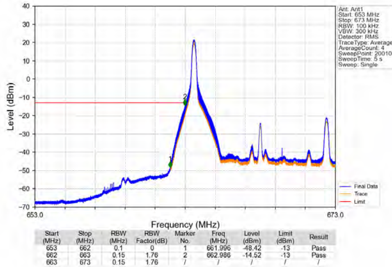
Band71_10MHz_64QAM_LCH_668MHz_RB_1_0_NTV
