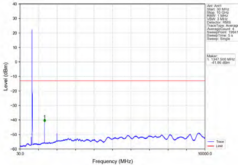
Band71_15MHz_16QAM_HCH_690.5MHz_RB_1_0_NTNV
