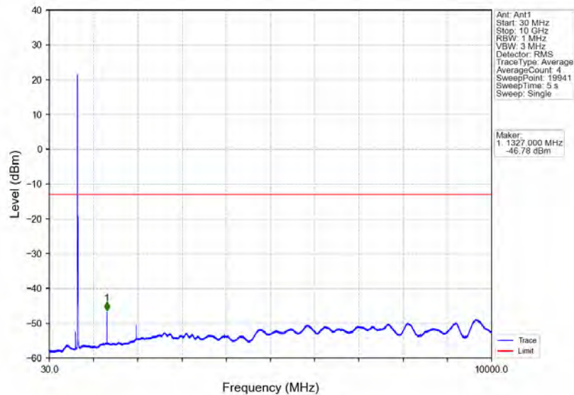
Band71_10MHz_64QAM_LCH_668MHz_RB_1_0_NTV
