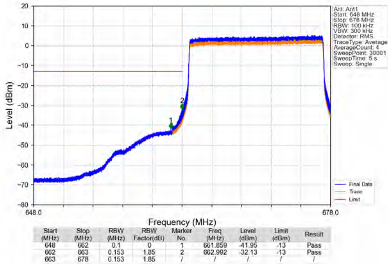
Band71_15MHz_QPSK_LCH_670.5MHz_RB_75_0_NTNV
