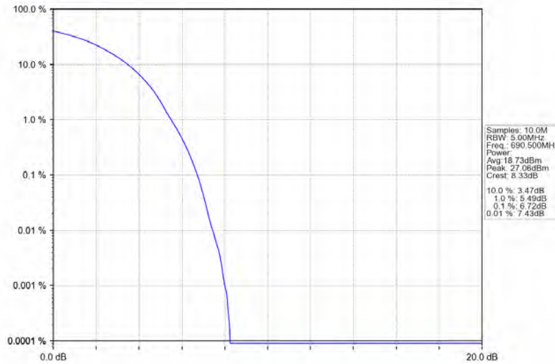
Band71_15MHz_QPSK_HCH_690.5MHz_RB_75_0_NTNV
