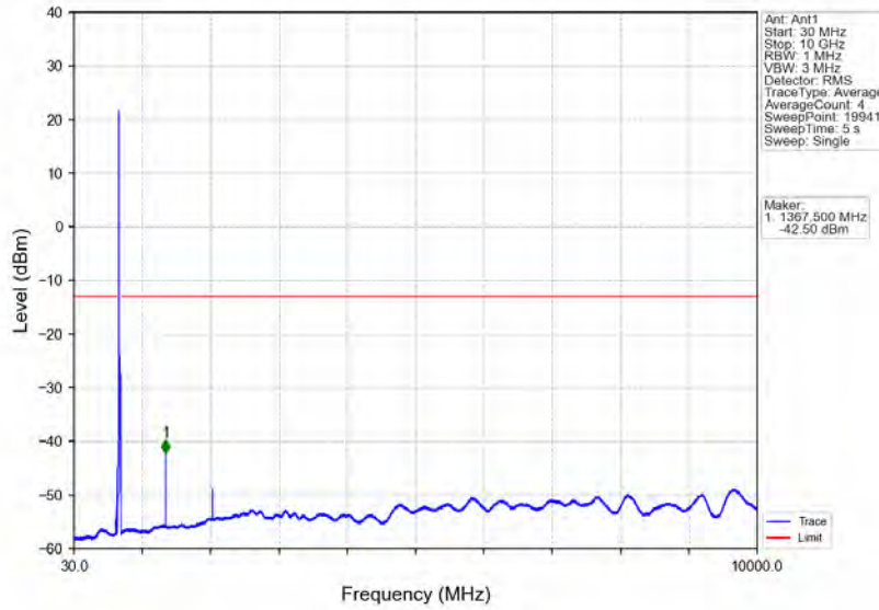
Band71_15MHz_64QAM_HCH_690.5MHz_RB_1_74_NTNV
