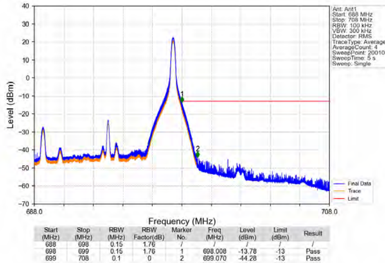
Band71_10MHz_16QAM_HCH_693MHz_RB_1_49_NTV
