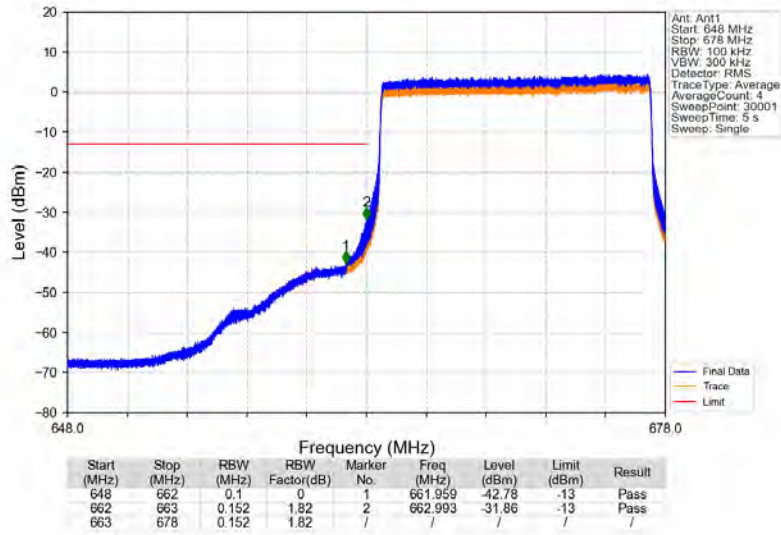
Band71_15MHz_16QAM_LCH_670.5MHz_RB_75_0_NTNV
