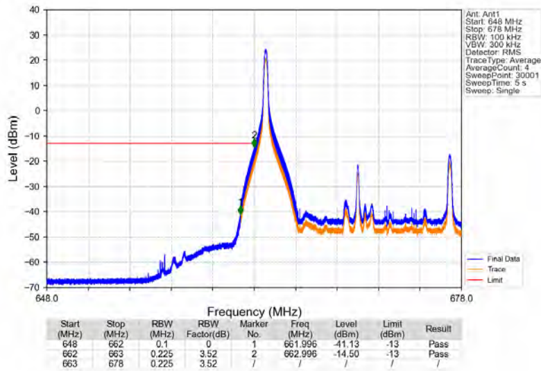
Band71_15MHz_16QAM_LCH_670.5MHz_RB_1_0_NTNV
