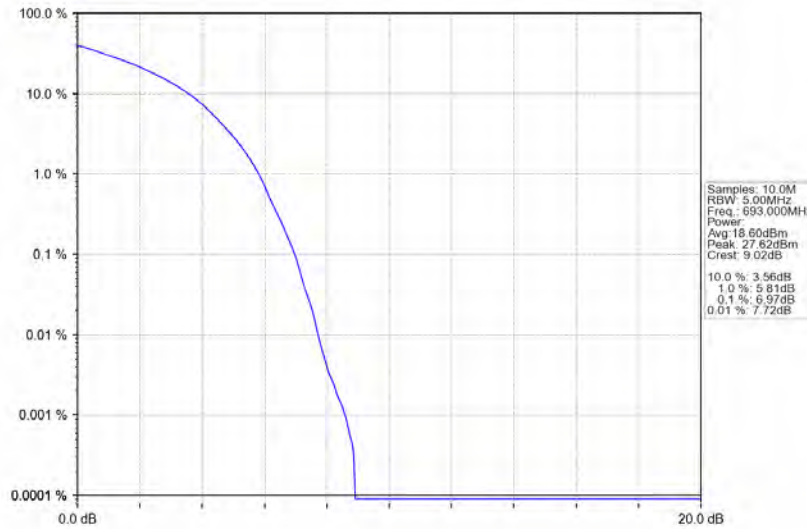
Band71_10MHz_64QAM_HCH_693MHz_RB_50_0_NTV
