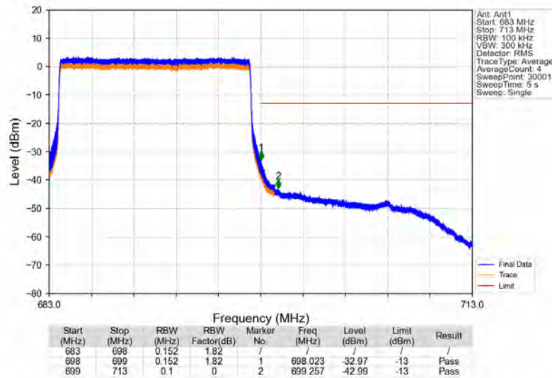
Band71_15MHz_64QAM_HCH_690.5MHz_RB_75_0_NTNV
