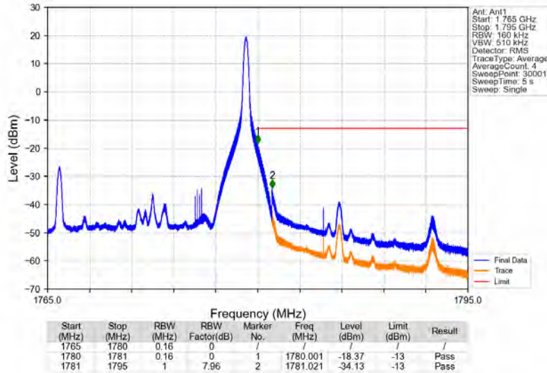
Band66_15MHz_64QAM_HCH_1772.5MHz_RB_1_74_NTNV
