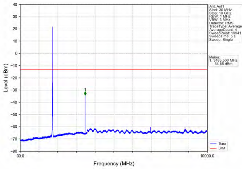
Band66_5MHz_QPSK_MCH_1745MHz_RB_1_0_NTNV
