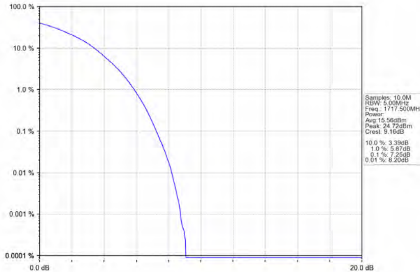
Band66_15MHz_64QAM_LCH_1717.5MHz_RB_75_0_NTNV
