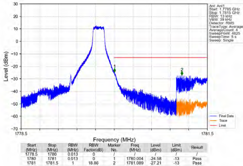
Band66_1.4MHz_QPSK_HCH_1779.3MHz_RB_1_5_NTNV
