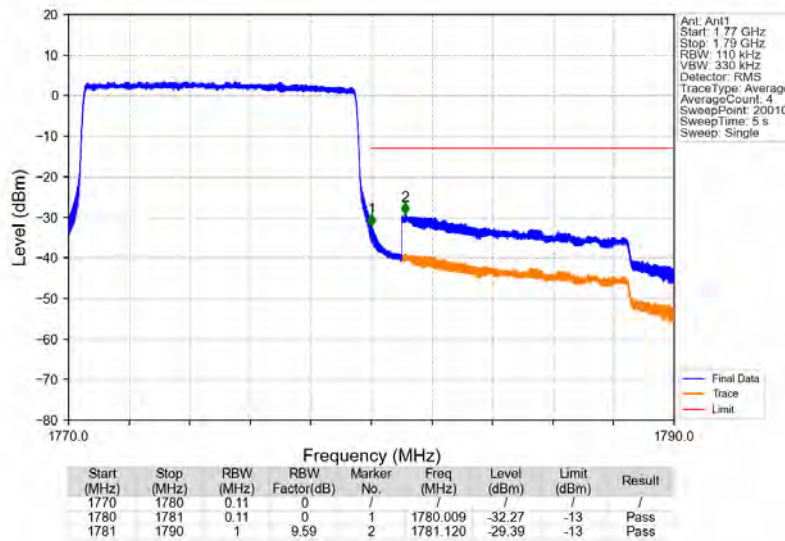
Band66_10MHz_QPSK_HCH_1775MHz_RB_50_0_NTV
