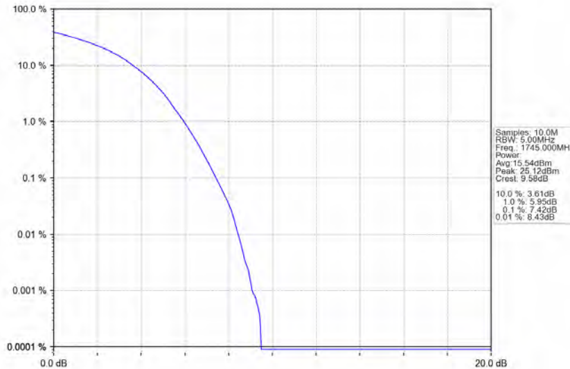
Band66_20MHz_16QAM_MCH_1745MHz_RB_100_0_NTNV
