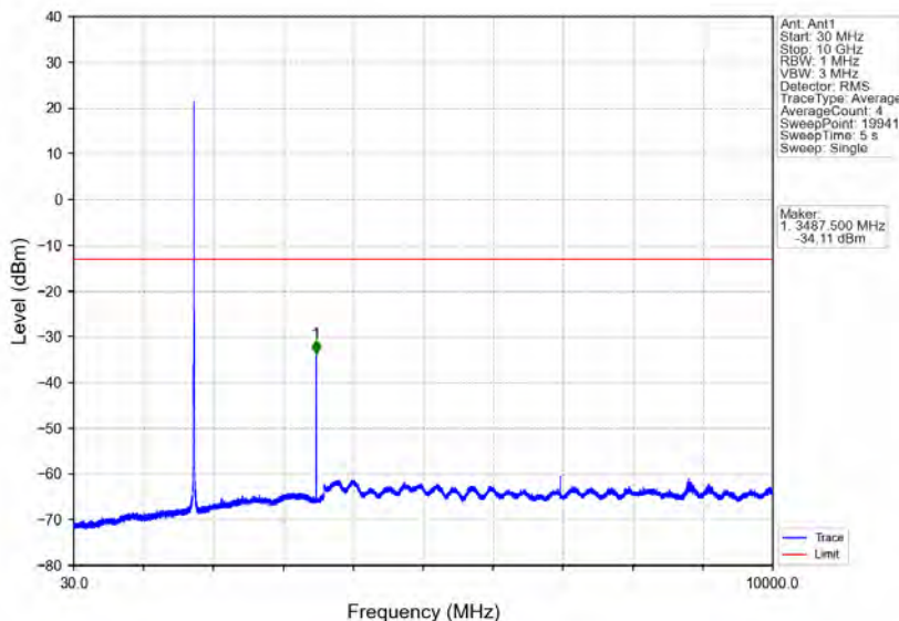
Band66_3MHz_QPSK_MCH_1745MHz_RB_1_0_NTNV
