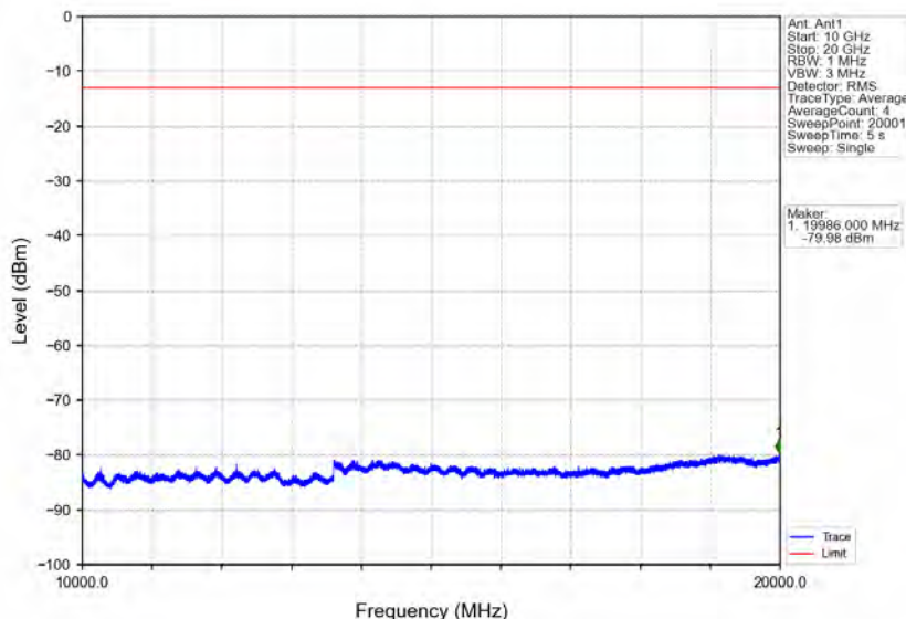
Band66_3MHz_QPSK_MCH_1745MHz_RB_1_0_NTNV
