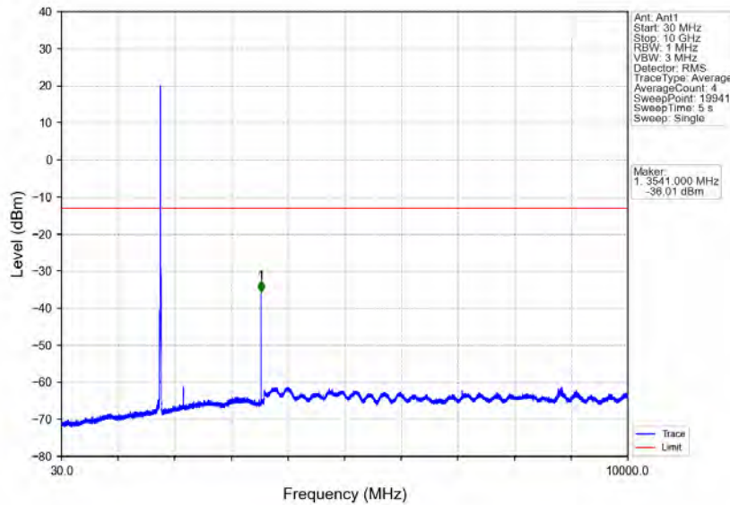
Band66_10MHz_64QAM_HCH_1775MHz_RB_1_0_NTV
