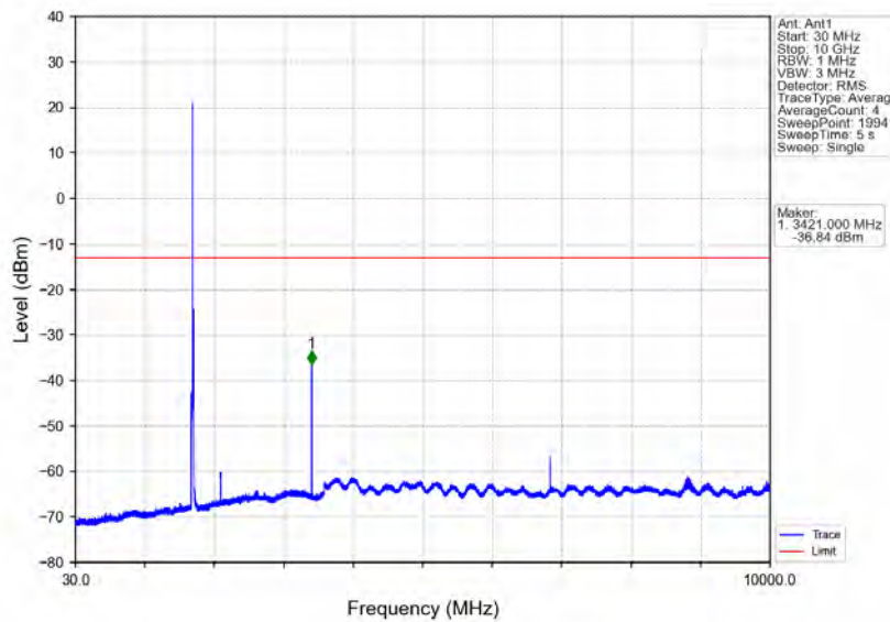
Band66_10MHz_16QAM_LCH_1715MHz_RB_1_0_NTNV
