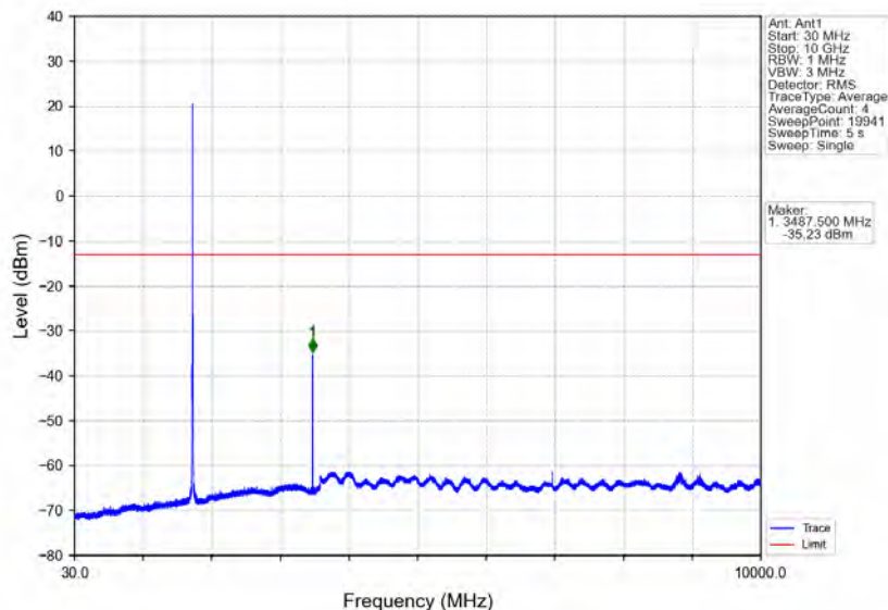
Band66_3MHz_16QAM_MCH_1745MHz_RB_1_0_NTNV
