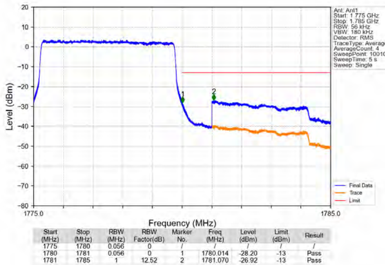
Band66_5MHz_QPSK_HCH_1777.5MHz_RB_25_0_NTNV
