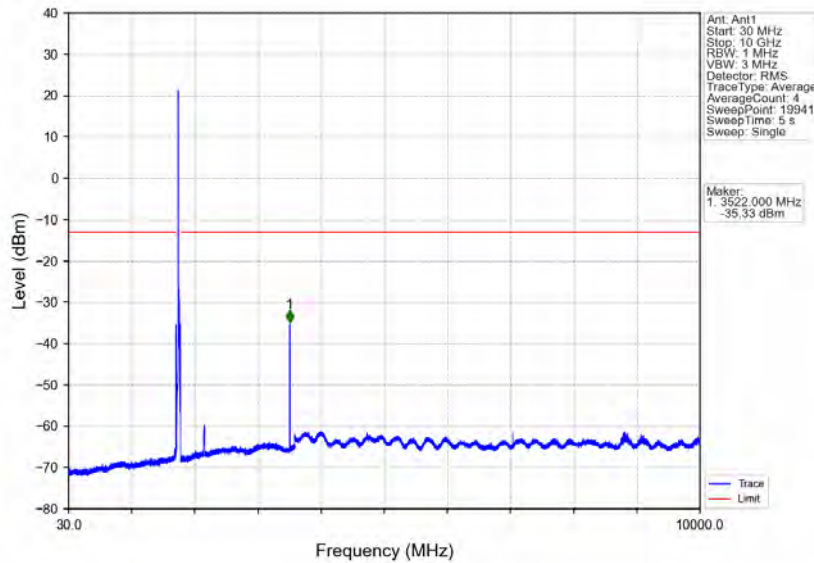
Band66_20MHz_16QAM_HCH_1770MHz_RB_1_0_NTV
