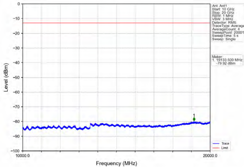
Band66_10MHz_64QAM_HCH_1775MHz_RB_1_0_NTV
