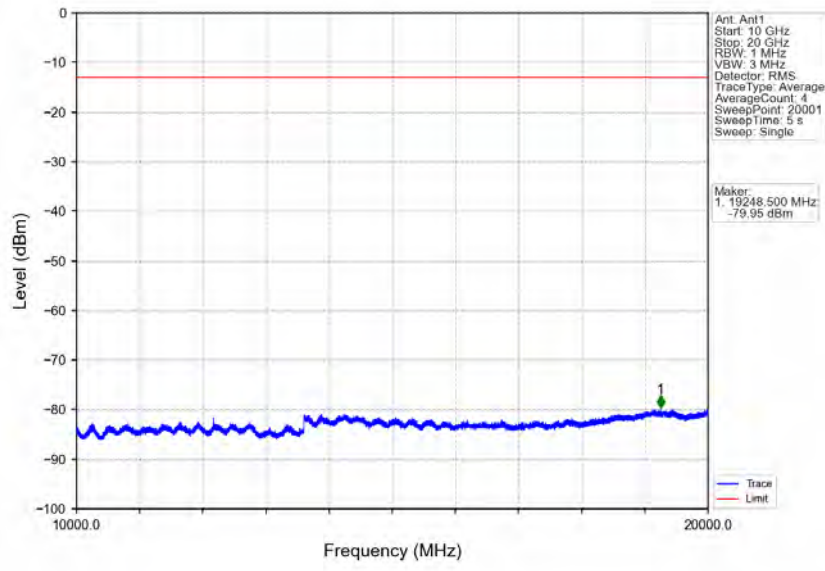
Band66_15MHz_64QAM_MCH_1745MHz_RB_1_0_NTNV
