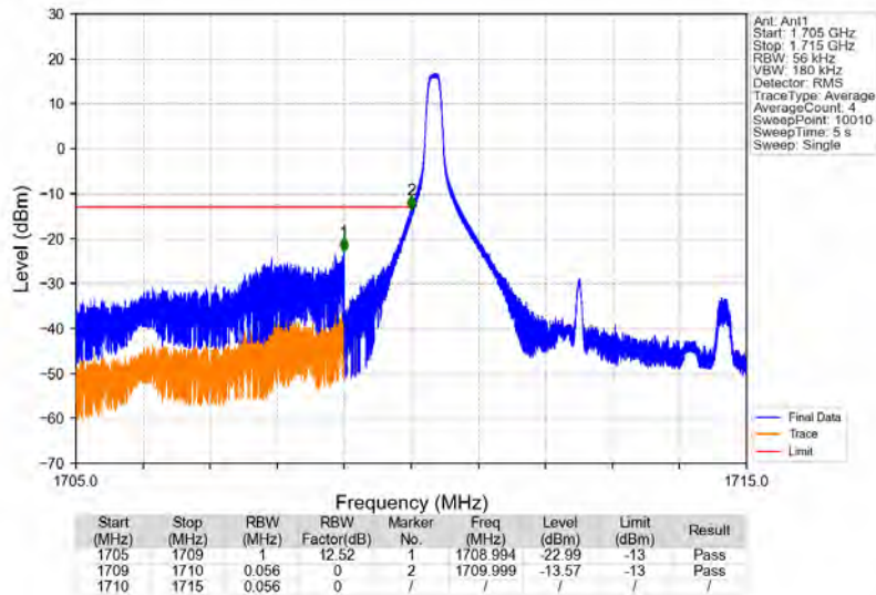
Band66_5MHz_16QAM_LCH_1712.5MHz_RB_1_0_NTNV
