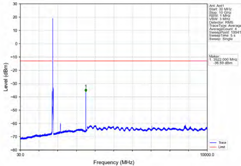
Band66_20MHz_64QAM_HCH_1770MHz_RB_1_0_NTV
