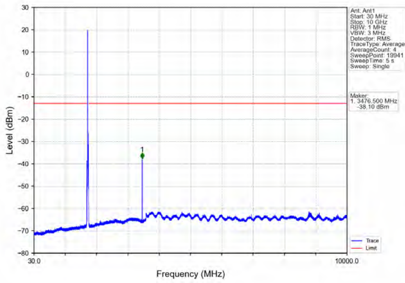
Band66_15MHz_64QAM_MCH_1745MHz_RB_1_0_NTNV
