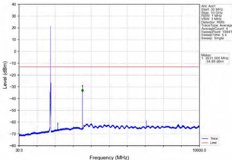
Band66_15MHz_QPSK_HCH_1772.5MHz_RB_1_0_NTNV
