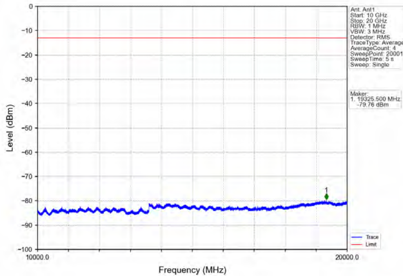
Band66_20MHz_16QAM_HCH_1770MHz_RB_1_0_NTV
