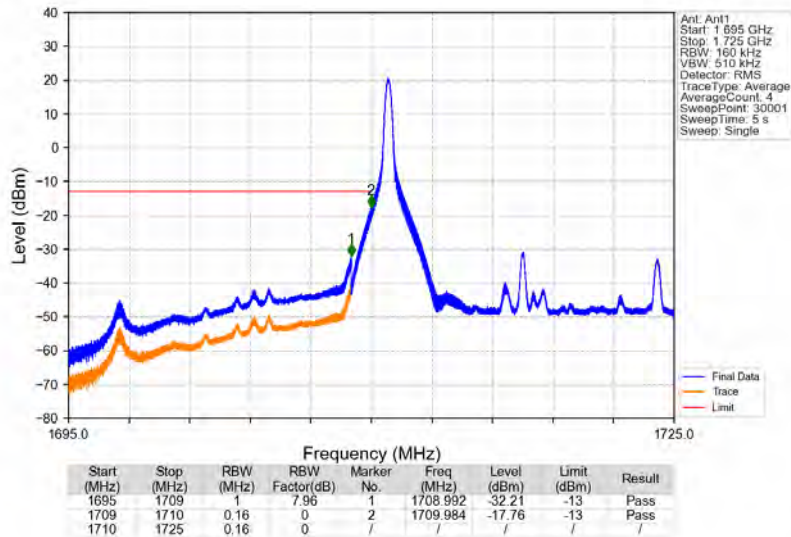
Band66_15MHz_16QAM_LCH_1717.5MHz_RB_1_0_NTNV
