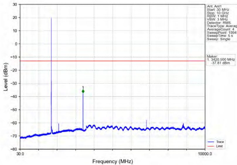
Band66_3MHz_64QAM_LCH_1711.5MHz_RB_1_0_NTNV
