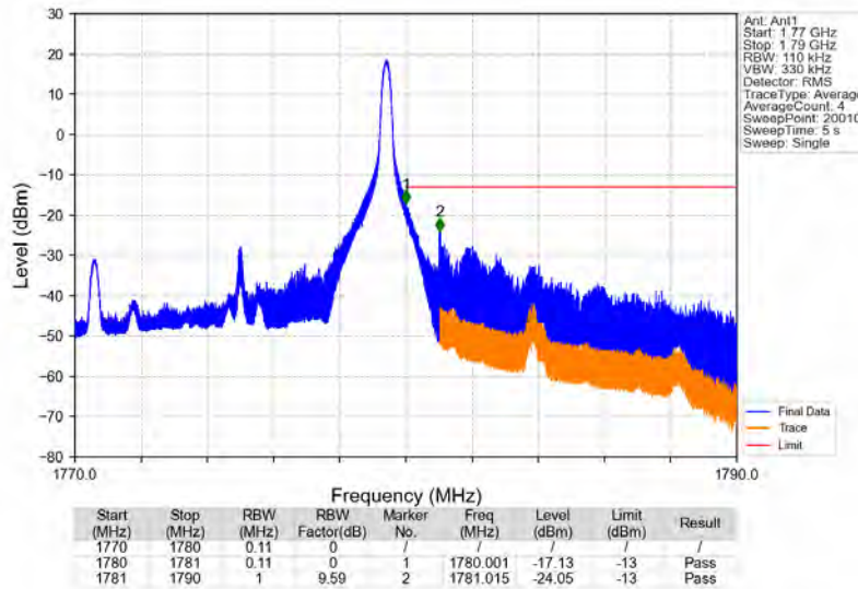
Band66_10MHz_64QAM_HCH_1775MHz_RB_1_49_NTNV
