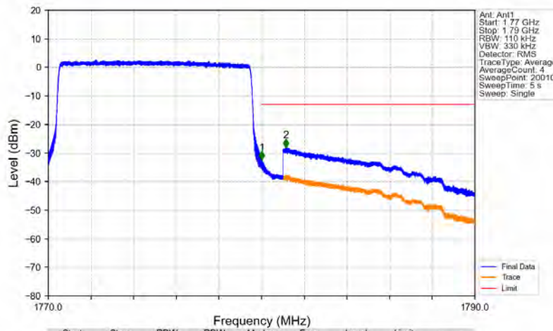
Band66_10MHz_16QAM_HCH_1775MHz_RB_50_0_NTNV
