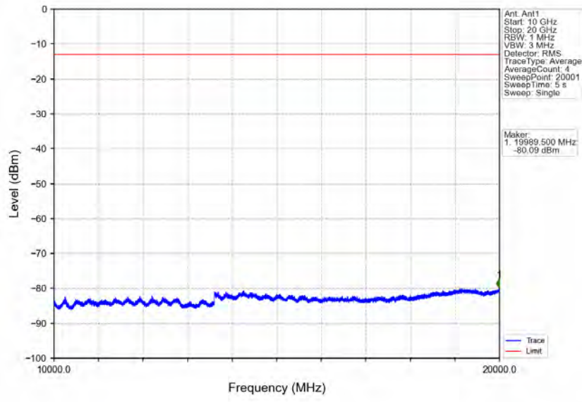
Band66_5MHz_QPSK_MCH_1745MHz_RB_1_0_NTNV
