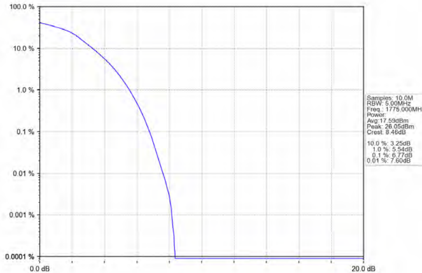
Band66_10MHz_64QAM_HCH_1775MHz_RB_50_0_NTNV
