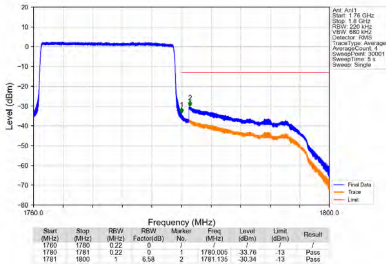
Band66_20MHz_16QAM_HCH_1770MHz_RB_100_0_NTNV
