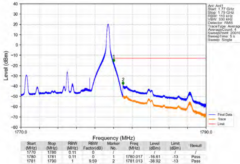
Band66_10MHz_QPSK_HCH_1775MHz_RB_1_49_NTV
