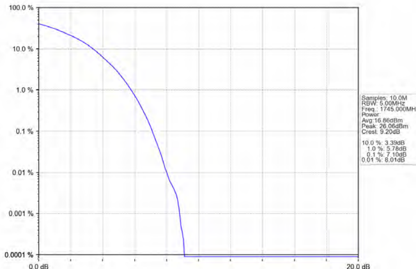
Band66_15MHz_16QAM_MCH_1745MHz_RB_75_0_NTNV
