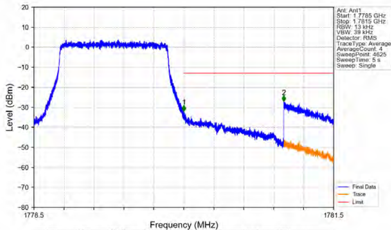
Band66_1.4MHz_16QAM_HCH_1779.3MHz_RB_6_0_NTNV
