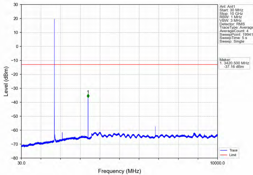
Band66_1.4MHz_64QAM_LCH_1710.7MHz_RB_1_0_NTNV
