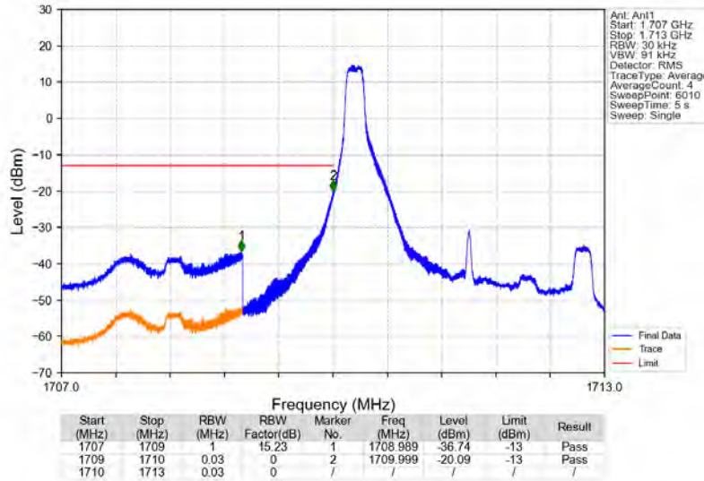
Band66_3MHz_16QAM_LCH_1711.5MHz_RB_1_0_NTNV
