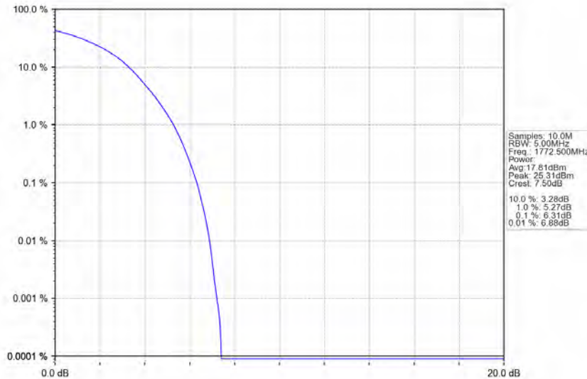
Band66_15MHz_QPSK_HCH_1772.5MHz_RB_75_0_NTNV
