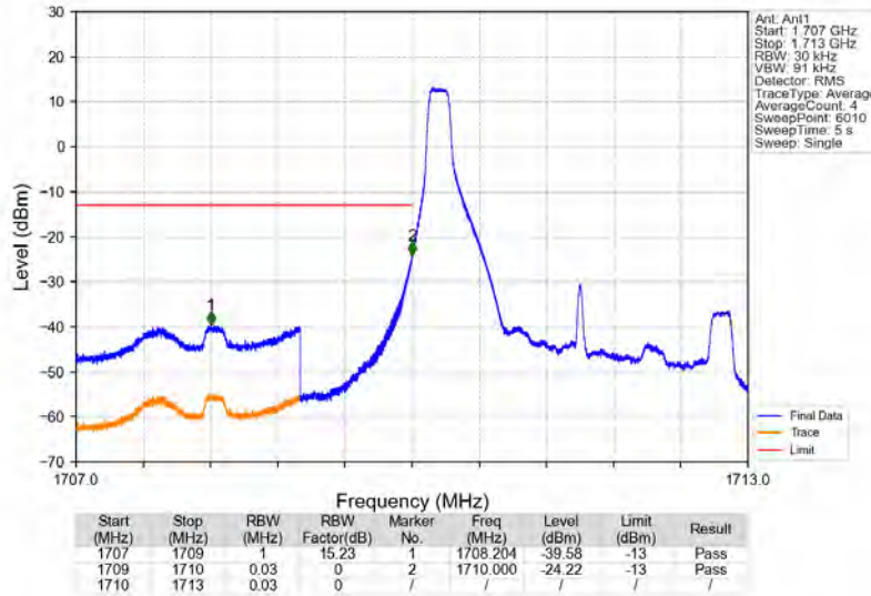
Band66_3MHz_64QAM_LCH_1711.5MHz_RB_1_0_NTNV
