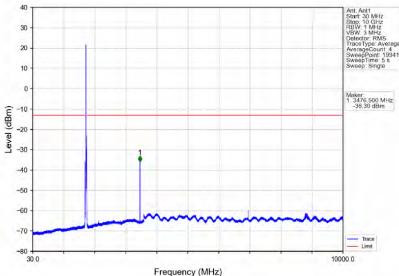
Band66_15MHz_QPSK_MCH_1745MHz_RB_1_0_NTNV
