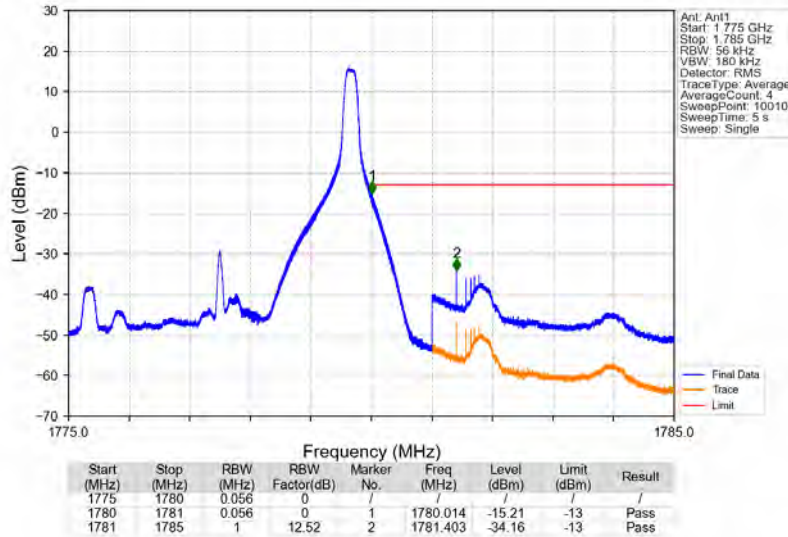
Band66_5MHz_64QAM_HCH_1777.5MHz_RB_1_24_NTNV
