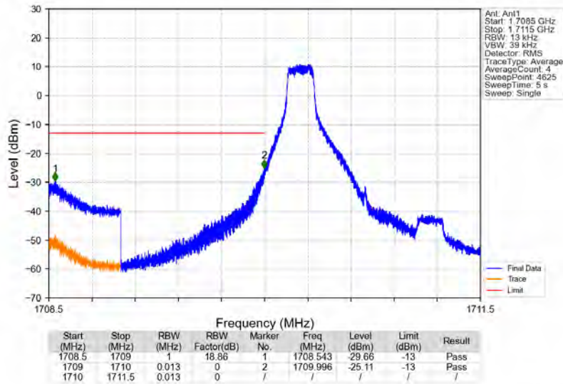
Band66_1.4MHz_64QAM_LCH_1710.7MHz_RB_1_0_NTNV
