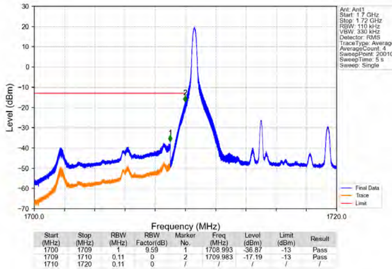
Band66_10MHz_16QAM_LCH_1715MHz_RB_1_0_NTNV
