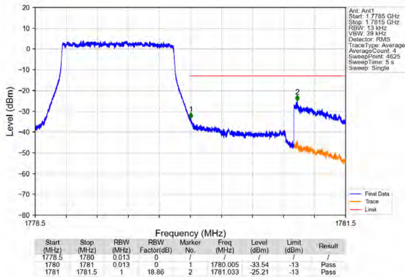
Band66_1.4MHz_QPSK_HCH_1779.3MHz_RB_6_0_NTNV
