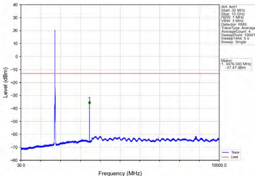
Band66_15MHz_16QAM_MCH_1745MHz_RB_1_0_NTNV
