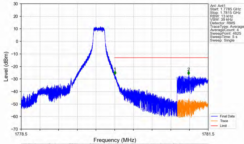
Band66_1.4MHz_16QAM_HCH_1779.3MHz_RB_1_5_NTNV
