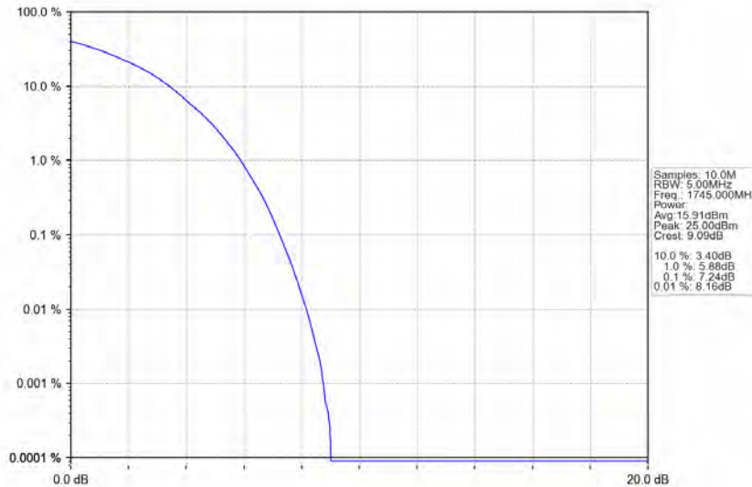
Band66_15MHz_64QAM_MCH_1745MHz_RB_75_0_NTNV
