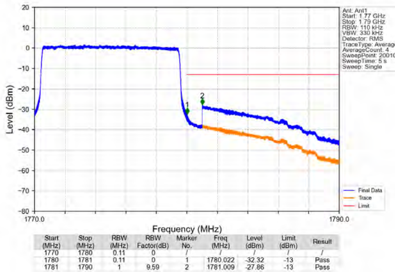
Band66_10MHz_64QAM_HCH_1775MHz_RB_50_0_NTNV
