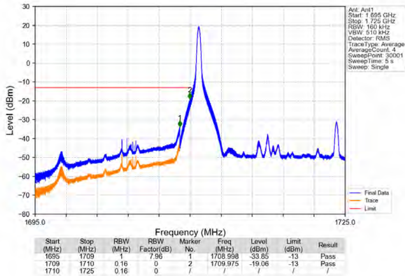
Band66_15MHz_64QAM_LCH_1717.5MHz_RB_1_0_NTNV
