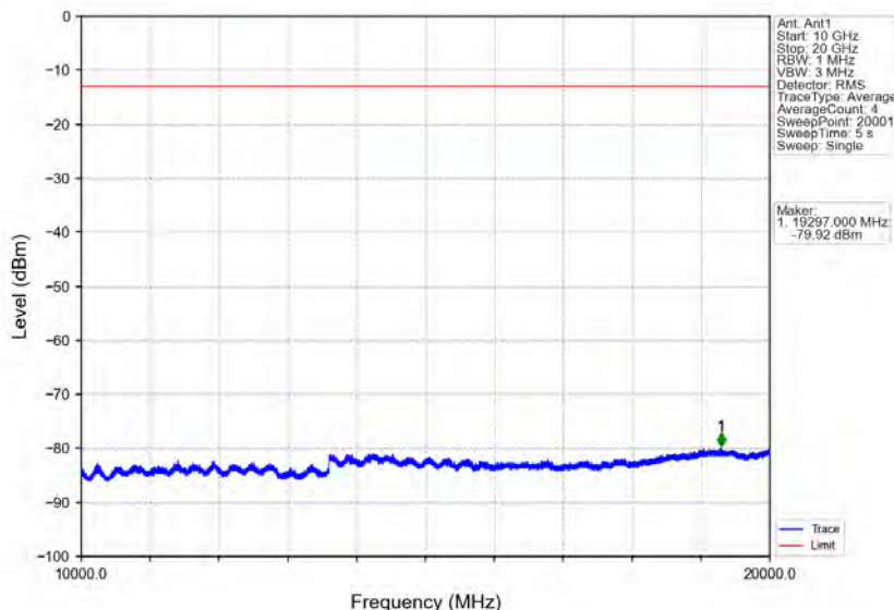
Band66_15MHz_QPSK_HCH_1772.5MHz_RB_1_0_NTNV
