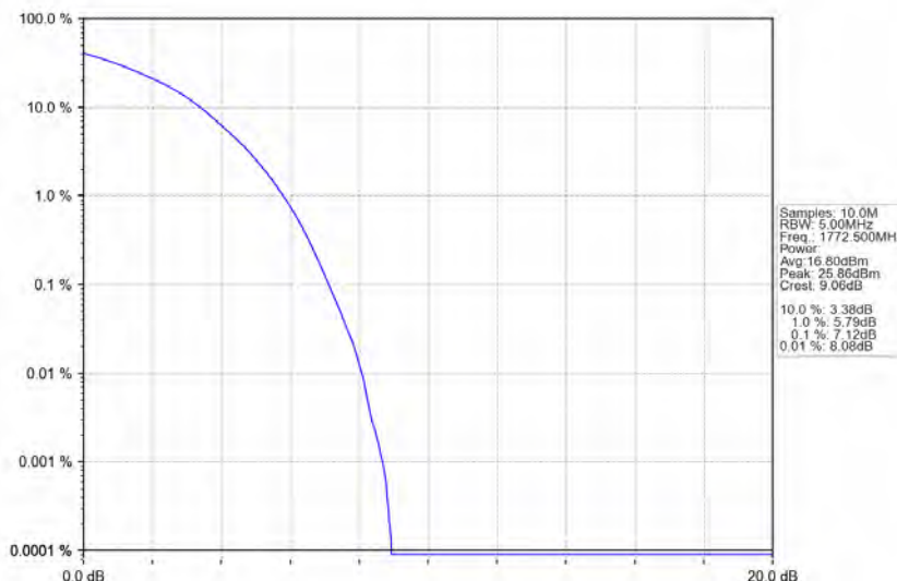
Band66_15MHz_16QAM_HCH_1772.5MHz_RB_75_0_NTNV
