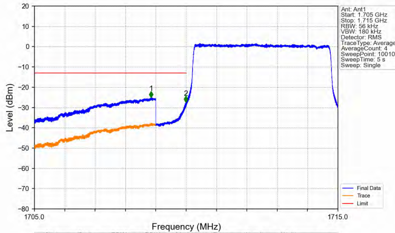
Band66_5MHz_64QAM_LCH_1712.5MHz_RB_25_0_NTNV
