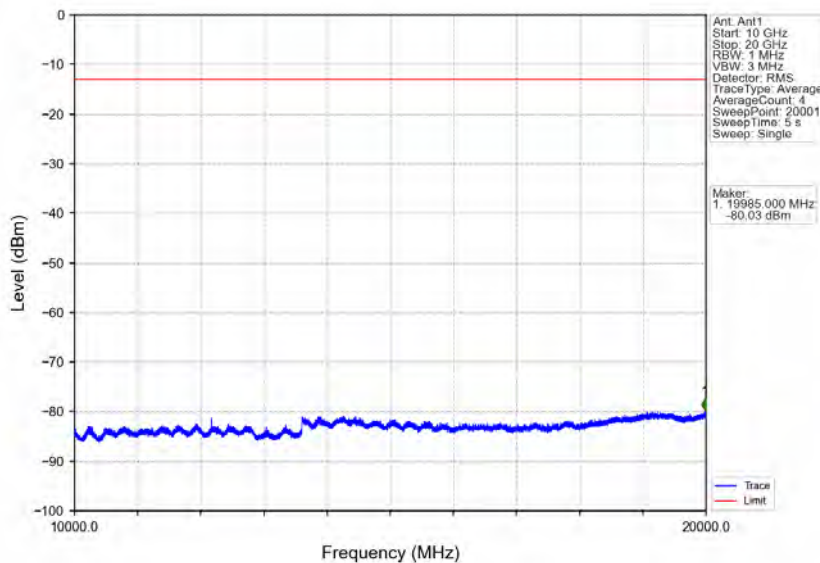
Band66_15MHz_QPSK_MCH_1745MHz_RB_1_0_NTNV
