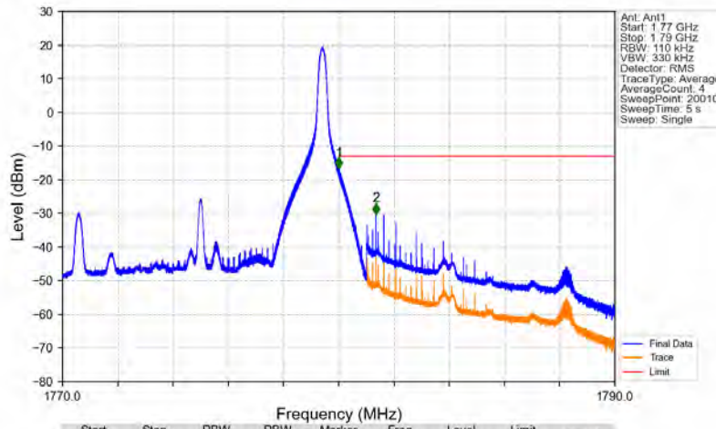
Band66_10MHz_16QAM_HCH_1775MHz_RB_1_49_NTNV
