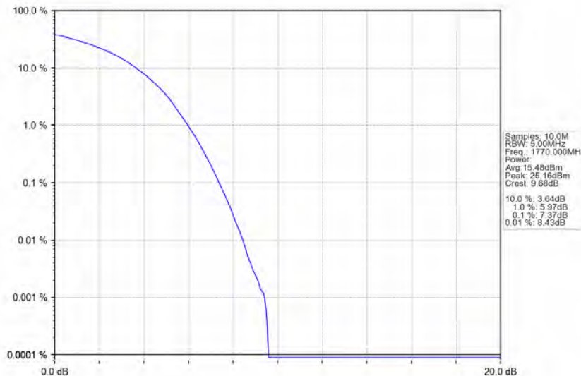
Band66_20MHz_16QAM_HCH_1770MHz_RB_100_0_NTNV
