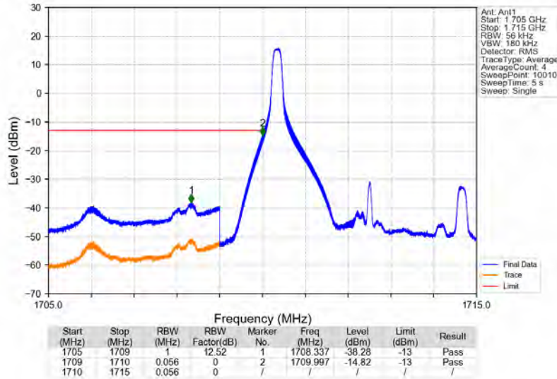
Band66_5MHz_64QAM_LCH_1712.5MHz_RB_1_0_NTNV
