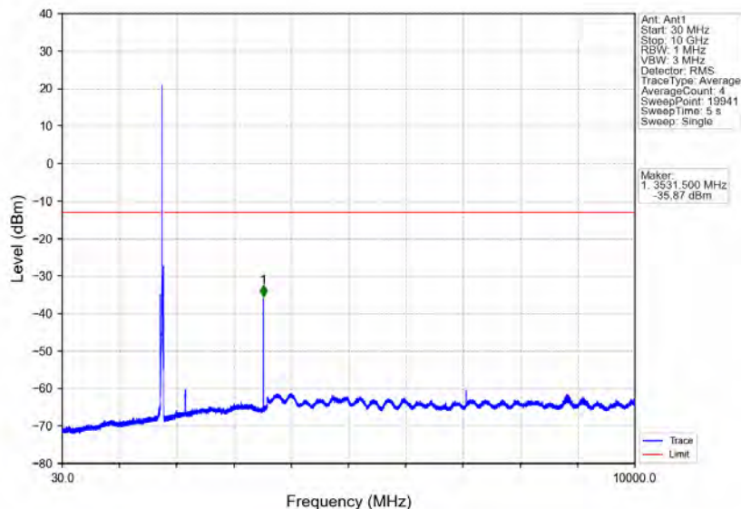
Band66_15MHz_16QAM_HCH_1772.5MHz_RB_1_0_NTNV
