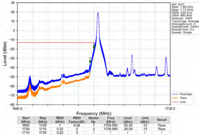
Band66_20MHz_64QAM_LCH_1720MHz_RB_1_0_NTNV
