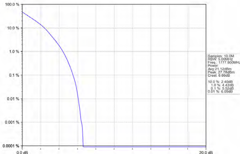
Band66_5MHz_QPSK_HCH_1777.5MHz_RB_25_0_NTNV
