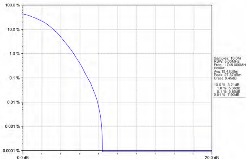
Band66_1.4MHz_64QAM_MCH_1745MHz_RB_6_0_NTNV
