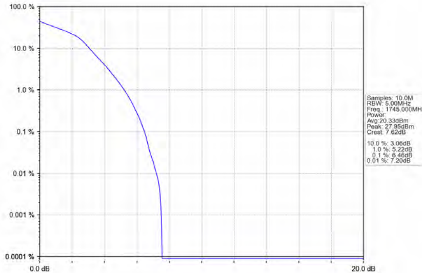
Band66_1.4MHz_16QAM_MCH_1745MHz_RB_6_0_NTNV
