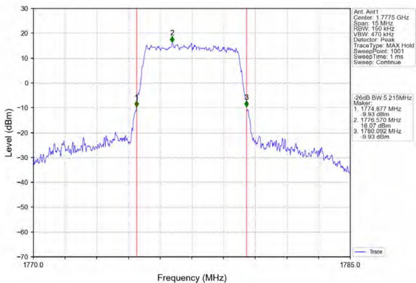
Band66_5MHz_16QAM_HCH_1777.5MHz_RB_25_0_NTNV
