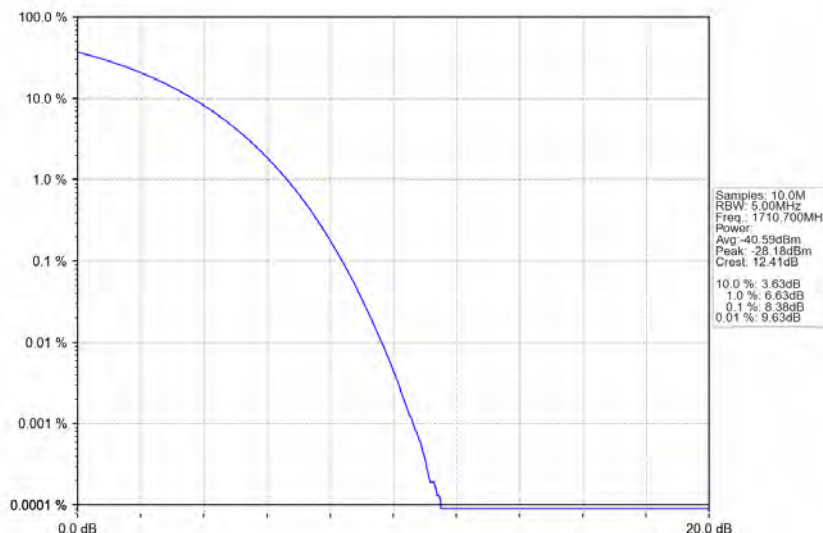
Band66_1.4MHz_16QAM_LCH_1710.7MHz_RB_6_0_NTNV
