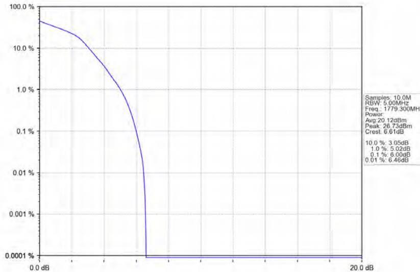
Band66_1.4MHz_16QAM_HCH_1779.3MHz_RB_6_0_NTNV
