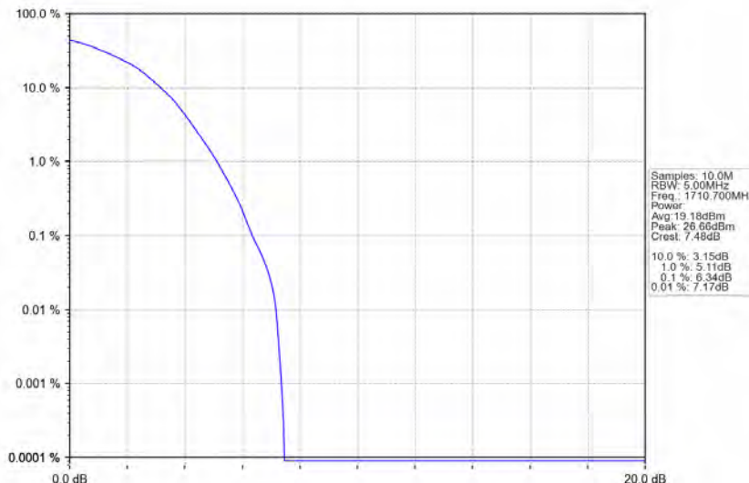
Band66_1.4MHz_64QAM_LCH_1710.7MHz_RB_6_0_NTNV
