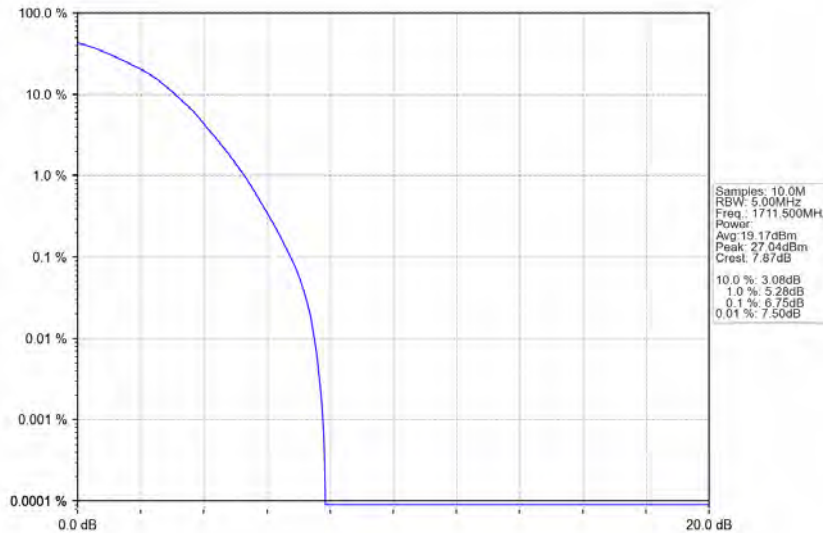
Band66_3MHz_64QAM_LCH_1711.5MHz_RB_15_0_NTNV
