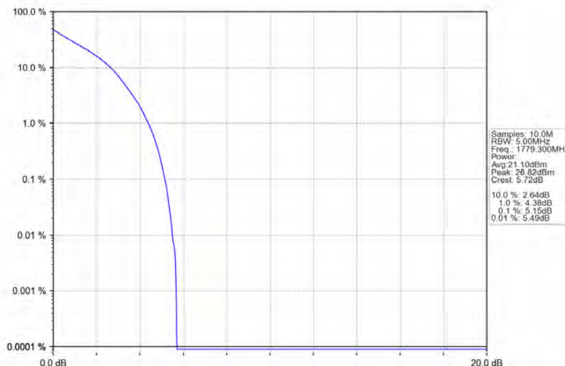
Band66_1.4MHz_QPSK_HCH_1779.3MHz_RB_6_0_NTNV
