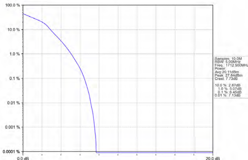
Band66_5MHz_16QAM_LCH_1712.5MHz_RB_25_0_NTNV
