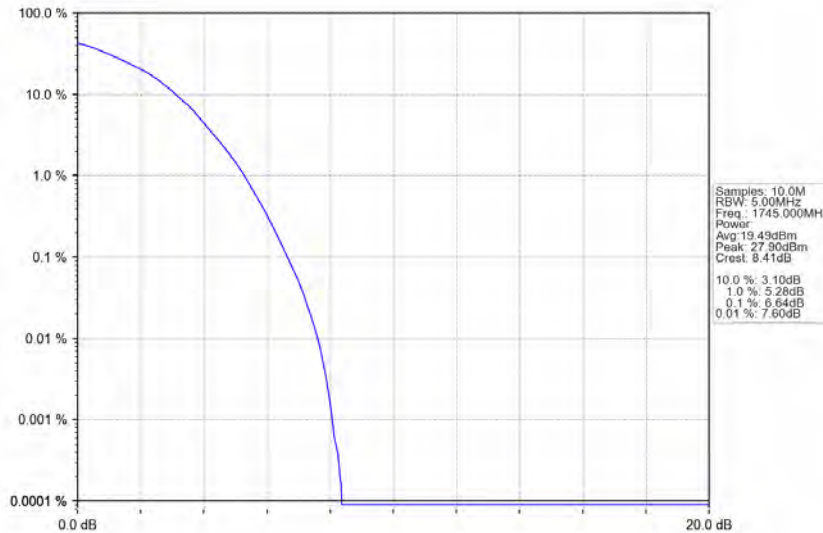
Band66_3MHz_64QAM_MCH_1745MHz_RB_15_0_NTNV
