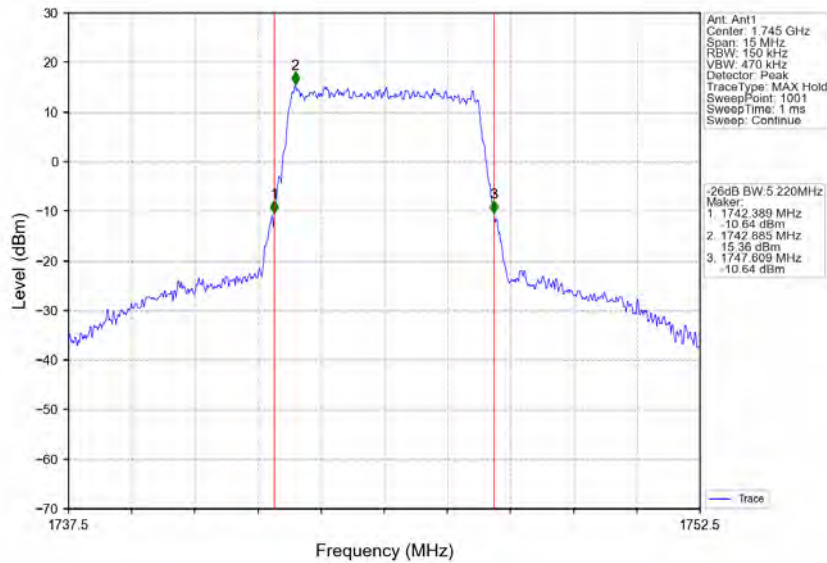
Band66_5MHz_64QAM_MCH_1745MHz_RB_25_0_NTNV
