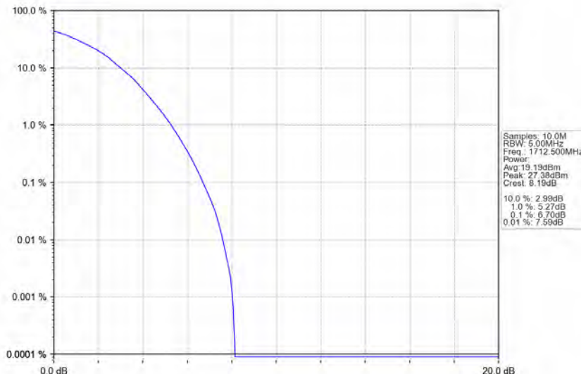
Band66_5MHz_64QAM_LCH_1712.5MHz_RB_25_0_NTNV
