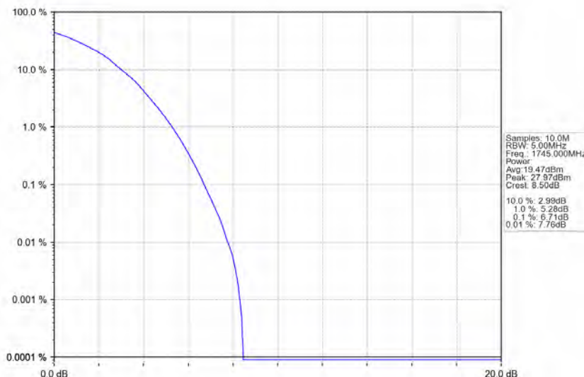
Band66_5MHz_64QAM_MCH_1745MHz_RB_25_0_NTNV
