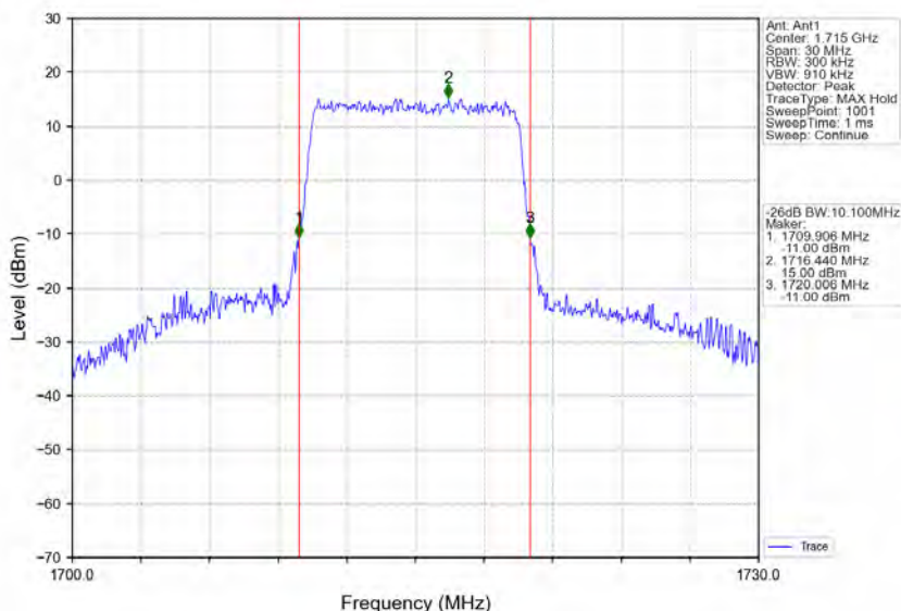
Band66_10MHz_64QAM_LCH_1715MHz_RB_50_0_NTNV
