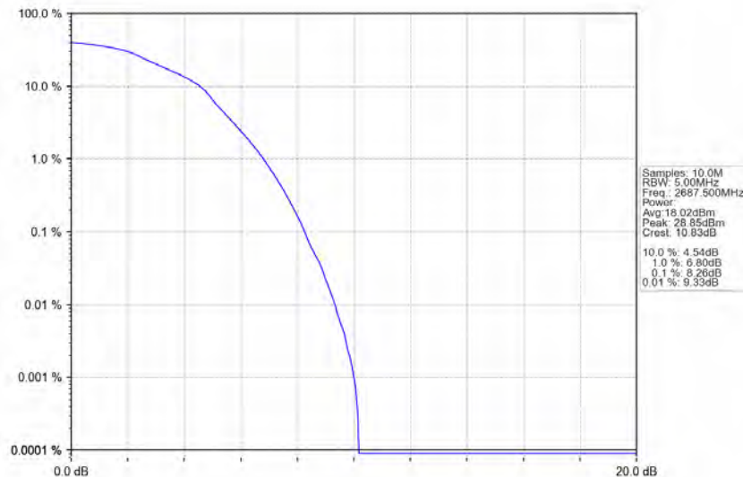
Band41_5MHz_16QAM_HCH_2687.5MHz_RB_25_0_NTNV
