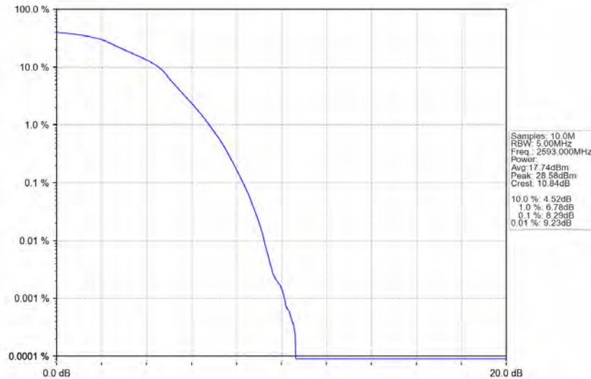
Band41_5MHz_16QAM_MCH_2593MHz_RB_25_0_NTNV
