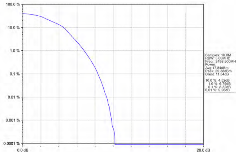
Band41_5MHz_16QAM_LCH_2498.5MHz_RB_25_0_NTNV
