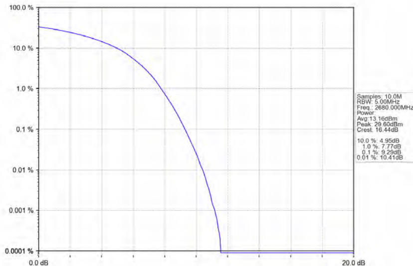
Band41_20MHz_16QAM_HCH_2680MHz_RB_100_0_NTNV
