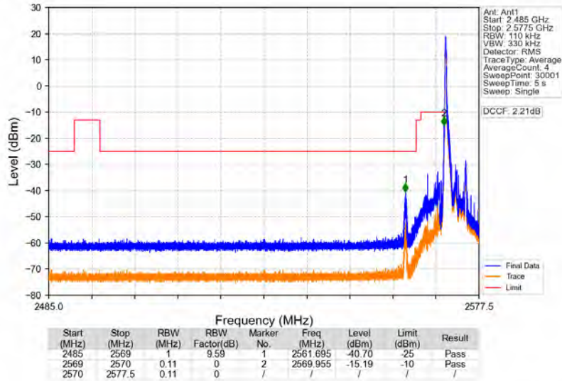
Band38_5MHz_64QAM_LCH_2572.5MHz_RB_1_0_NTV
