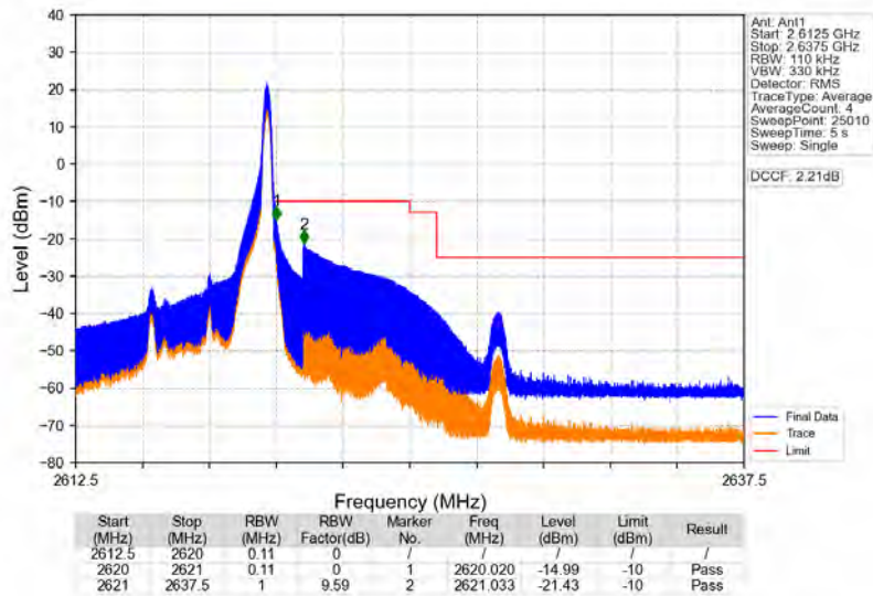
Band38_5MHz_16QAM_HCH_2617.5MHz_RB_1_24_NTNV
