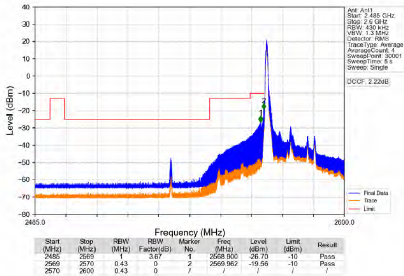
Band38_20MHz_64QAM_LCH_2580MHz_RB_1_0_NTNV
