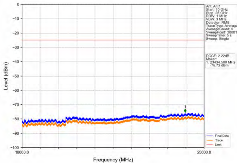
Band38_20MHz_64QAM_HCH_2610MHz_RB_1_0_NTV
