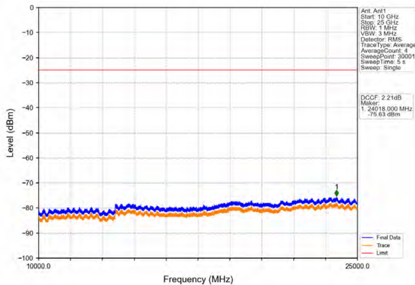
Band38_10MHz_64QAM_HCH_2615MHz_RB_1_0_NTV
