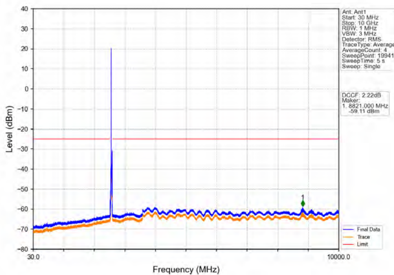
Band38_20MHz_64QAM_LCH_2580MHz_RB_1_0_NTNV
