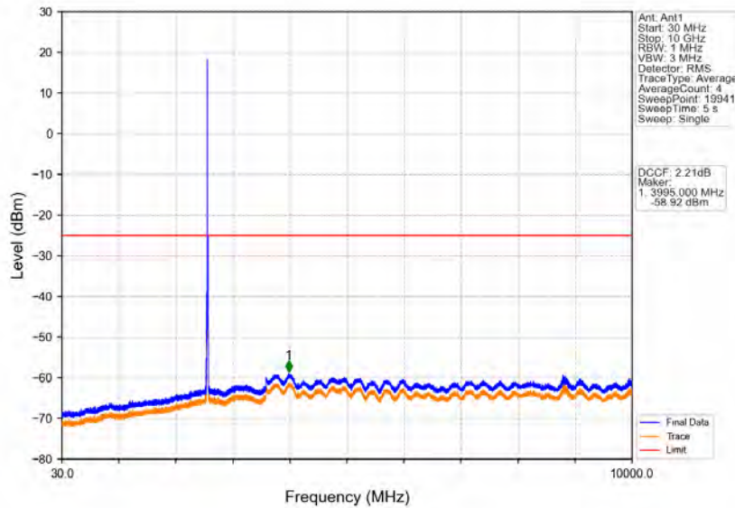
Band38_10MHz_16QAM_LCH_2575MHz_RB_1_0_NTV
