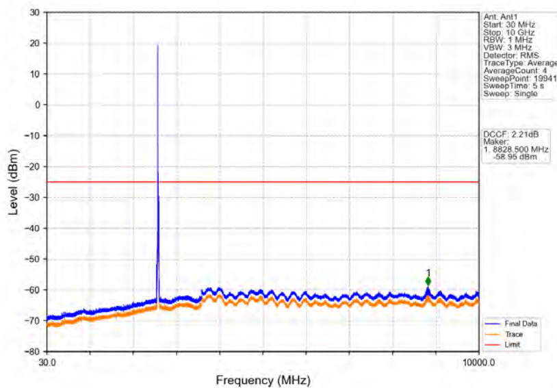
Band38_15MHz_64QAM_MCH_2595MHz_RB_1_0_NTNV
