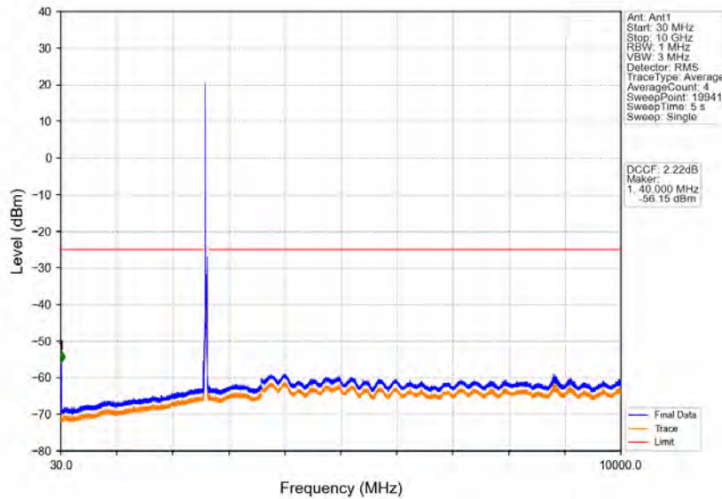
Band38_20MHz_64QAM_HCH_2610MHz_RB_1_0_NTV
