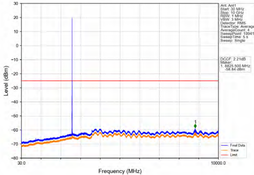
Band38_5MHz_16QAM_MCH_2595MHz_RB_1_0_NTNV
