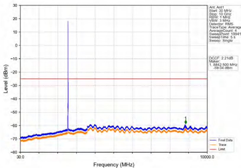
Band38_10MHz_64QAM_LCH_2575MHz_RB_1_0_NTNV
