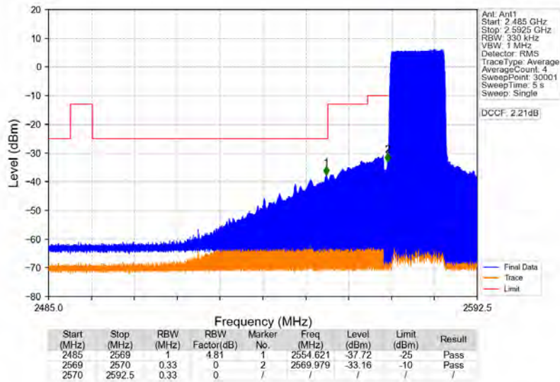
Band38_15MHz_64QAM_LCH_2577.5MHz_RB_75_0_NTNV
