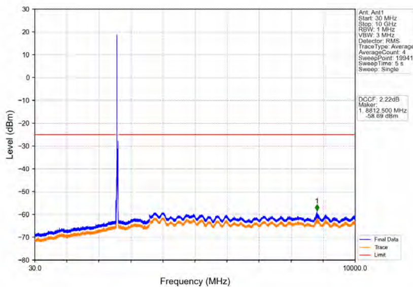
Band38_20MHz_64QAM_MCH_2595MHz_RB_1_0_NTNV
