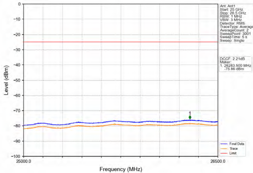
Band38_10MHz_16QAM_LCH_2575MHz_RB_50_0_NTNV
