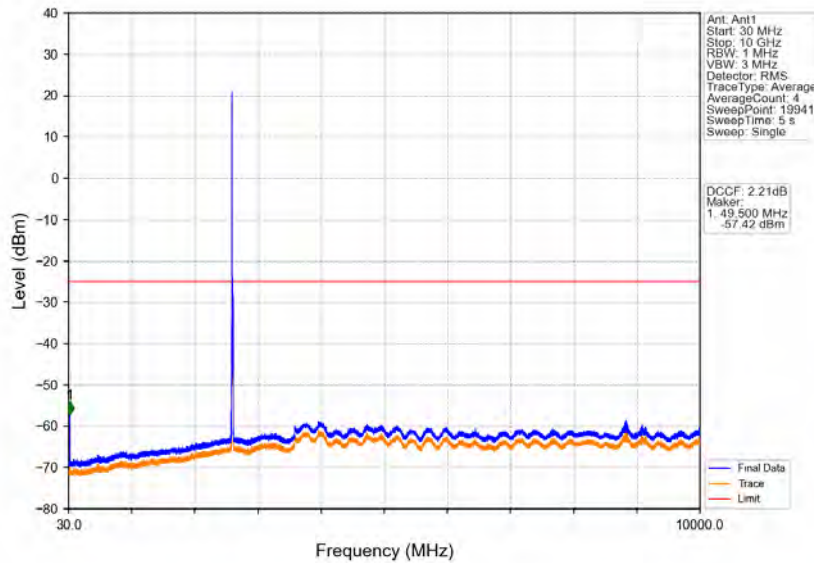
Band38_10MHz_64QAM_HCH_2615MHz_RB_1_0_NTV
