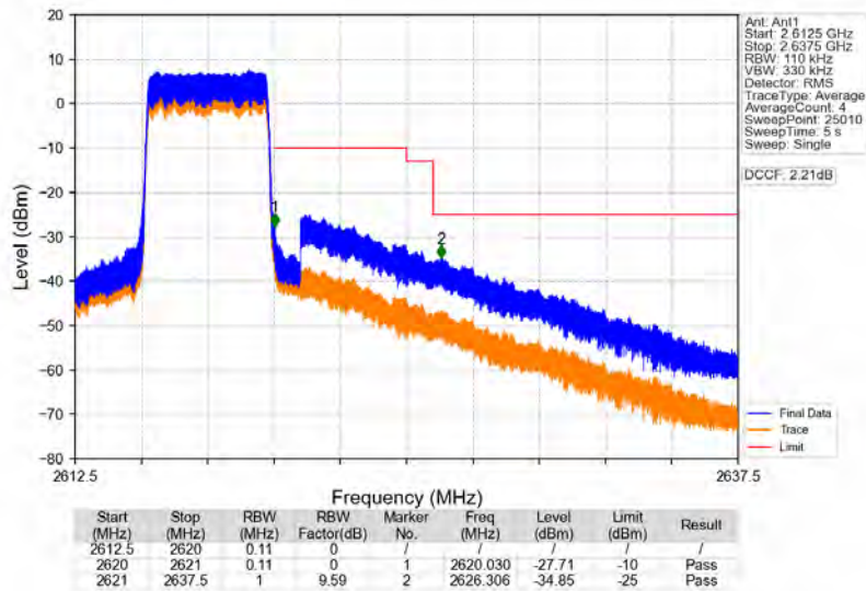
Band38_5MHz_16QAM_HCH_2617.5MHz_RB_25_0_NTNV
