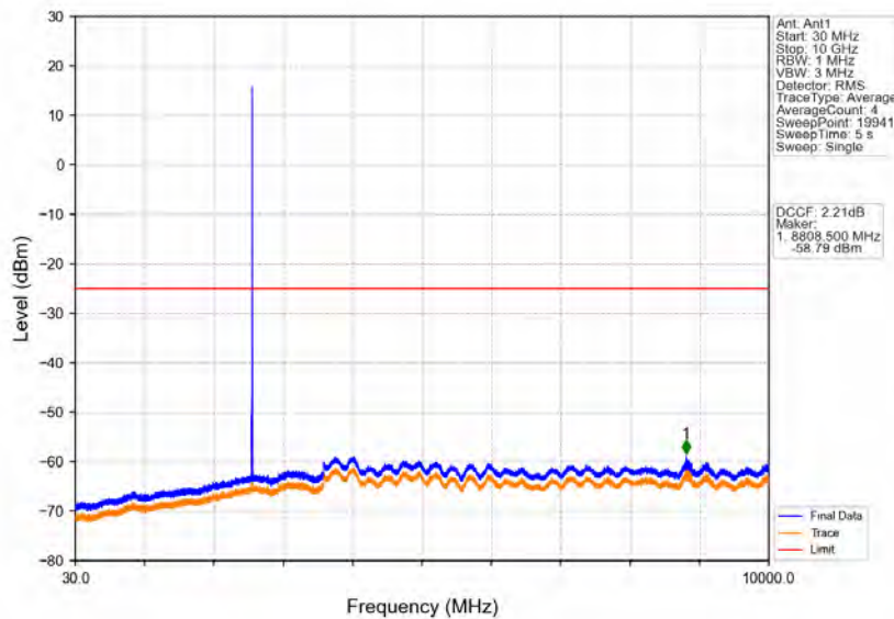
Band38_5MHz_64QAM_LCH_2572.5MHz_RB_1_0_NTV
