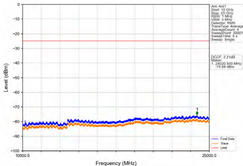
Band38_10MHz_16QAM_LCH_2575MHz_RB_1_0_NTV
