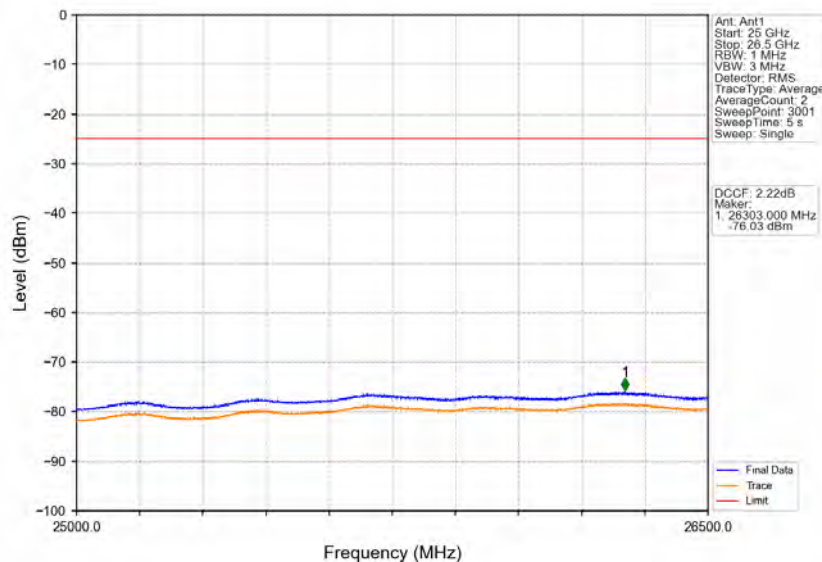
Band38_20MHz_64QAM_LCH_2580MHz_RB_1_0_NTV
