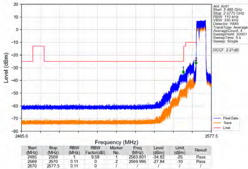
Band38_5MHz_QPSK_LCH_2572.5MHz_RB_25_0_NTNV
