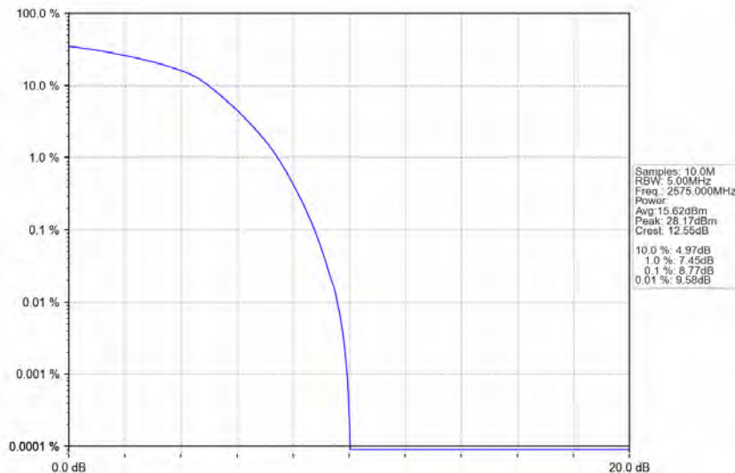
Band38_10MHz_16QAM_LCH_2575MHz_RB_50_0_NTNV
