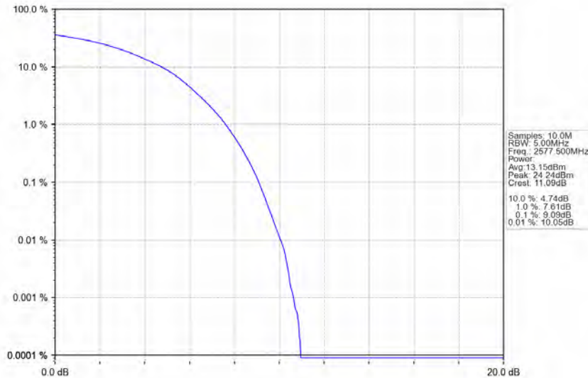
Band38_15MHz_64QAM_LCH_2577.5MHz_RB_75_0_NTNV
