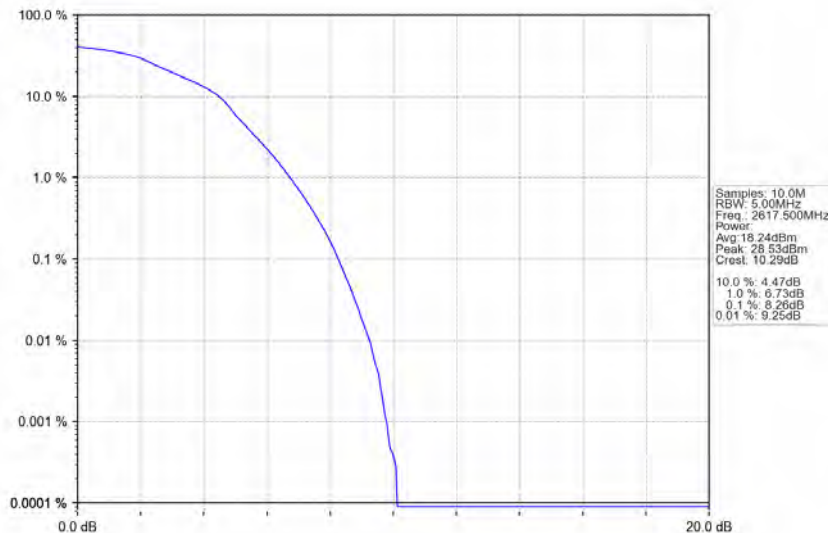
Band38_5MHz_16QAM_HCH_2617.5MHz_RB_25_0_NTNV
