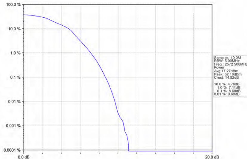
Band38_5MHz_16QAM_LCH_2572.5MHz_RB_25_0_NTNV
