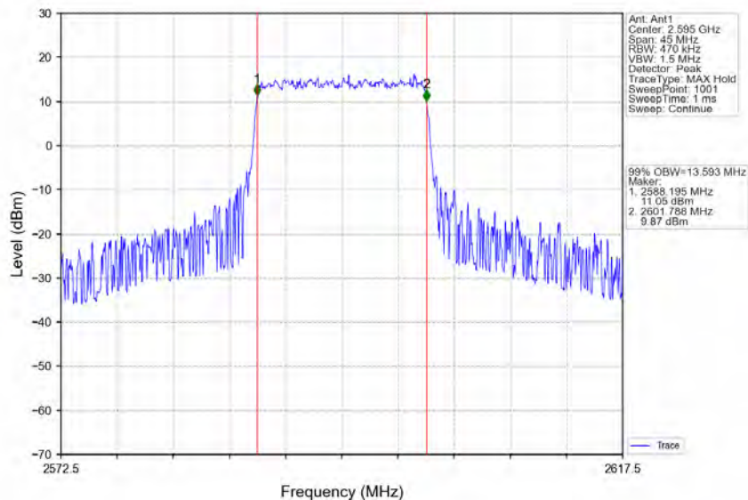
Band38_15MHz_64QAM_MCH_2595MHz_RB_75_0_NTNV
