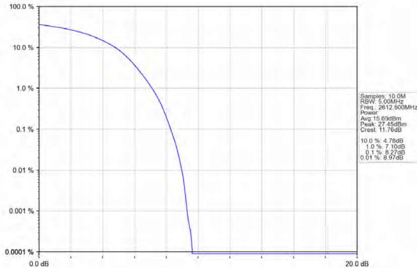
Band38_15MHz_QPSK_HCH_2612.5MHz_RB_75_0_NTNV
