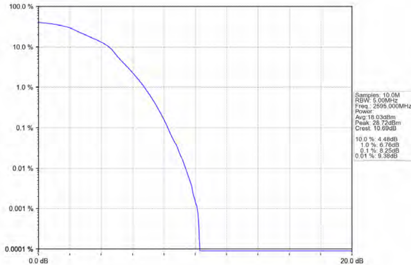
Band38_5MHz_16QAM_MCH_2595MHz_RB_25_0_NTNV
