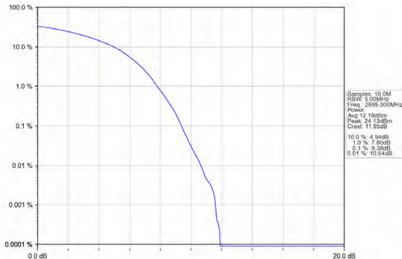
Band38_20MHz_64QAM_MCH_2595MHz_RB_100_0_NTNV
