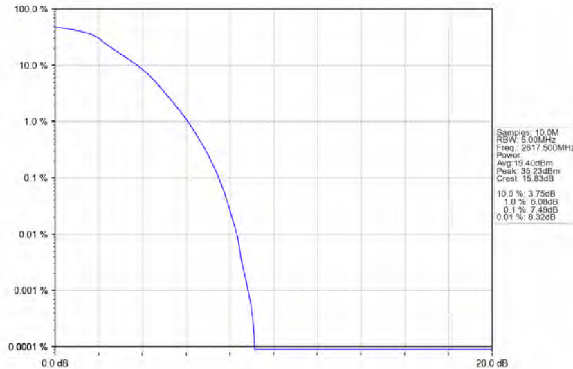
Band38_5MHz_QPSK_HCH_2617.5MHz_RB_25_0_NTNV
