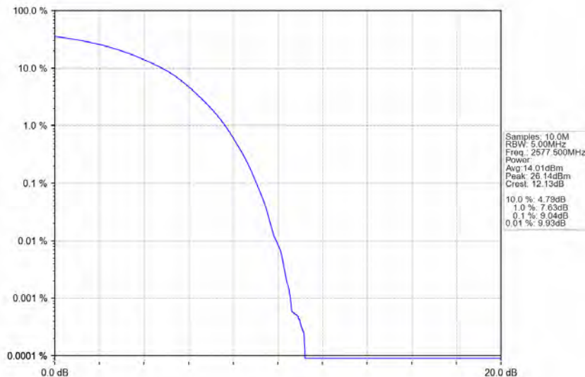
Band38_15MHz_16QAM_LCH_2577.5MHz_RB_75_0_NTNV
